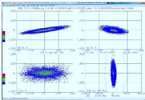
Figure 3: Particle distribution of muons at the RFQ II exit.
