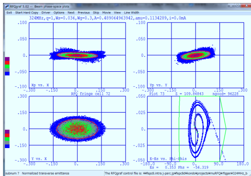
Figure 8: Phase plots of extracted particles from muRFQ.
