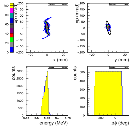
Figure 1: UCM distribution at the RFQ II entrance. The ellipses in upper figures represent the matched ellipses of \epsilon_{t,n,rms} = 0.167\pi \text{ mm mrad} .
