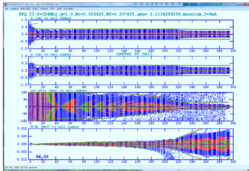
Figure 2: PARMTEQM simulation result of UCM acceleration.
