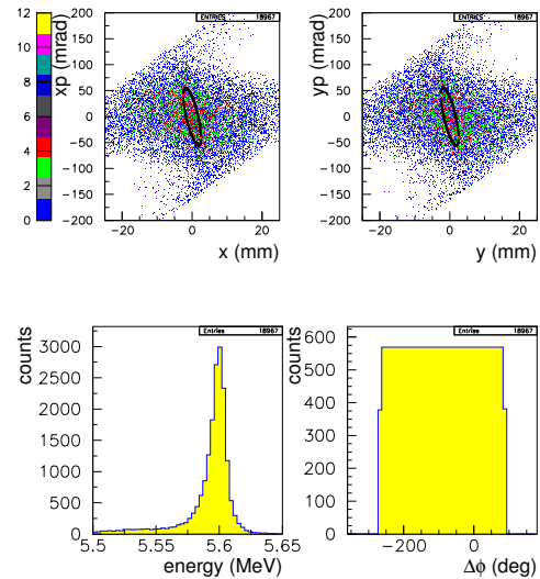
Figure 4: Input distribution of the Mu - simulation.
