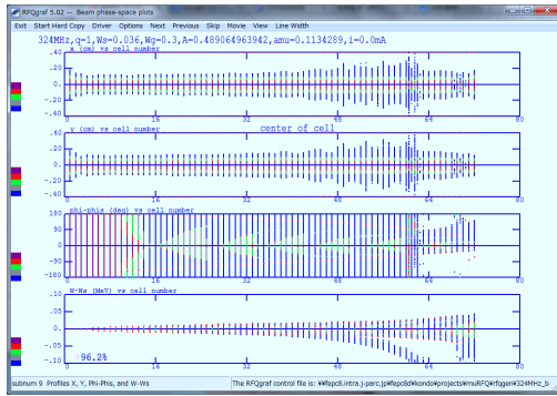
Figure 7: Evolution of the distribution in muRFQ.
