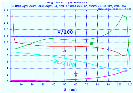
Figure 6: Designed cell parameters of the muRFQ using RFQGEN.
