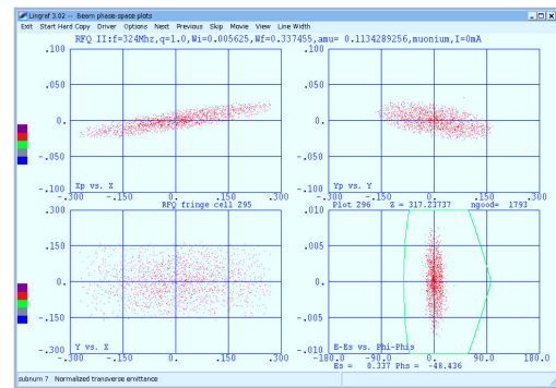
Figure 5: Phase plots of Mu - at the RFQ exit.
