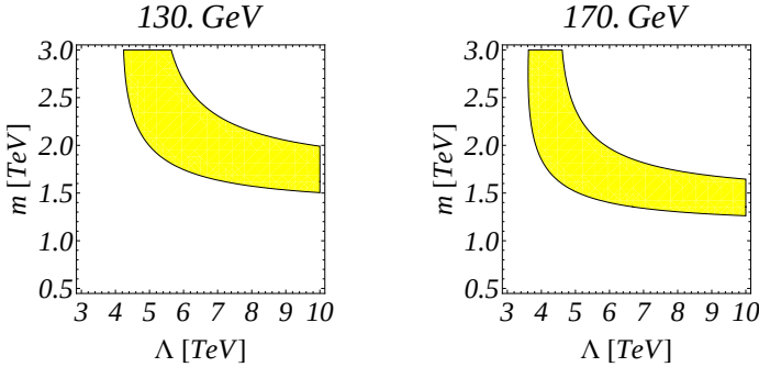
Fig. 2. The allowed region in the (m, \Lambda) plane for D_t = 0 , N_\varphi = 6 and \sum_{i=1}^{N_\varphi} \Omega_\varphi^{(i)} h^2 = 0.106 \pm 0.008 at the 3\sigma level for m_h = 130 GeV and 170 GeV (as indicated above each panel).
