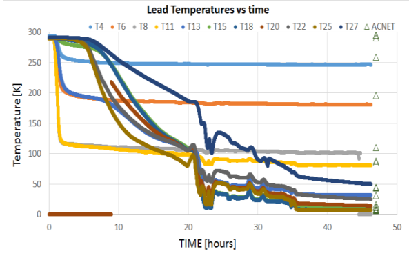
Fig. 13. Leads cooling down.
