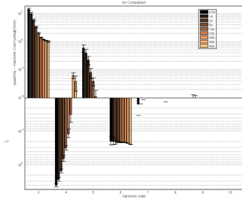
Fig. 7. Quadrupole normal integrated field harmonics.
