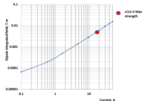
Fig. 6. Dipole corrector integrated field.
