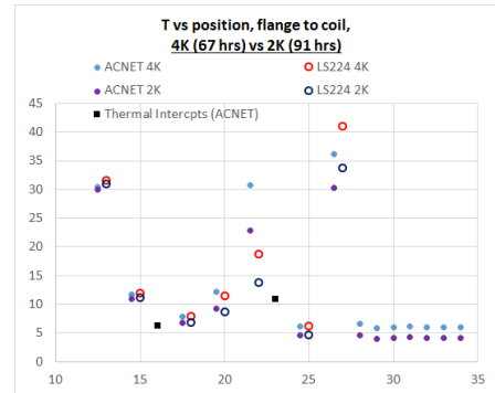
Fig. 15. The temperature distribution along the cold part of leads.
