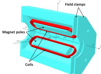
Fig. 3. One half of magnet package view.
