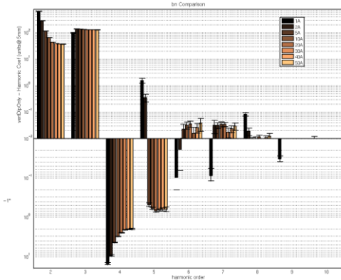
Fig. 8. Dipole integrated normal field harmonics.
