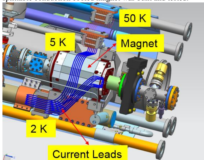
Fig. 1. Magnet package inside the SCRF Cryomodule.
