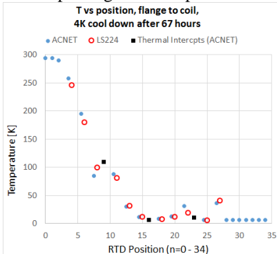
Fig. 14. Temperature profile along leads from 300 K to 4 K after 67 hours.
