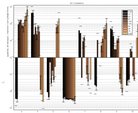
Fig. 9. Quadrupole integrated normal geometric field harmonics.
