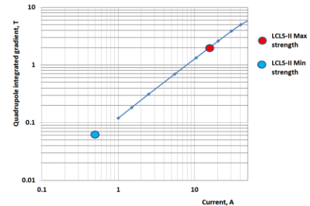
Fig. 5. Quadrupole magnet integrated gradient.
