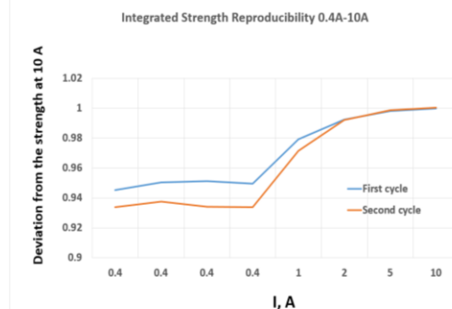
Fig. 10. Quadrupole strength reproducibility for multiple ramps.
