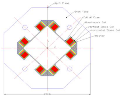
Fig. 2. The magnet package cross-section.
