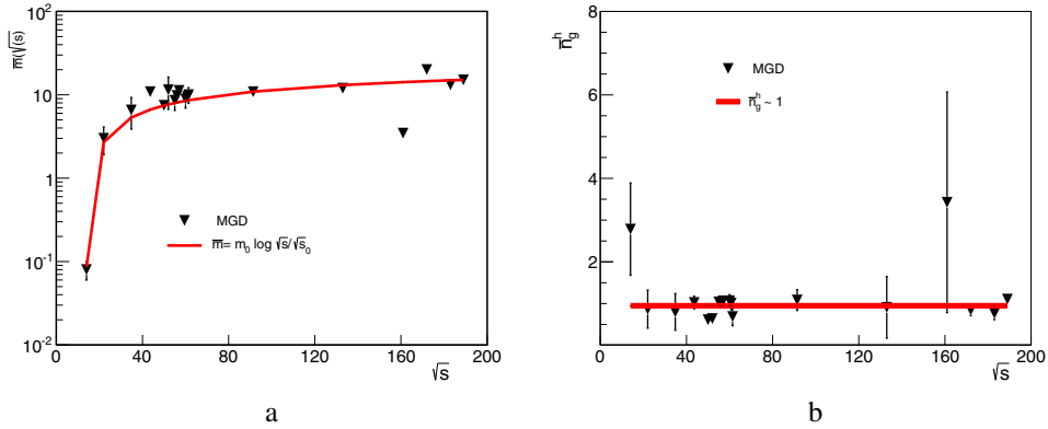
Figure 1. (a) The parameter \bar{m}_g , average multiplicity of gluons formed in the qg -cascade from a single gluon. (b) The hadronization parameter \bar{n}_g^h ([4]) means the average multiplicity of hadrons formed from single gluon. The number of hadrons formed from one gluon during its passing of the second stage. Experimental data for the MD description of hadrons by GDM was taken from about 10 GeV up to 200 GeV [5]
