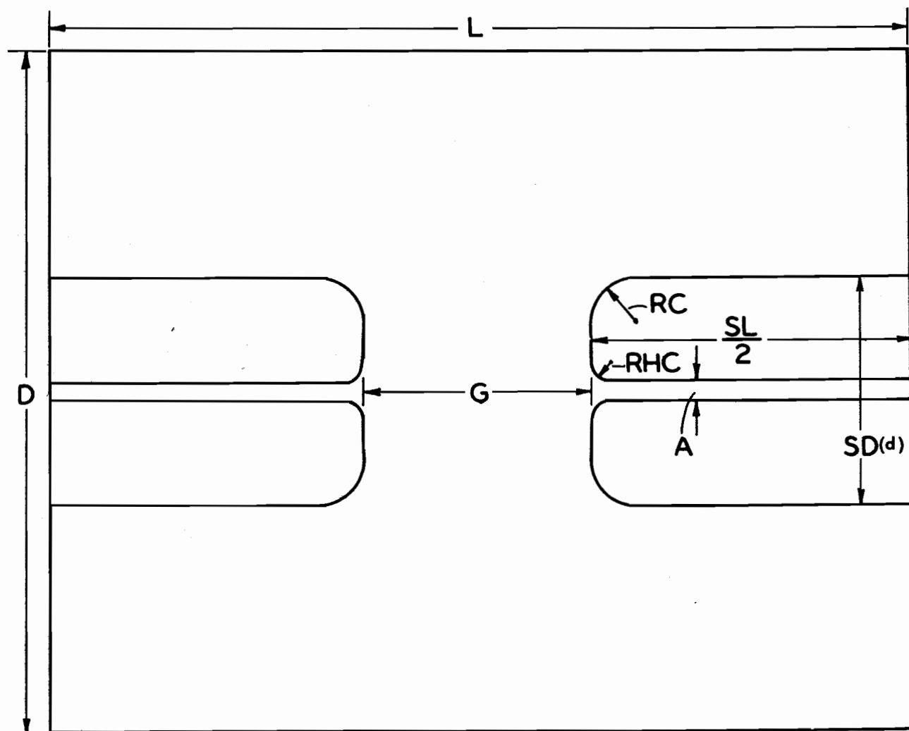
Fig. 1 Unit Cell Geometry (Cylindrical Drift Tube)
