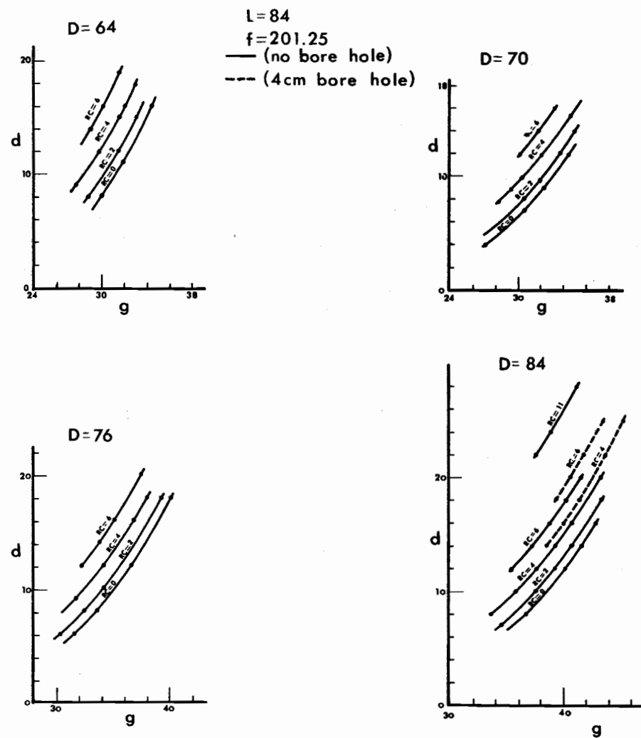
Fig.7 Resonance Cures For Cylindrical Drift Tubes At 200 MeV
