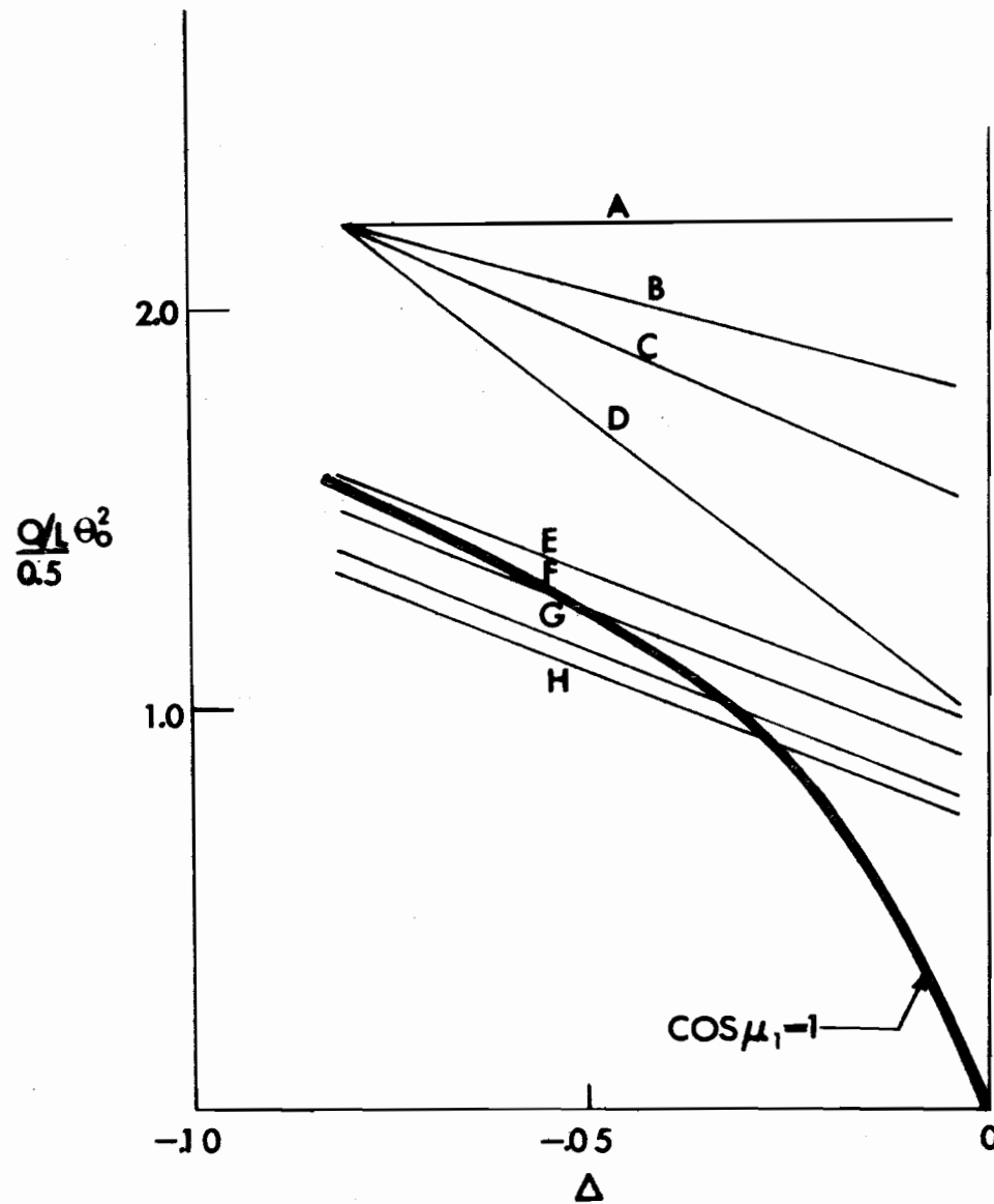
STABILITY DIAGRAM
