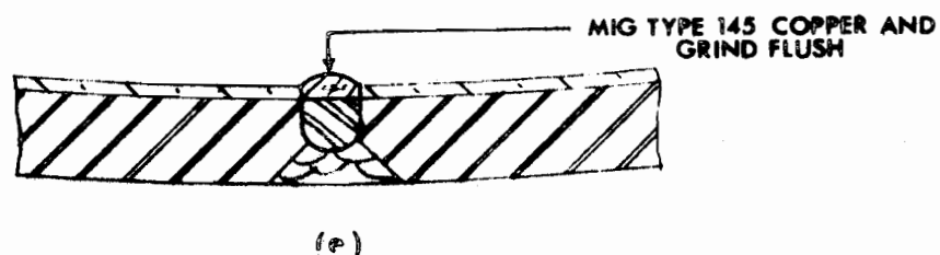
COPPER CLAD CAVITY WELDING SEQUENCE
