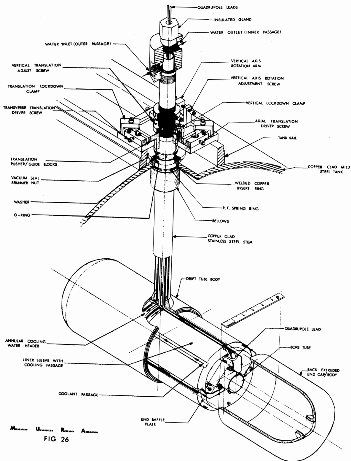
DRIFT TUBE ISOMETRIC
