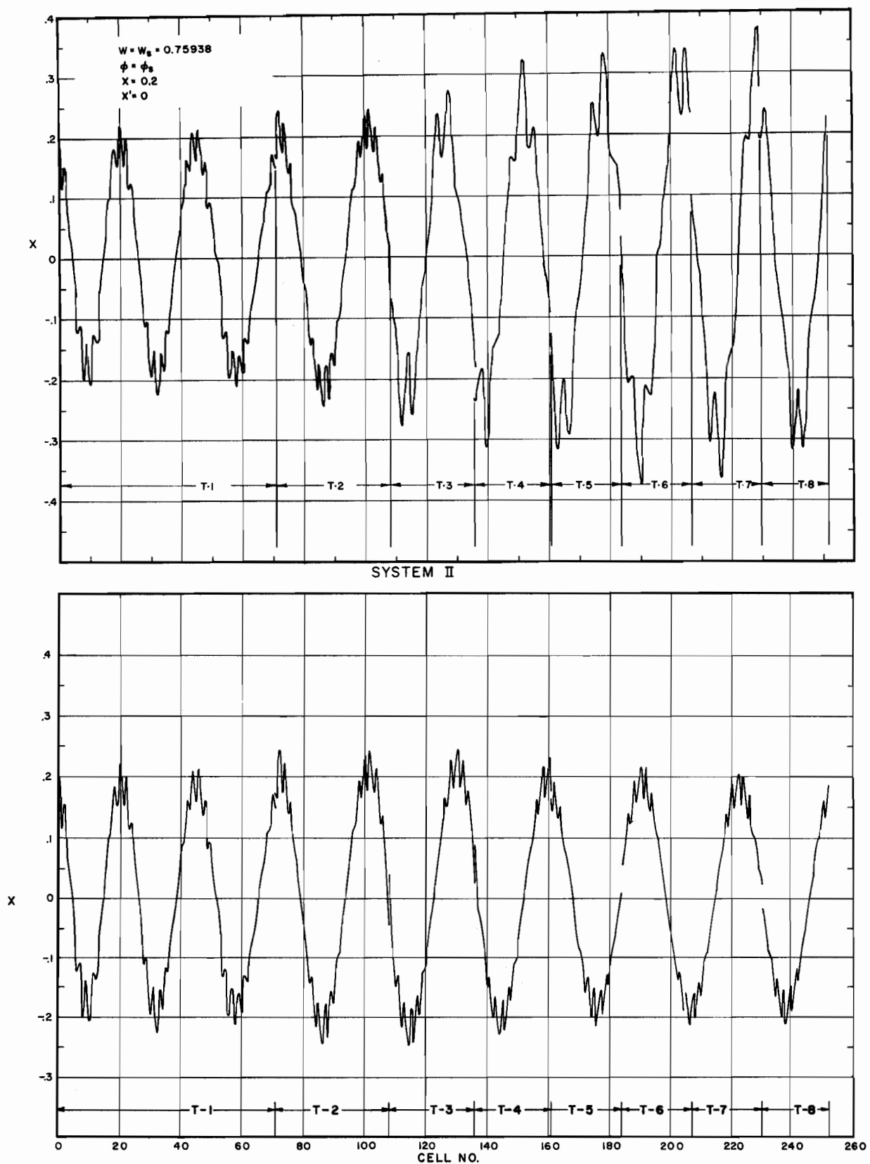
Fig. 20 TRANSVERSE MOTION (QUADRUPOLE SYSTEM I)
