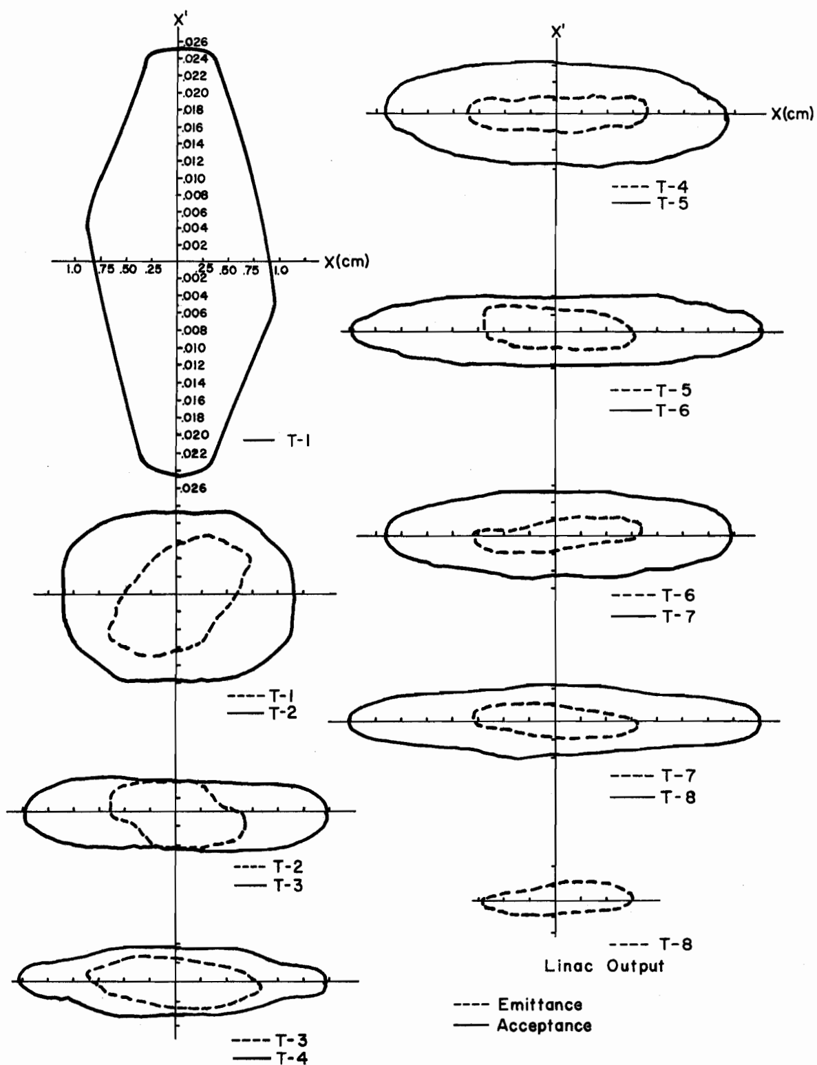
FIG.15 X, X' ACCEPTANCE-EMITTANCE PLOTS FOR EACH CAVITY
