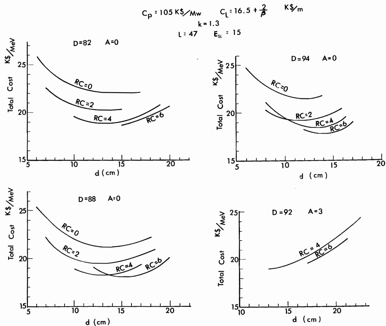
FIG. 8 COST CURVES AT 50 MeV
