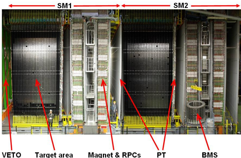
Fig. 2. View of the OPERA detector. The neutrino beam enters from the left. Arrows show the position of the VETO planes, the target and TT, the drift tubes (PT), the magnets and the resistive plates chambers (RPC) installed between the magnet iron slabs.
