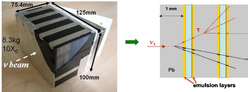
Fig. 1. ECC Brick: form (left) and scheme of the internal structure with one typical \nu_\tau detection topology (right).
