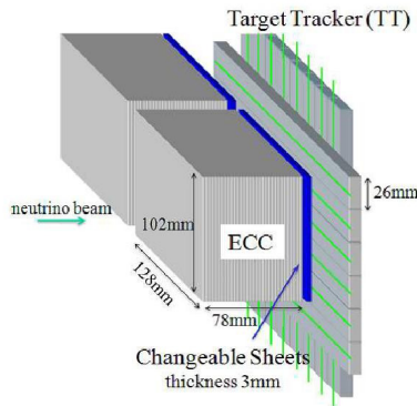
Fig. 4. Schematic view of the bricks with their CS attached in front of TT planes.
