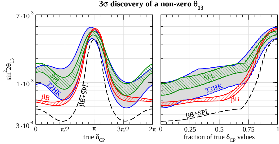
Fig. 10. 3\sigma discovery sensitivity to \sin^2 2\theta_{13} for \beta B , SPL, and T2HK as a function of the true value of \delta_{CP} (left panel) and as a function of the fraction of all possible values of \delta_{CP} (right panel). The width of the bands corresponds to values for the systematical errors between 2% and 5%. The dashed curves correspond to the combination of \beta B and SPL with 10 yrs of total data taking each for a systematical error of 2%.
