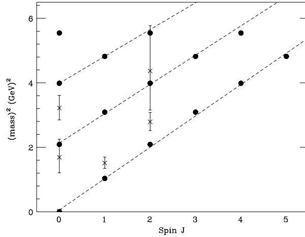
Fig. 4. The meson masses square, M^2 , in the pion channel are plotted as a function of their spins, J . The experimental masses are shown by the crosses with experimental widths of the corresponding states and the theoretical ones by the black dots connected by dashed straight lines.
