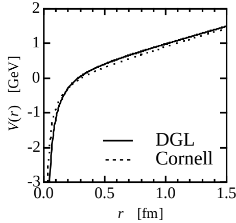
Fig. 1. The static potential between a quark and antiquark pair calculated within the DGL theory to compare with the phenomenological potential of Cornell group. Taken from Suganuma et al. . [15]
