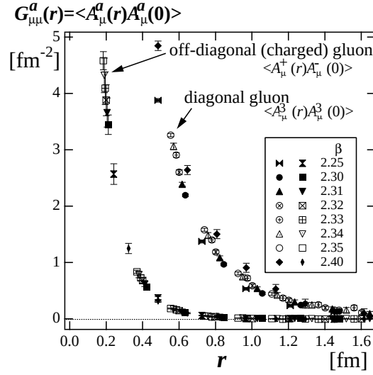
Fig. 3. The gluon correlation, \langle A_\mu^a(r)A_\mu^a(0) \rangle , on the lattice for the diagonal gluon and the charged gluon for the SU(2) gauge as a function of the four dimensional distance, r . Taken from Amemiya and Suganuma [19].
