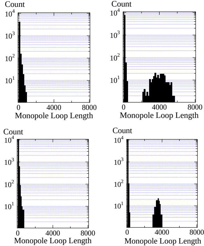
Fig. 5. The monopole length distribution. The upper two figures are the results of the multi-instanton gas with small density (left) and with large density (right). The lower two figures correspond to the case of pure SU(2) gauge theory on 163 \times 4 at high temperature (left) and at low temperature (right), which correspond to the confined phase. Taken from Fukushima et al. [21]
