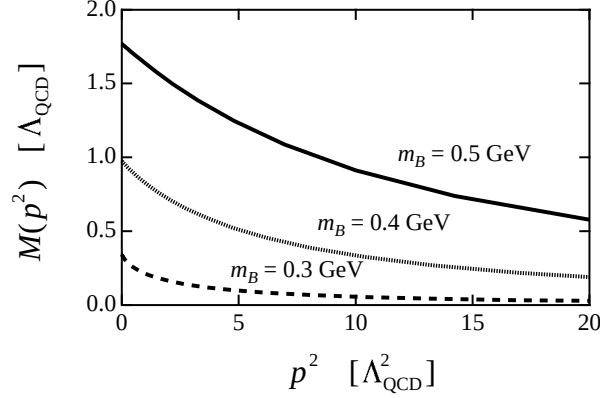
Fig. 2. The constituent quark mass calculated within the DGL theory with various values of the dual gluon mass, which indicates the strength of monopole condensation, as a function of the Euclidean momentum square. The unit \lambda_{\text{QCD}} is 200MeV. Taken from Suganuma et al. [15]
