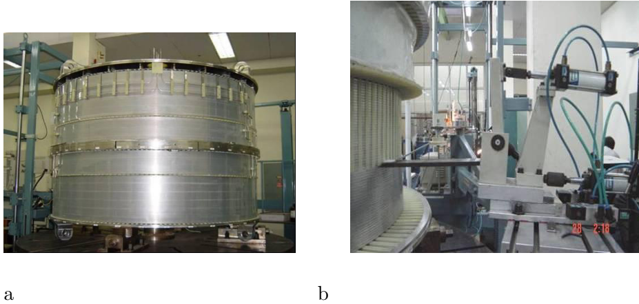
Figure 19. (a) The superconducting magnet. (b) Wrapping wire around the magnet.
