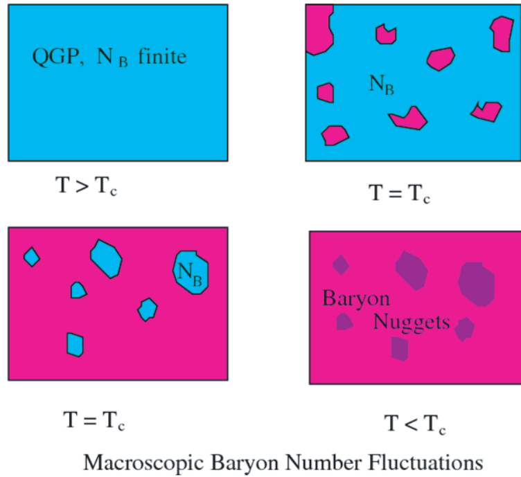
Figure 12. A hypothetical QGP phase transition in the early universe.
