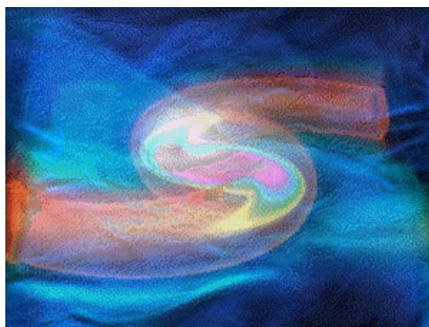
Figure 15. The a pictorial representation of the evolution of the collision of neutron stars.
