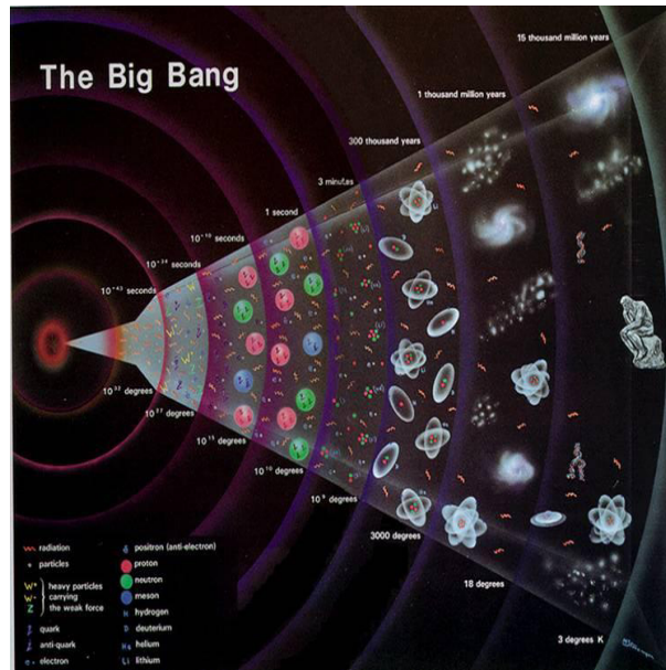
Figure 11. A pictorial history of the big bang.
