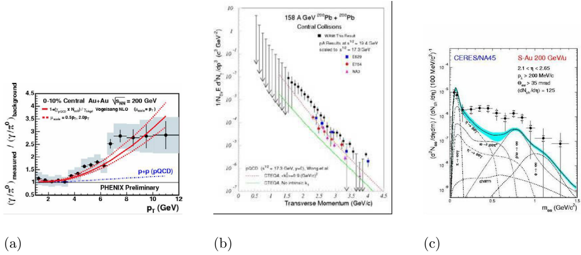
Figure 7. a Hard photons measured at RHIC b Soft photons measured at CERN c Soft dileptons measured at CERN .
