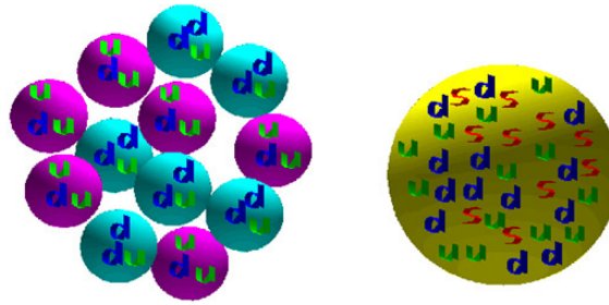
Figure 13. Nuclear matter and strange quark matter.
