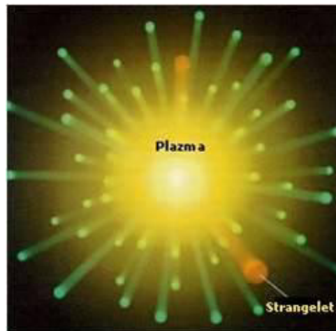
Figure 14. The primeval QGP making strangelets.
