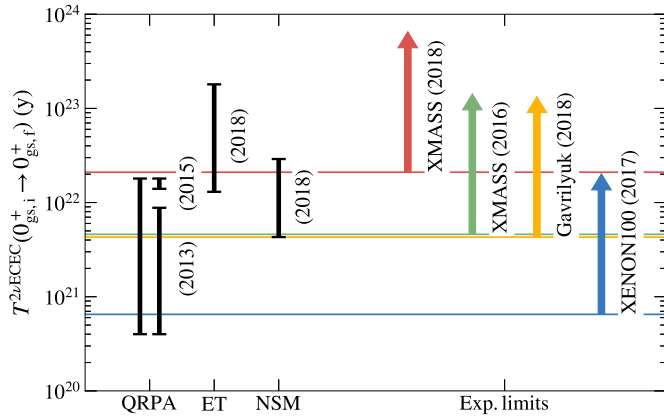
Fig. 2. ^{124}\text{Xe} half-life for the 2\nu\text{EEEC} of two K-shell electrons. The black bars show the theoretical predictions from the effective theory (ET) and the nuclear shell model (NSM), as well as most recent QRPA calculations [39,40], in comparison to the horizontal lines that indicate the experimental lower limits set by the XENON100 [34] (blue) and XMASS [33,35] (green, red) collaborations as well as Gavriluk et al. [32] (yellow).
