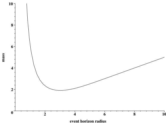
Fig. 1. The mass, \frac{M}{\sqrt{\theta}} , versus the event horizon radius, \frac{r_H}{\sqrt{\theta}} . As can be seen from the figure, the existence of a minimal non-zero mass is clear, i.e. M_0 \approx 1.9\sqrt{\theta} .
