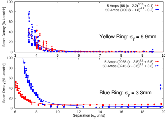
Figure 2: Beam loss rate as a function of vertical distance, in Yellow and Blue ring for experiment 2. The solid lines are power law fits to the respective data.
