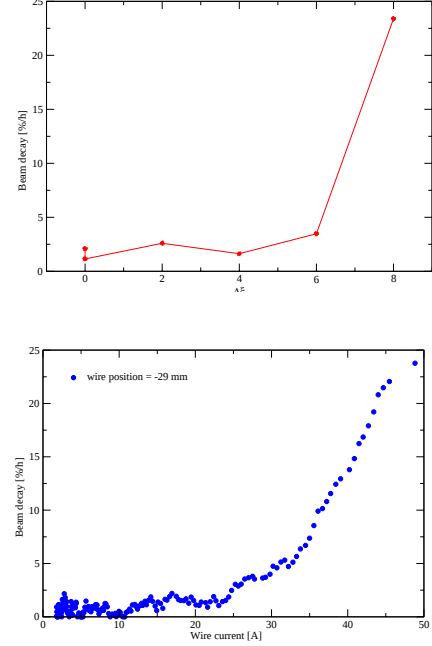
Figure 4: Yellow beam loss rate as a function of vertical chromaticity change (top) with the wire at fixed position -29 mm, and Yellow beam loss rate as a function of wire current at the maximum chromaticity setting (bottom). For the data in the latter plot the wire current was gradually turned off.
