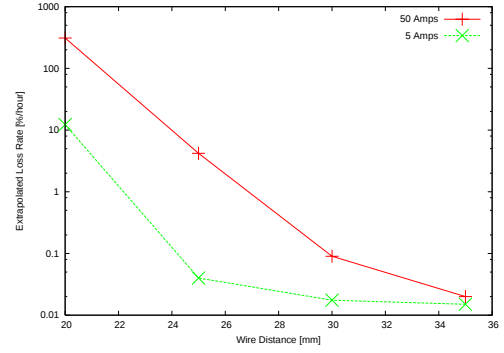
Figure 8: Loss rate as a function of wire distance for 5 A and 50 A wire current, calculated with PLIBB, for the Blue beam in experiment 2 [8].
