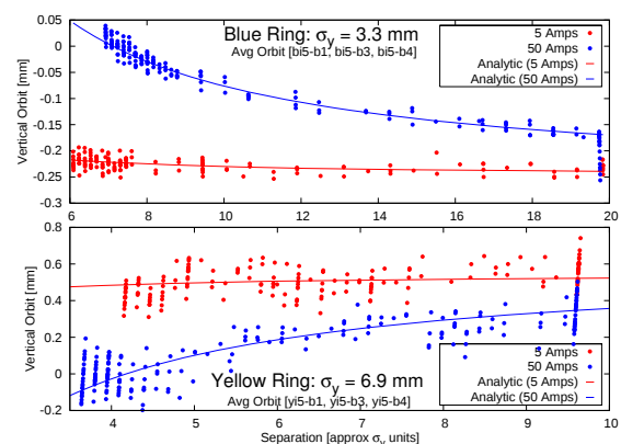
Figure 1: Vertical orbit change (average of 3 BPMs near wire) as a function of vertical distance, in Blue and Yellow ring for experiment 2 (May 9, 2007).
