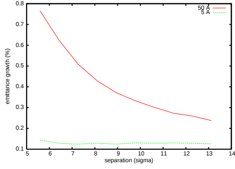
Figure 5: Blue emittance growth in percent over 10^5 turns for 5 A and 50 A wire current.
