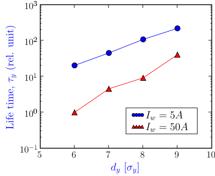
Figure 6: Vertical escape time \tau_y , calculated from the diffusion coefficient D_{y,s} as a function of separation for 5 A and 50 A wire current, and normalized by the lifetime \tau_y for 6\sigma separation and 50 A current.
