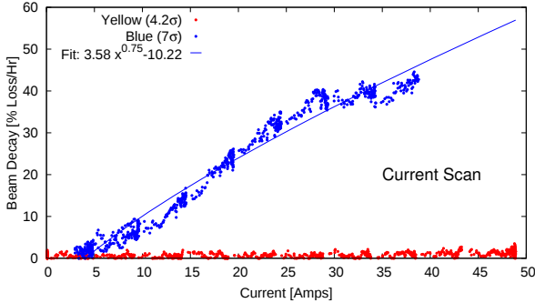
Figure 3: Blue and Yellow beam loss rates as a function of wire current during experiment 2. The Blue wire is fixed at +23 mm, the Yellow wire at -29 mm.
