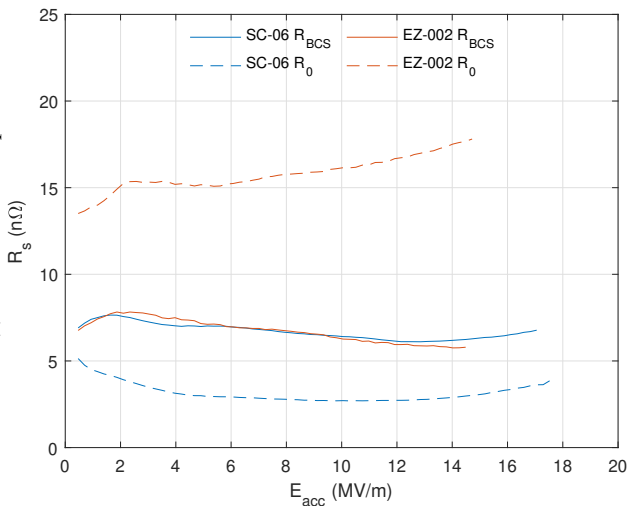
Figure 9: RF test results of the two cavities treated with 2/0 doping. R_{BCS} taken at 2 K. Peak field shown here does not indicate quench field.
