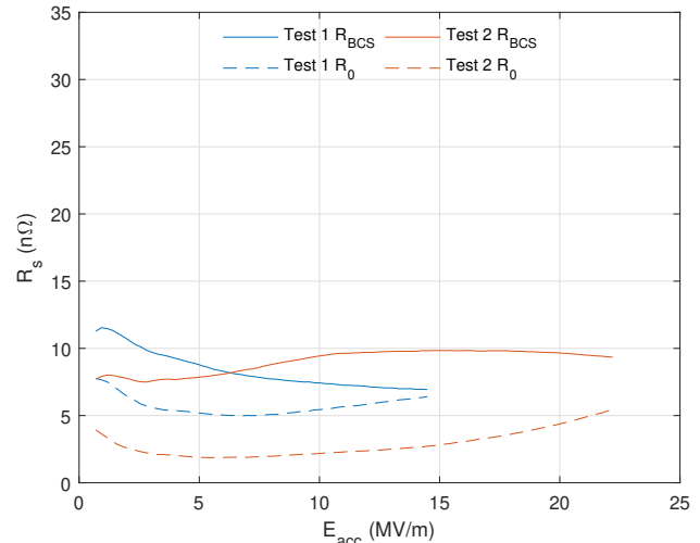
Figure 7: RF test results of the two infusion tests of cavity LTE1-1. R_{BCS} taken at 2 K. Peak field shown here does not indicate quench field.
