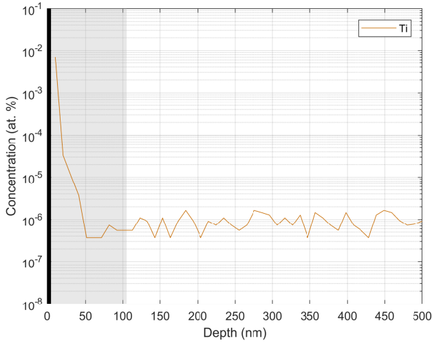
Figure 2: SIMS measurement of atomic concentration of titanium impurities on a witness sample baked alongside SC-06 during the nitrogen infusion run. Black bar indicates surface oxide; gray bar approximates RF penetration layer.
