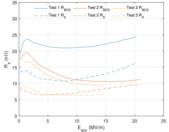
Figure 3: RF test results of the three infusion tests of cavity SC-06. R_{\text{BCS}} taken at 2 K. Peak field shown here does not indicate quench field.
