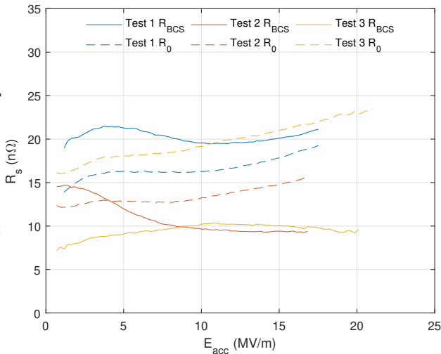
Figure 5: RF test results of the three infusion tests of cavity RDTTD-4. R_{BCS} taken at 2 K. Peak field shown here does not indicate quench field.
