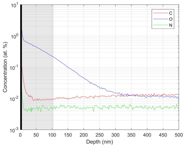
Figure 8: SIMS measurement of atomic concentration of impurities in a witness sample baked with cavity LTE1-1 in its infusion run. Black bar indicates surface oxide; gray bar approximates RF penetration layer.
