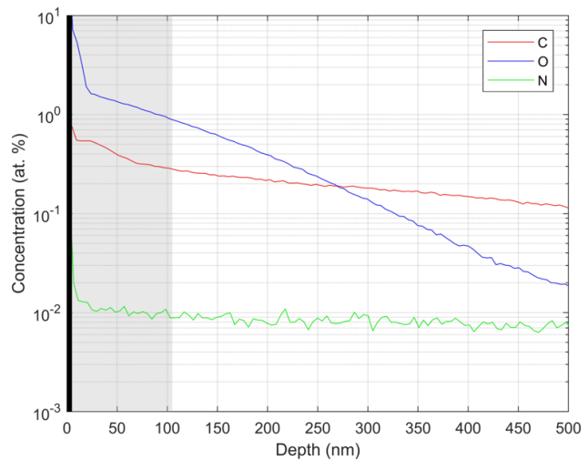
Figure 4: SIMS measurement of atomic concentration of impurities in a witness sample baked with cavity SC-06 in its infusion run. Black bar indicates surface oxide; gray bar approximates RF penetration layer.
