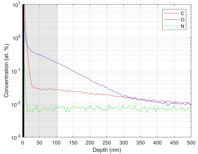
Figure 6: SIMS measurement of atomic concentration of impurities in a witness sample baked with cavity RDTTD-4 in its infusion run. Black bar indicates surface oxide; gray bar approximates RF penetration layer.
