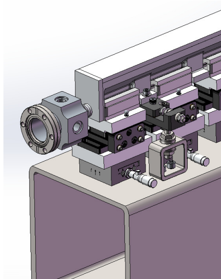
Figure 3: Truncated view of the engineering model of the IOTA insert.
