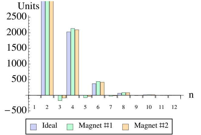
Figure 2: Upright harmonic content of the 1 segments of the IOTA insert prototype, B_n , in units of 10^4 where B_2 \equiv 10^4 (and has been intentionally clipped). Measurement error is less than 2 units. The values have been corrected for feed down.
