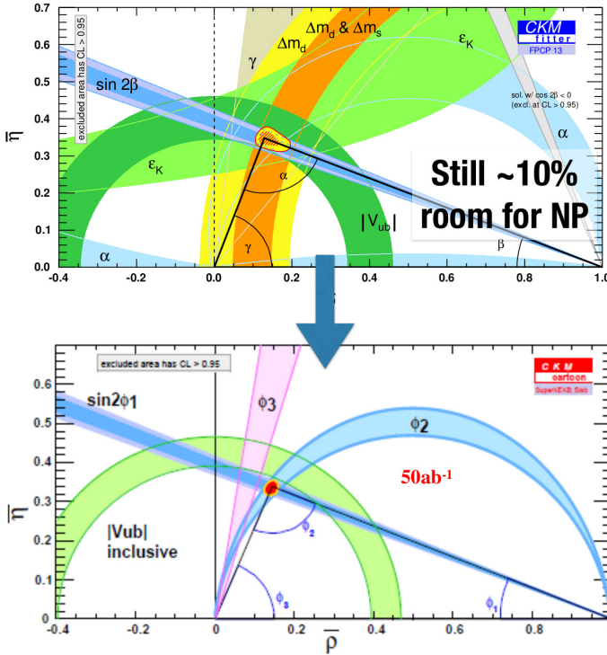
Fig. 2. Projected improvements in the CKM matrix experimental determination [8].
