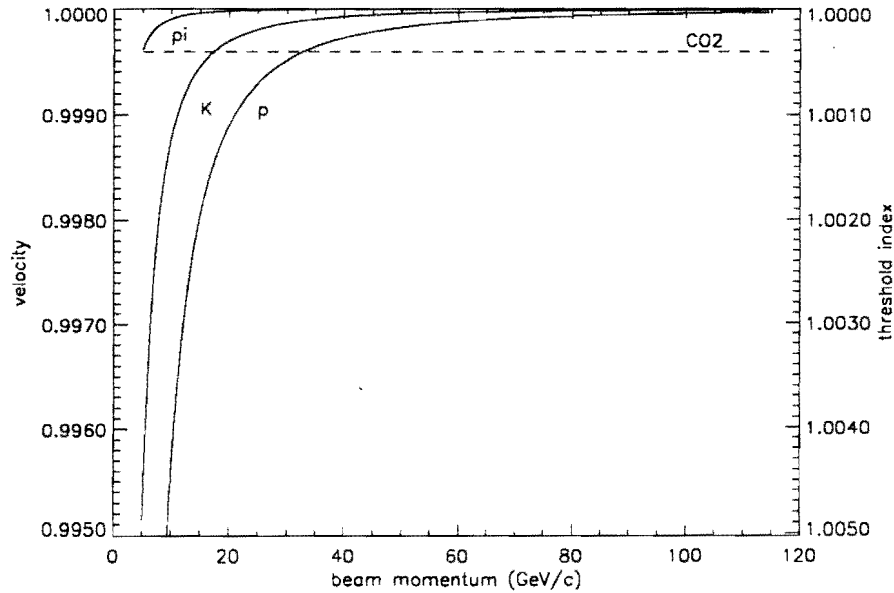
FIG. 10. Particle velocities and threshold indices of refraction as a function of secondary beam momentum.
