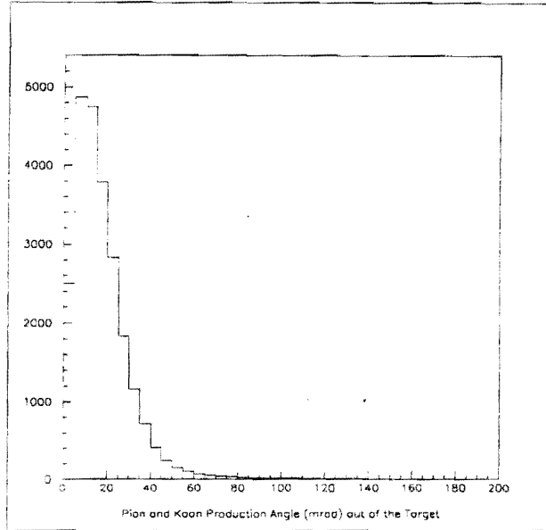
FIG. 3. The hadron production angle out of the target for NuMI.
