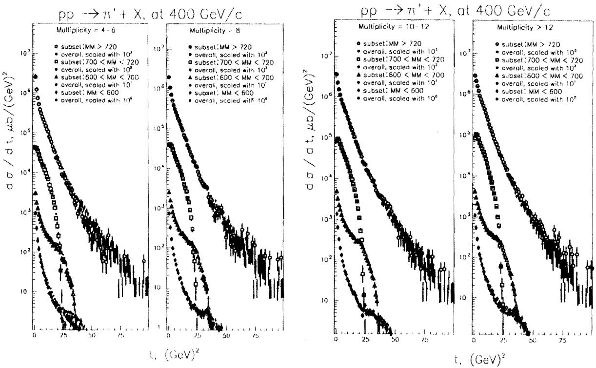
FIG. 2. t distribution for the various subsets in various M^2 ranges. Overall data, weighted by appropriate \beta_{\text{subset}}(M^2) is superimposed on the subset data. Data for each M^2 range is offset from the neighboring one by a factor of 10
