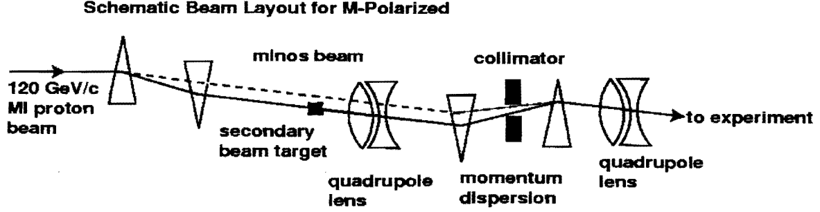
FIG. 6. Schematic of secondary beam-line proposed for M-Polarized.
