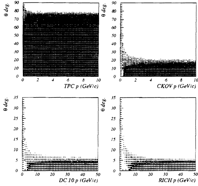
FIG. 12. Acceptance Efficiencies
