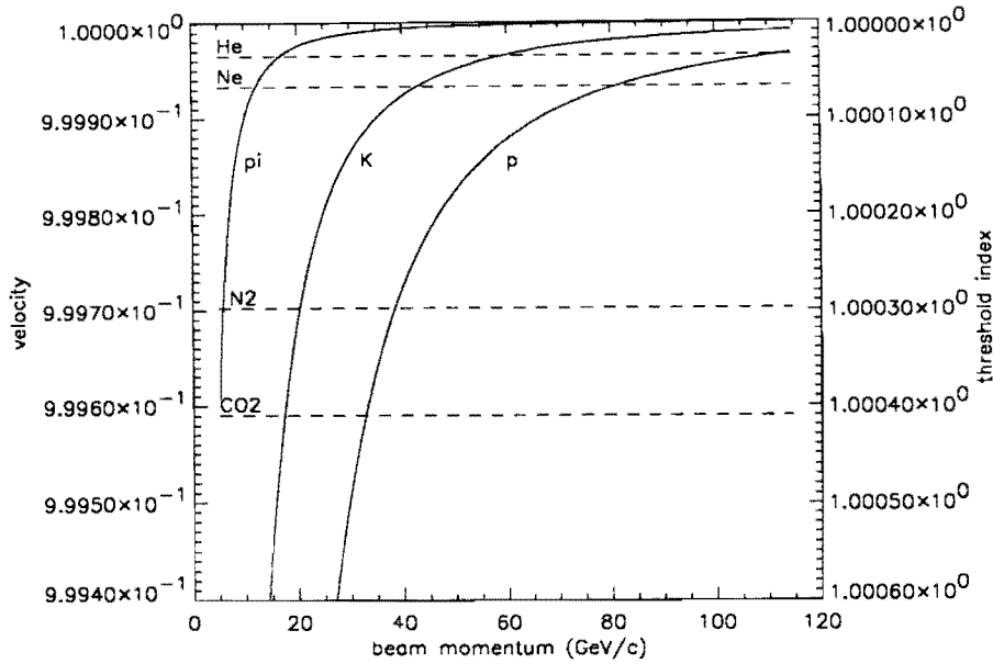
FIG. 11. Particle velocities and threshold indices of refraction as a function of secondary beam momentum.
