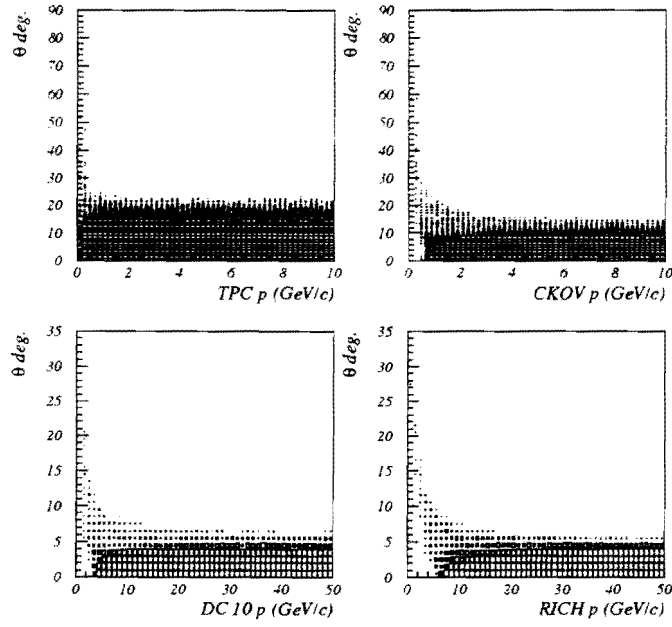
FIG. 13. Acceptance Efficiencies
