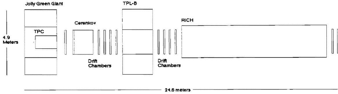
FIG. 5. Experimental layout schematic
