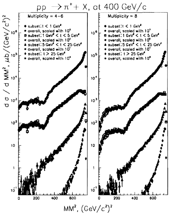
FIG. 1. M^2 distribution for the various subsets in various t ranges. Overall data, weighted by appropriate \beta_{subset}(M^2) is superimposed on the subset data. Data for each t range is offset from the neighboring one by a factor of 10
