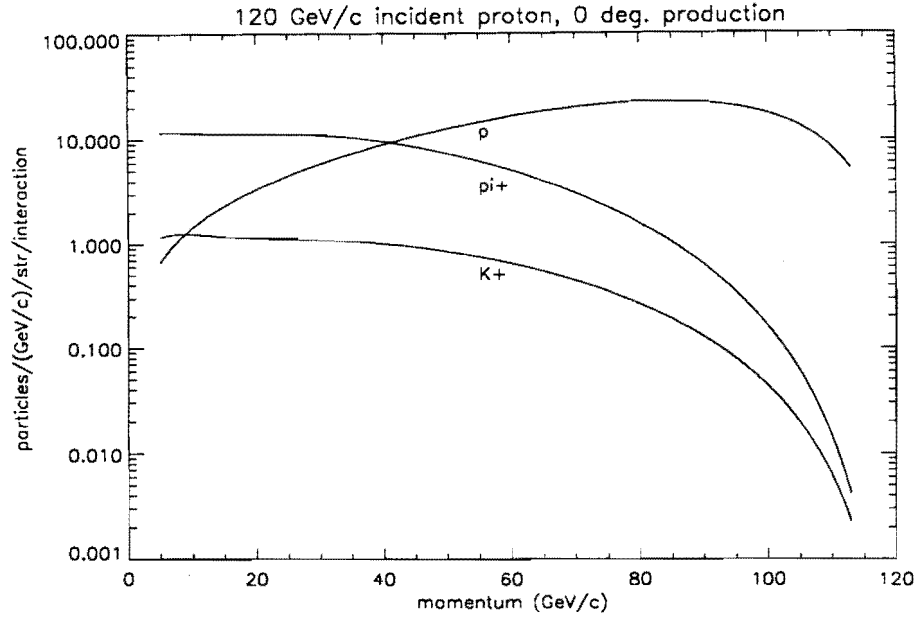
FIG. 8. Positive particle production for 120 GeV/c incident proton beam from [4].
