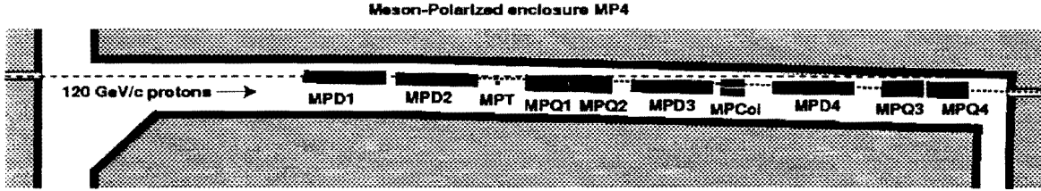
FIG. 7. Layout of proposed M-Polarized beam line in enclosure MP4.
