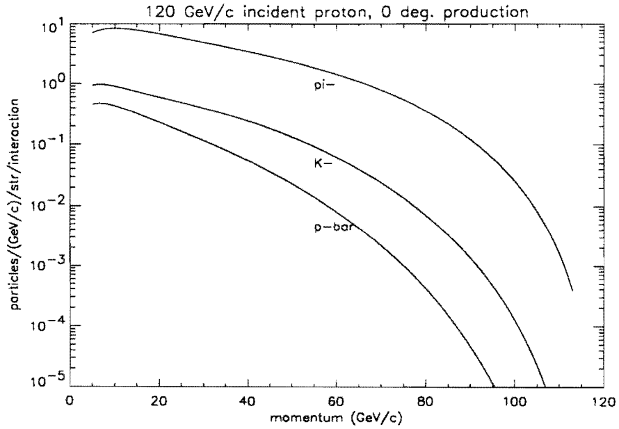
FIG. 9. Negative particle production for 120 GeV/c incident proton beam from [4].
