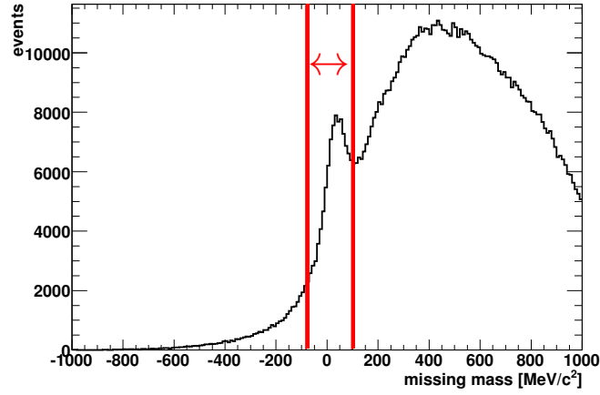
Figure 4.16: Missing mass distribution MM(\gamma N \pi^0 \gamma) for the LH_2 data. The cut limits are indicated by red lines.
