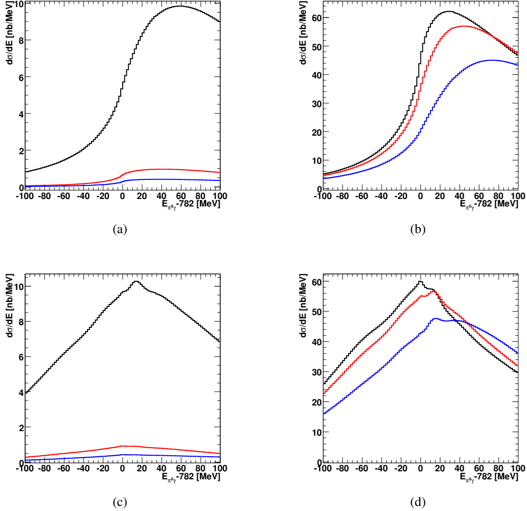
Figure 1.18: (a) and (c): Spectra integrated over angle for three different incoming photon energies: 1.25 GeV (black), 2.0 GeV (red), 3.1 GeV (blue). (b) and (d): Spectra averaged for three different angles: 1° (black), 5° (red), 10° (blue). (a) and (b) are for a zero potential of (V_0, W_0) = (0, 70) MeV (see figure 1.17). (c) and (d) are for a strongly attractive potential (V_0, W_0) = (-156, 70) MeV (see figure 1.16). The cross sections fall off strongly with increasing energy while they decrease with increasing proton angle.
