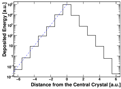
(a) The lateral energy distribution of the shower is approximated by an exponential function.
