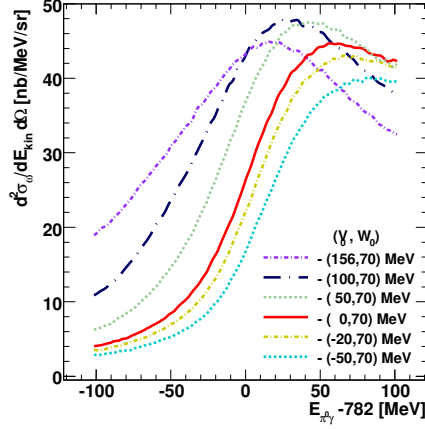
(a) Double differential cross section for \omega -production for different real potential depths and an imaginary potential of W_0(\rho_0) = -70 MeV.
