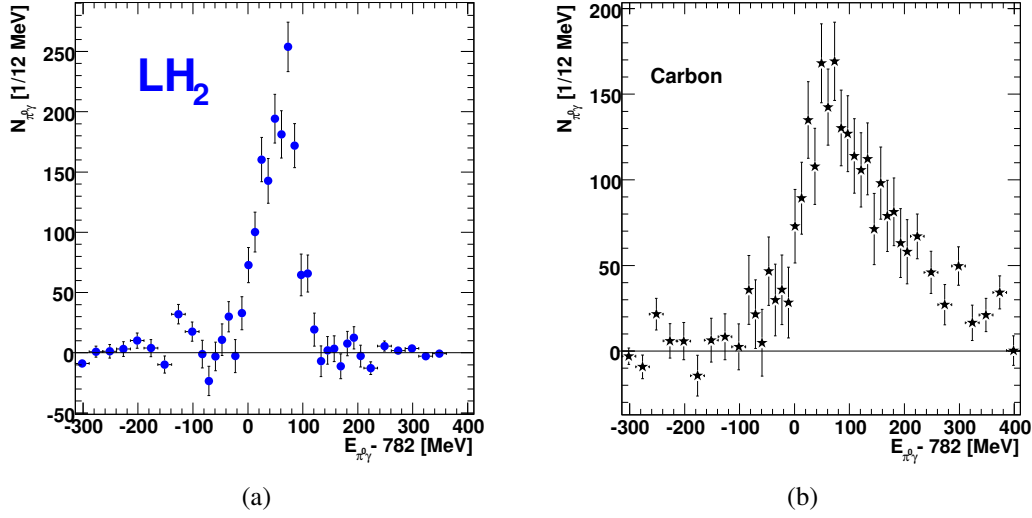
Figure 4.29: E_{\pi^0\gamma} - 782.65 MeV signal spectrum after background subtraction for (a) LH 2 data and (b) carbon data.
