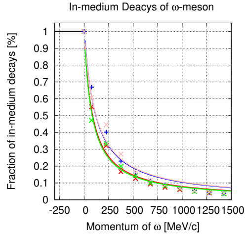
Figure 6.3: In-medium fraction of \omega -meson decays as a function of momentum for calculations on carbon for the incident photon energies of 1250 - 3100 MeV. In red and blue the scenario with collisional broadening only ( \Gamma(\rho_0) = 150 MeV), in green and pink with additional mass shift ( V_0(\rho_0) = -125 MeV) are displayed. Blue and pink show the fraction of in-medium decays ( \rho > 0.1 \rho_0 ), red and green the fraction after reconstruction.
