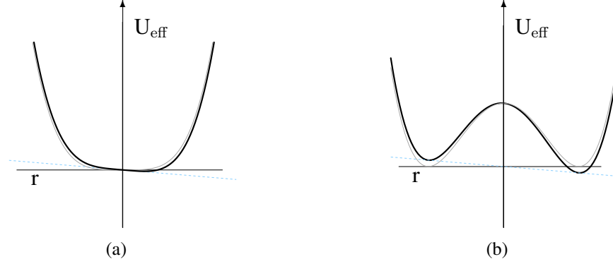
Figure 1.4: Explicit breaking of the chiral symmetry. The thin gray line represents the symmetric Lagrangian. The thin cyan line shows the explicit symmetry breaking term ( -m\bar{\phi}_q\phi_q ), the black line is the full Lagrangian. [4]
