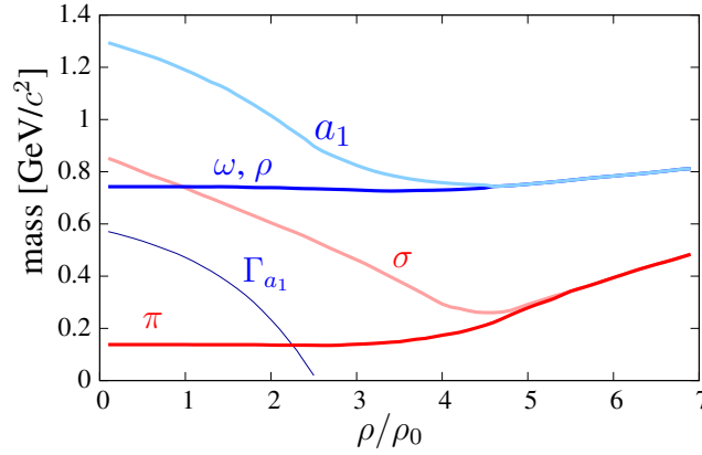
Figure 1.6: Prediction of the NJL model for meson masses as function of density. The decay width a_1 \rightarrow \bar{q}q is also shown. Beyond a critical density the chiral partners ( \pi , \sigma ) and ( \rho , a_1 ) are degenerate in mass. [6]
