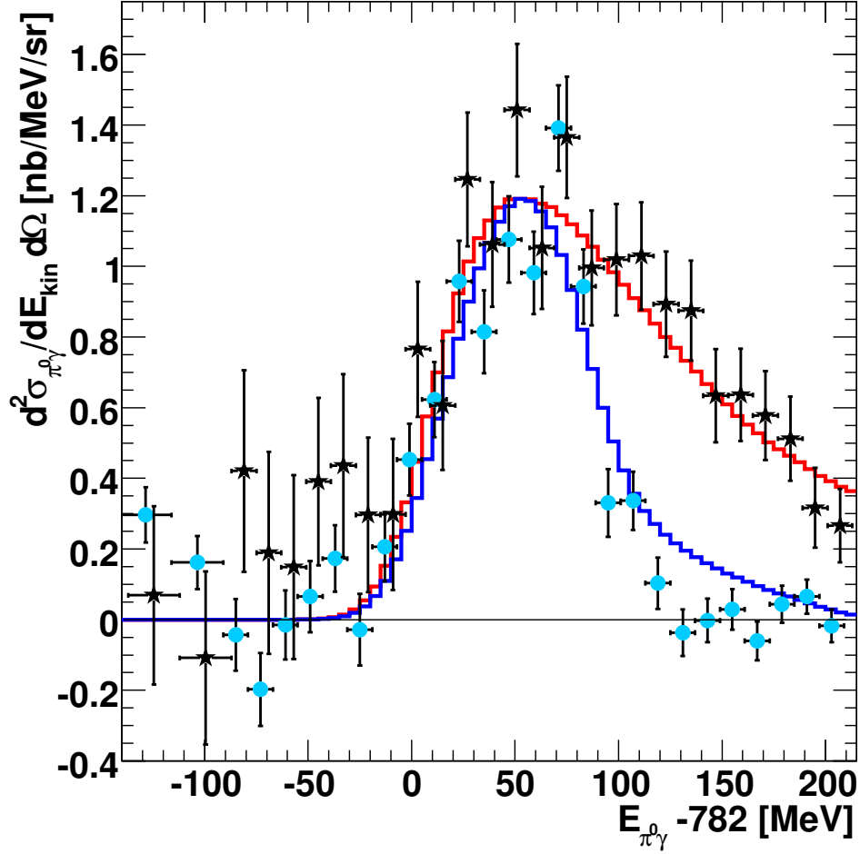
Figure 7.3: Comparison of the experimental double differential cross section (light blue points: LH 2 data, black stars: carbon data) to Monte Carlo calculations (blue histogram: LH 2 target, red histogram: carbon target with Fermi motion). The histograms and the blue data points are scaled to the maximum of the fit to the carbon data (see figure 7.1(a)); data points are shifted by \pm 2 MeV with respect to each other to avoid overlap. For all distributions a polar angle range of the proton 1^\circ < \Theta_p < 11^\circ is requested. For details see figure 5.2 and section 5.1.
