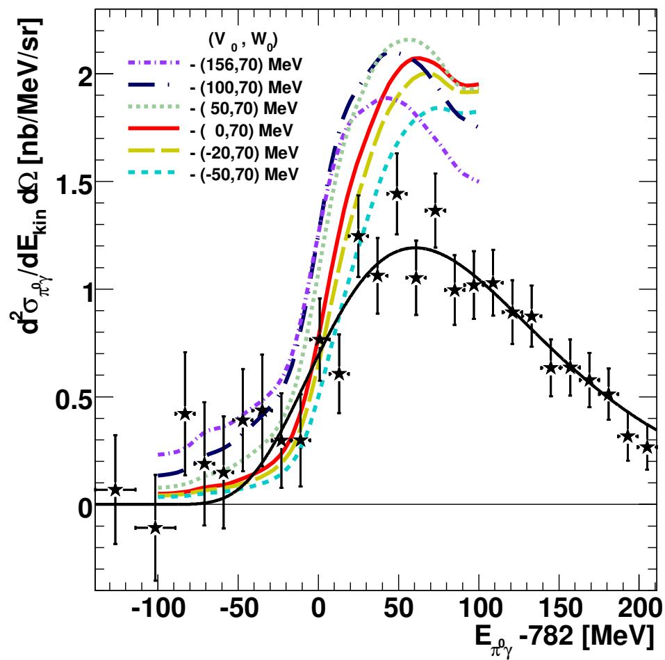
Figure 7.5: Comparison of the predictions by Nagahiro et al. multiplied by the branching ratio of figure 7.4(b) to the carbon data.
