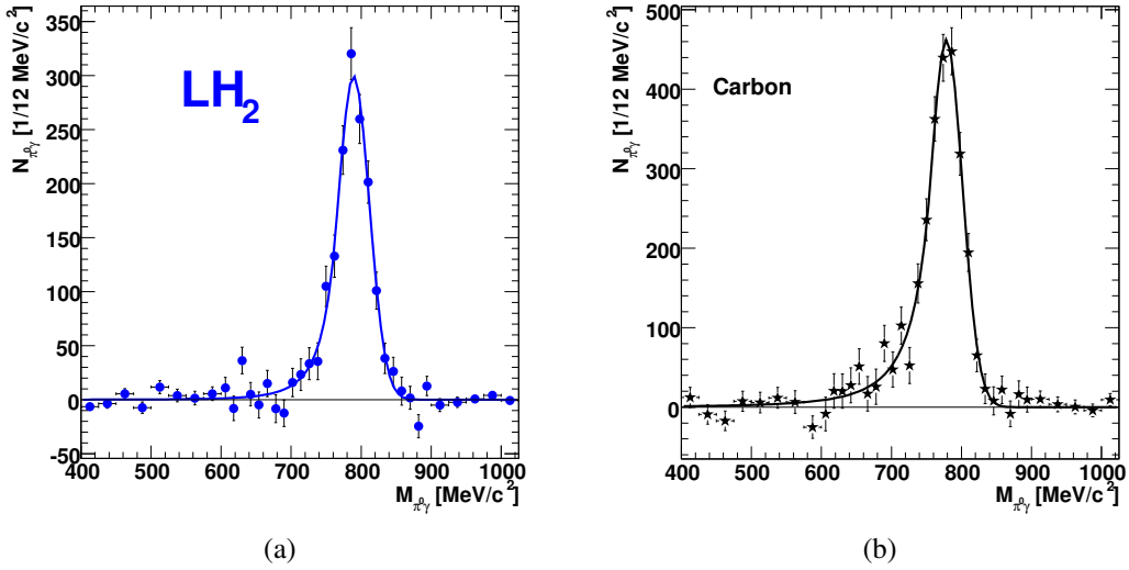
Figure 4.28: \pi^0\gamma -invariant mass signal after background subtraction for (a) \text{LH}_2 data and (b) carbon data. Both distributions are fitted with the Crystal Ball function [59]. The widths are \sigma_{\text{LH}_2} = 22.5 MeV and \sigma_{\text{carbon}} = 23.0 MeV.
