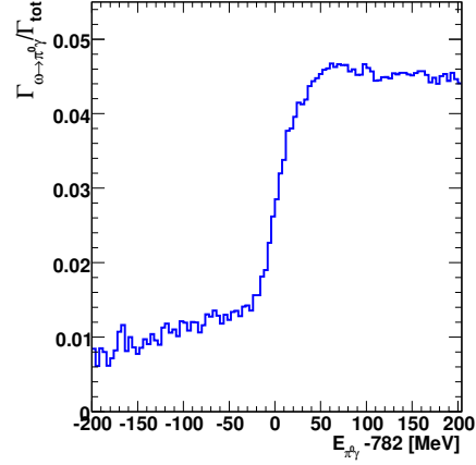
(b) Branching ratio for the decay of bound and quasi-free \omega -mesons into the \pi^0\gamma -channel, deduced by GiBUU calculations.
