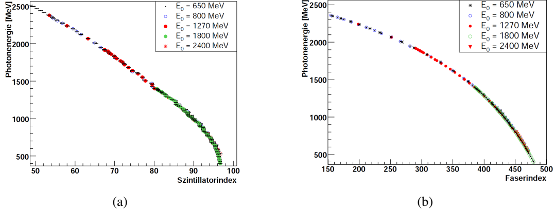
Figure 2.5: Energy calibration of the tagger-bars (a) and -fibers (b) [27].
