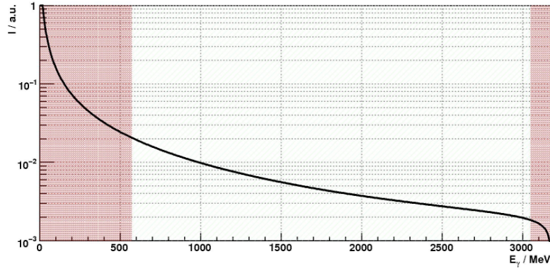
Figure 2.3: Energy coverage of the tagger for an incident electron energy of 3.2 GeV. The shaded energy regions are not tagged. [27]
