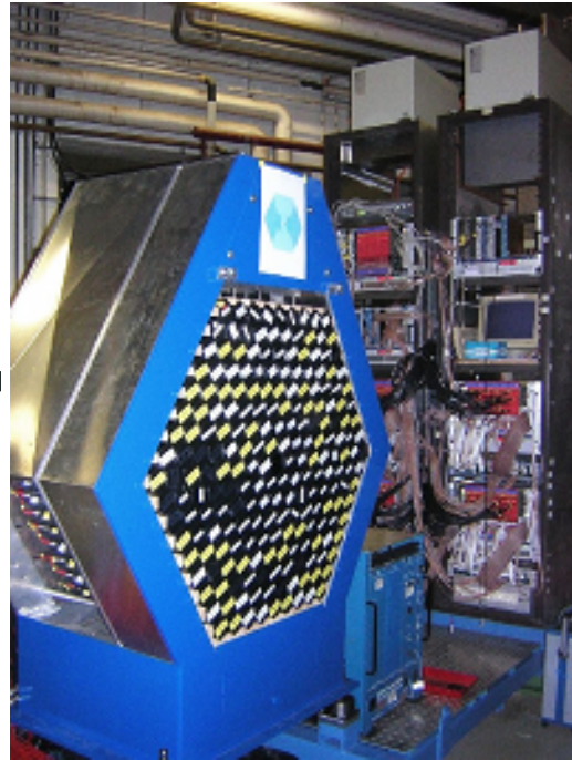
Figure 2.12: Arrangement of crystals inside the MiniTAPS wall. One crystal is removed from the center of the setup. Photons which did not generate hadronic reactions will leave the setup through this hole.
