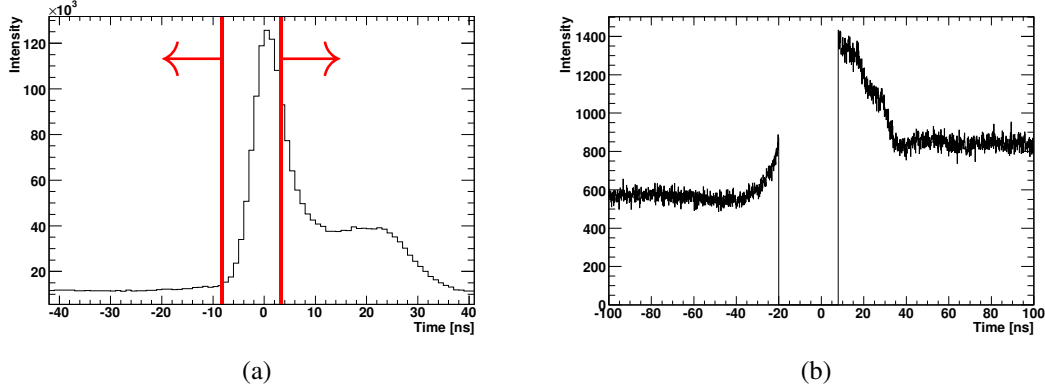
Figure 4.13: Aerogel-Čerenkov detector time distribution (LH 2 beamtime, October 2008) (a) before the anti-cut and (b) after the anti-cut on the prompt peak.
