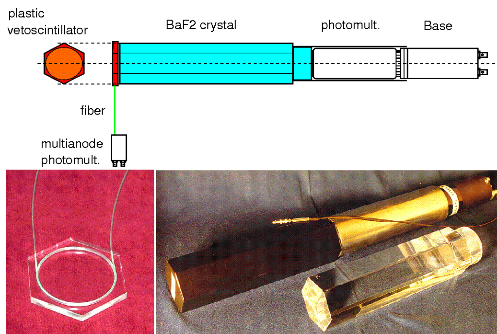
Figure 2.11: Schematic view (above [37]) and photograph (below) of one MiniTAPS module consisting of a BaF 2 crystal and a plastic veto.
