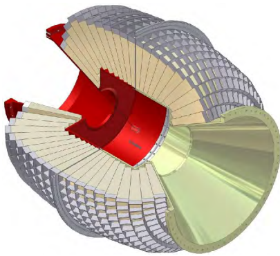
Figure 2.8: CAD of the Crystal Barrel detector [26].
