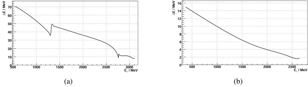
Figure 2.4: Energy resolution of the tagger-bars (a) and -fibers (b) for an incident electron energy of 3.2 GeV [27].
