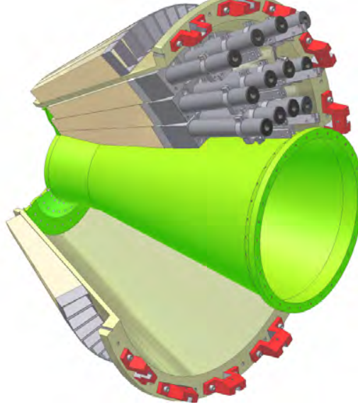
Figure 2.10: CAD of the Forward Plug detector [26].
