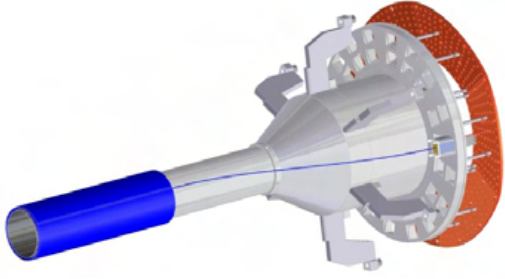
Figure 2.6: Schematic view of the Inner Detector [26].
