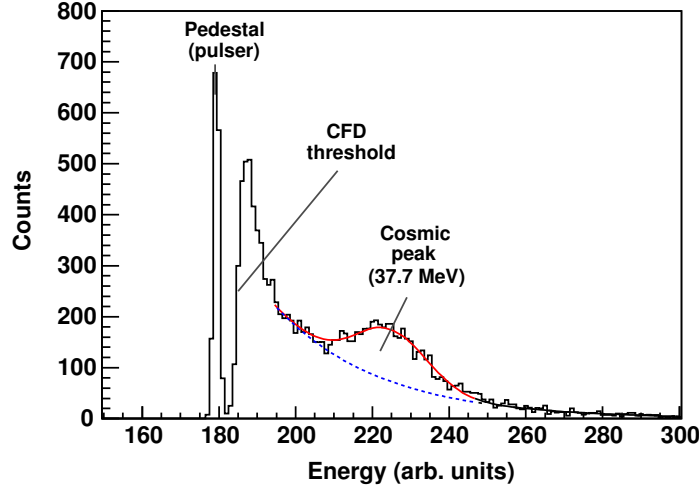
Figure 4.2: Typical cosmic muon spectrum obtained with MiniTAPS. The pedestal peak (zero energy peak), the CFD threshold and the minimum ionizing peak of cosmic muons are clearly recognizable. [49]
