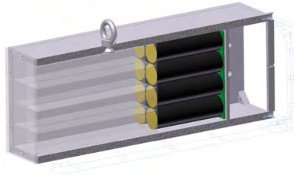
Figure 2.16: CAD of the Gamma Intensity Monitor [26].
