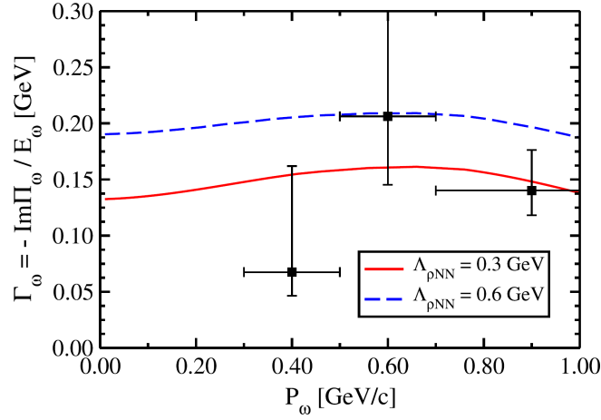
Figure 1.11: Momentum dependence of \Gamma_{\omega \rightarrow \rho\pi} at saturation density for on-shell \omega -mesons compared to data from [12]. [13]
