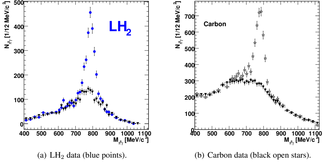
Figure 4.25: \pi^0\gamma -invariant mass signal with normalized background contribution (scaled, black triangles).
