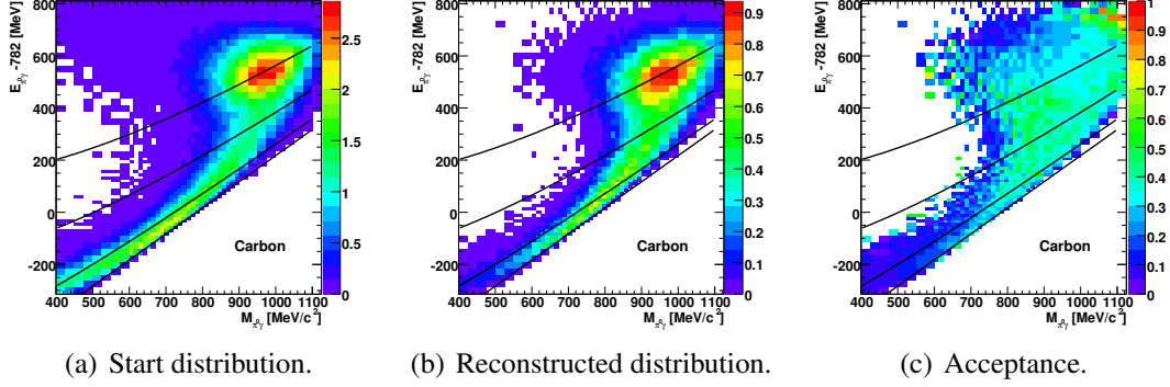
Figure F.1: \pi^0\gamma -simulation for E_\gamma = 1450 - 1650 MeV on carbon.
