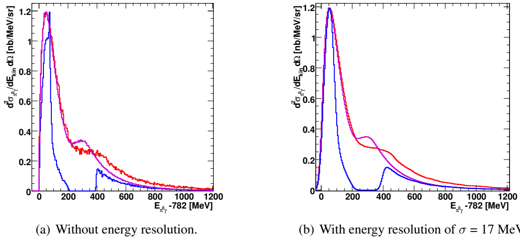
Figure 5.2: \pi^0\gamma -kinetic energy start distribution for E_\gamma = 1250 - 3100 MeV. The kinetic energy of the \omega -meson is plotted for production on a free proton (blue), on a bound proton with Fermi motion (red) and in addition with a constant proton removal energy E_{rem} of +20 MeV (magenta) for (a) without energy resolution and (b) with energy resolution of \sigma = 17 MeV. All curves are scaled to the maximum of the fit to the experimental cross section on carbon (see figures 7.1(a) and 7.3).
