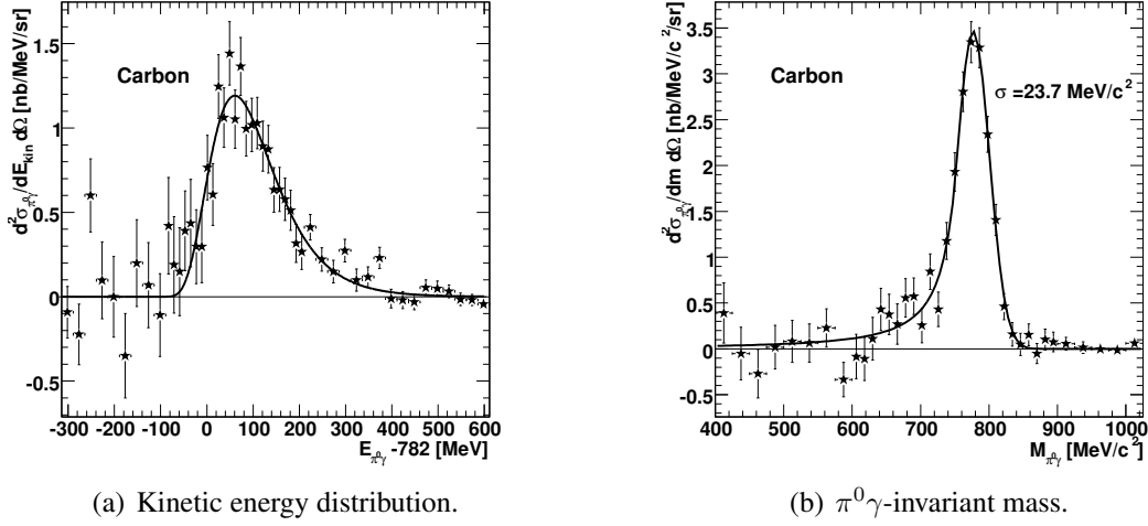
Figure 7.1: Double differential cross section for the photoproduction of \omega -mesons off carbon in coincidence with a proton within 1^\circ < \Theta_p < 11^\circ (a) as a function of the total energy of the \pi^0\gamma -pair minus 782 MeV and (b) as a function of the \pi^0\gamma -invariant mass, fitted with the Crystal Ball function [59]. The width is \sigma_{\text{carbon}} = 23.7 \text{ MeV}/c^2 .
