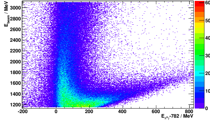
Figure 5.3: Correlation between kinetic energy and beam energy for \omega -mesons for recoil protons in MiniTAPS ( 1^\circ < \Theta_p < 11^\circ ). The plot shows two different branches of the produced mesons: One where the mesons go forward and one where they go backward in the CM-system. By applying a cut on the beam energy one can separate the two branches in the projection on the kinetic energy. To determine the peak position of this distribution only the branch with the low energy mesons should be taken.
