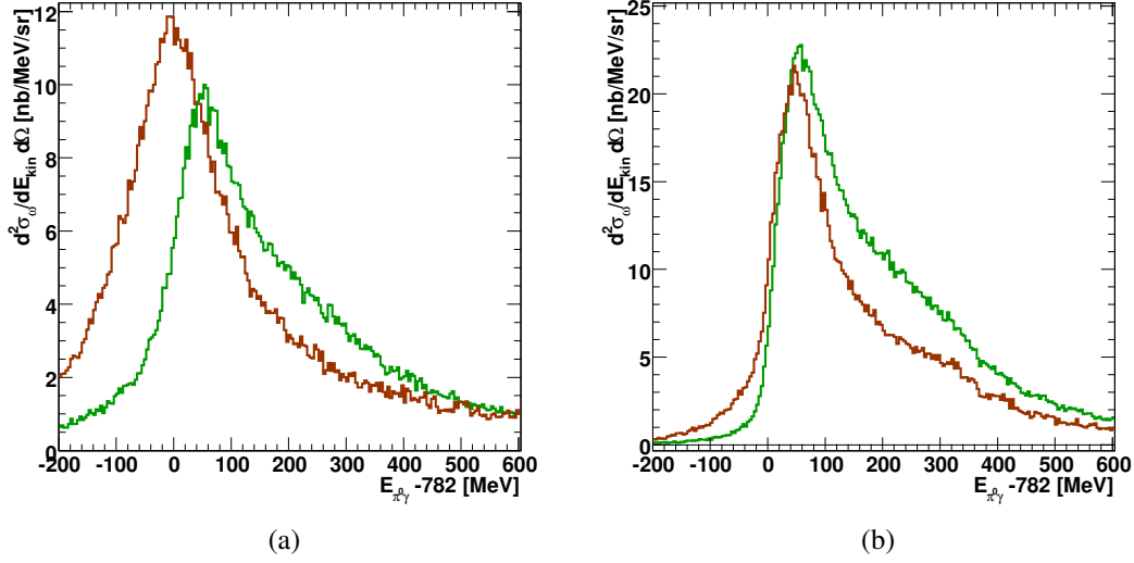
Figure 6.6: Energy spectra of \omega -mesons in coincidence with a forward going proton (with proton FSI) for two different in-medium scenarios: Collisional broadening only (green) and in addition an attractive potential of -125 MeV (brown). (a): Energy spectrum of \omega -mesons at the time of absorption. (b): Energy spectrum of \omega -mesons at the time of decay.
