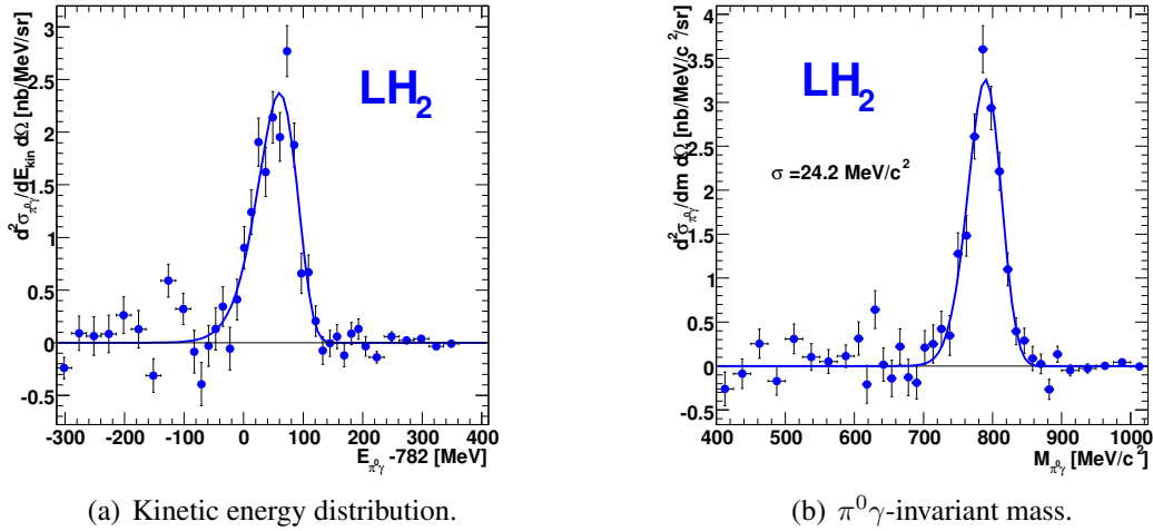
Figure 7.2: Double differential cross section for the photoproduction of \omega -mesons off the free proton in coincidence with a proton within 1^\circ < \Theta_p < 11^\circ (a) as a function of the total energy of the \pi^0\gamma -pair minus 782 MeV and (b) as a function of the \pi^0\gamma -invariant mass, fitted with the Novosibirsk function [54, 55]. The width is \sigma_{LH_2} = 24.2 \text{ MeV}/c^2 .
