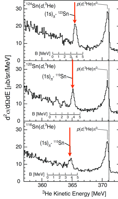
Figure 1.13: Double differential cross section for pionic tin isotopes as function of the kinetic energy of the outgoing Helium nucleus. The arrows indicate the deeply bound pions in the 1s-state. [16]
