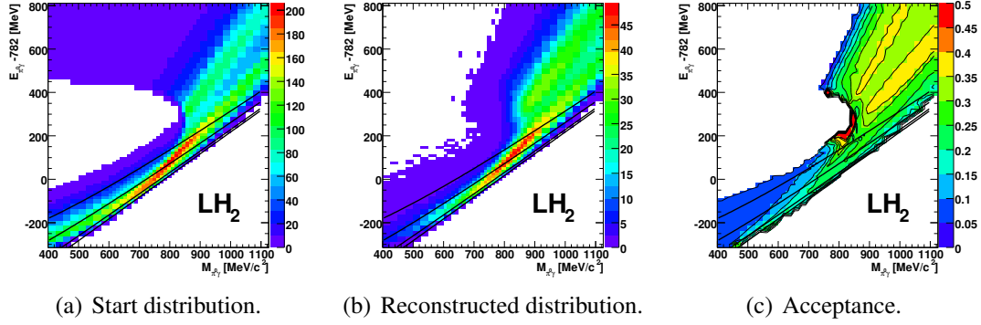
Figure 5.9: \pi^0\gamma -simulation for E_\gamma = 1250 - 3100 MeV on a free proton.
