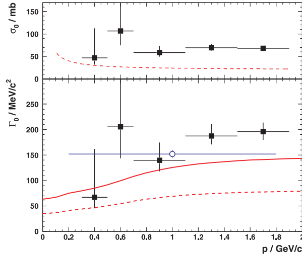
Figure 1.10: Upper part: The inelastic \omega N cross section extracted from the Glauber analysis in comparison to the cross section used in GiBUU. Lower part: Measured widths of the \omega -meson inside the nuclear medium as a function of the \omega -momentum in comparison to the GiBUU model calculations (red dashed line), and after a fit to the data (solid red line). [12]
