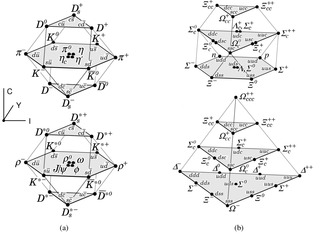
Figure 1.1: (a) Hexadecuplets of pseudoscalar and vector mesons. On the I -, C -, Y -axes the isospin component I_z , the charm quark content C and the hypercharge Y=B+S-C/3 are shown, respectively. (b) Multiplets of baryons. [1]
