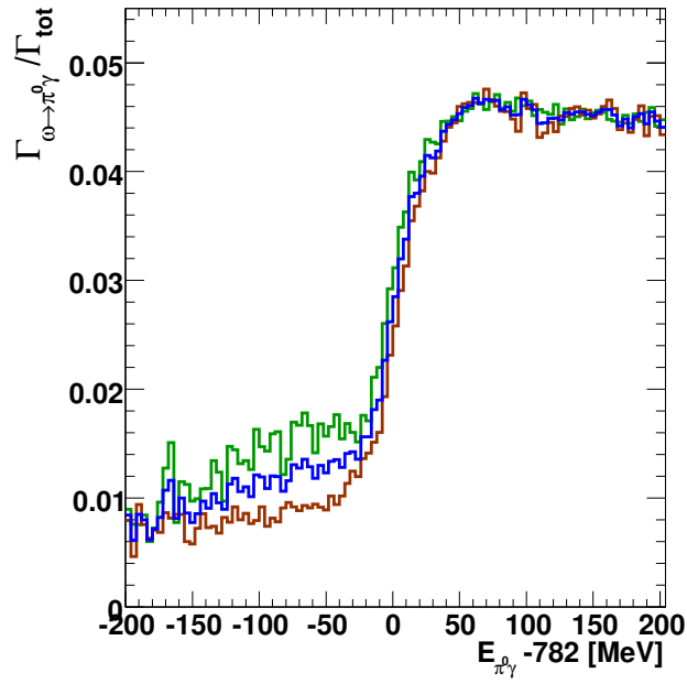
Figure 6.8: Effective branching ratio as function of the \omega -kinetic energy for two different in-medium scenarios. Green: Collisional Broadening only, brown: additional attractive potential of -125 MeV, blue: average of both spectra. The green and brown curves are the ratio of the two spectra 6.7(b) and 6.7(a).
