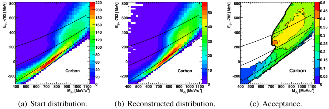
Figure 5.8: \pi^0\gamma -simulation for E_{\gamma} = 1250 - 3100 MeV on carbon.
