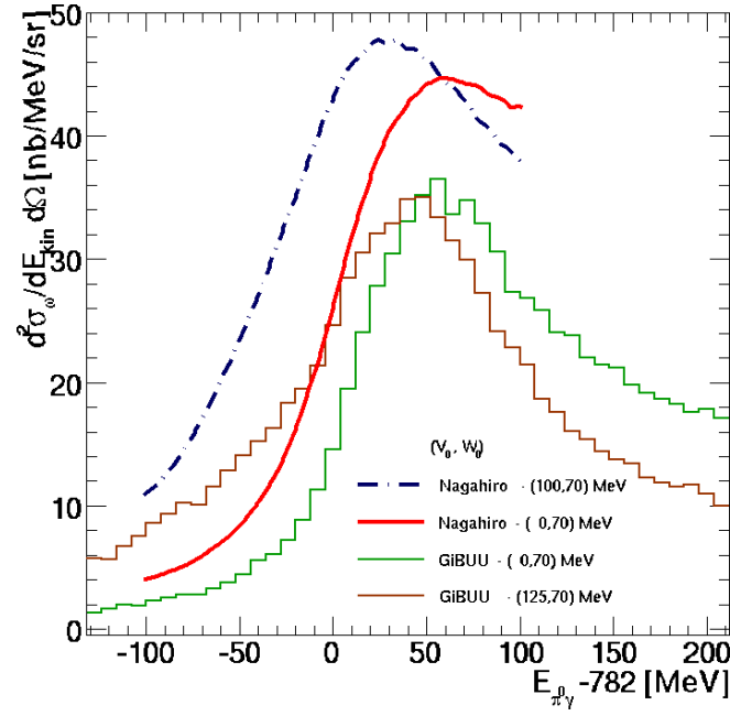
Figure 6.5: Double differential formation cross section (histograms) of \omega -photoproduction in coincidence with a forward going proton in Mini-TAPS ( 1^\circ < \Theta_p < 11^\circ ) for two different in-medium scenarios, using GiBUU: Collisional broadening only \Gamma(\rho_0) = 150 MeV (green) and in addition an attractive potential of V_0(\rho_0) = -125 MeV (brown). For comparison the quantum-mechanical calculations by Nagahiro et al. (see section 1.4) are shown (lines).
