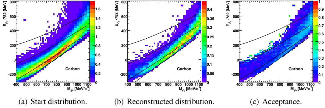
Figure F.4: \pi^0\gamma -simulation for E_\gamma = 2250 - 2450 MeV on carbon.
