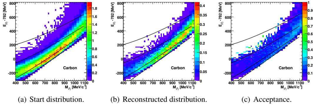
Figure F.5: \pi^0\gamma -simulation for E_\gamma = 2450 - 2650 MeV on carbon.
