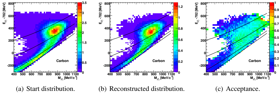
Figure 5.5: \pi^0\gamma -simulation for E_\gamma = 1250 - 1450 MeV on carbon.
