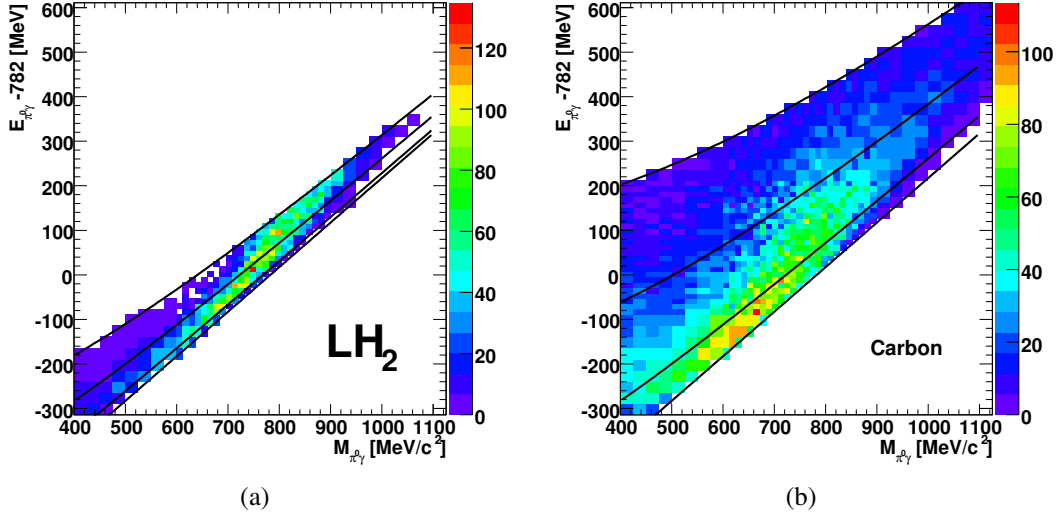
Figure 4.24: Background spectrum (scaled): Two-dimensional plot of total \pi^0\gamma -energy minus 782.65 MeV vs. the \pi^0\gamma -invariant mass for events with four neutral and one charged hit in MiniTAPS for (a) LH 2 data and (b) carbon data. One of the four photons has been omitted in the analysis. The spectrum has been scaled within momentum slices (for details see text).
