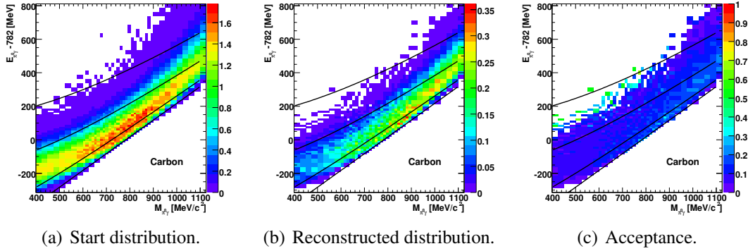
Figure 5.7: \pi^0\gamma -simulation for E_{\gamma} = 2850 - 3100 MeV on carbon.
