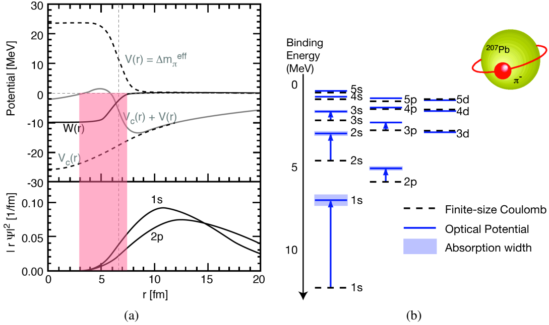
Figure 1.12: (a) Upper panel: Decomposition of the pion-nucleus potential for ^{207}\text{Pb} into the Coulomb potential V_C and the real and imaginary s-wave potential ( V , W ) [14, 15]. Lower panel: Pionic density distribution for 1s- and 2p-states. (b) Calculated level scheme of pionic ^{207}\text{Pb} . Level shifts and widths are indicated by vertical arrows and shaded areas [17].
