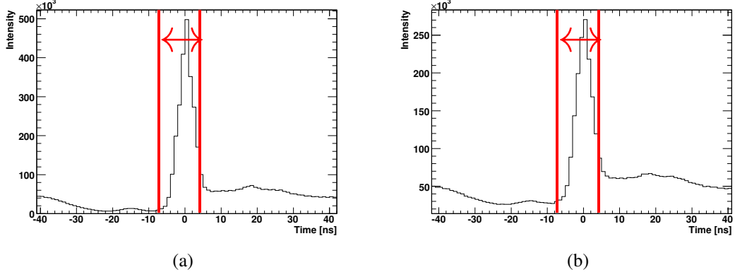
Figure 4.11: Time distributions of hits in the tagger scintillation detectors: (a) Tagger bars and (b) tagger fibers (LH 2 beamtime, October 2008). The cut limits are shown in table 4.1.
