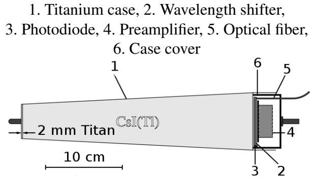
Figure 2.9: Composition of one Crystal Barrel module [33].
