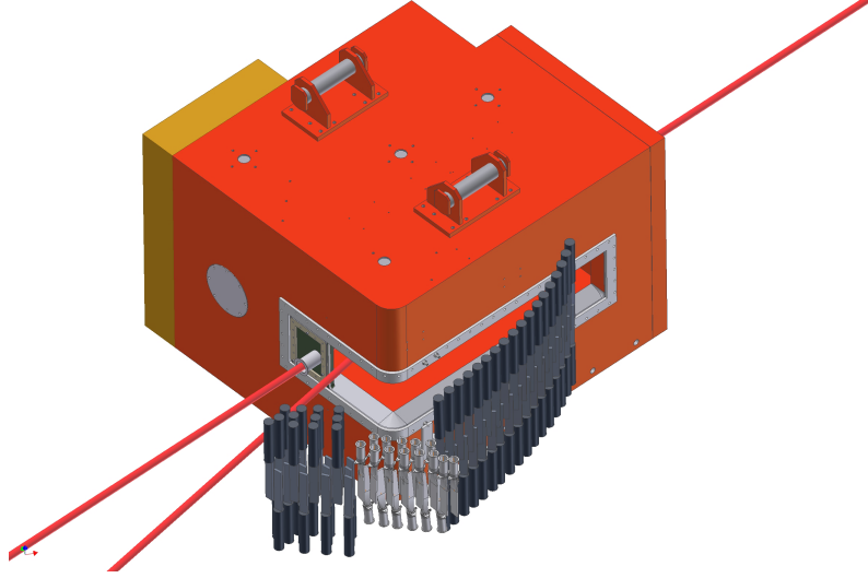
Figure 2.2: CAD of tagger magnet (orange) and the 96 partly overlapping scintillator tagger bars. The electrons arrive from the right side and are deflected towards the scintillator bars. [26]
