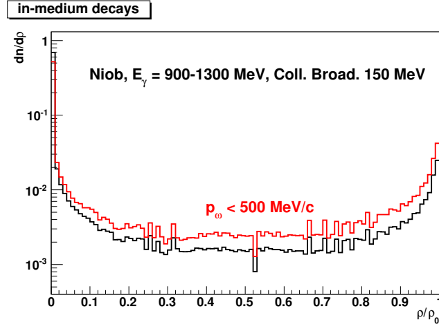
Figure 6.2: Nuclear density distribution for decaying \omega -mesons for all momenta (black) and momenta p_\omega < 500 MeV/c (red). This condition reduces the total \omega -yield by 25%, but enhances the average density at the decay point.
