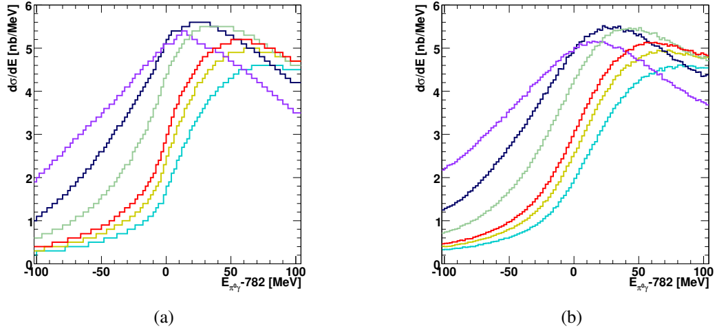
Figure 1.19: Calculated spectra from figures 1.16, 1.17 and appendix B; integrated over angle and summed over energy. The curves are shown for an imaginary part of the potential of W_0 = 70 MeV and different real parts V_0 : -156 MeV (violet), -100 MeV (dark blue), -50 MeV (green), 0 MeV (red), +20 MeV (yellow), +50 MeV (light blue). (a) Without energy resolution, (b) with energy resolution of \sigma = 17 MeV.
