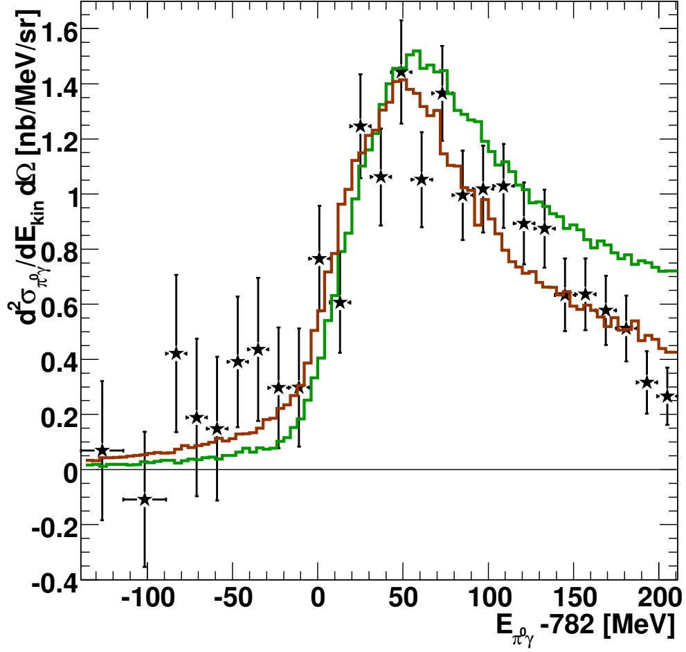
Figure 7.6: Comparison of the GiBUU calculations to the carbon data for two different in-medium modification scenarios (brown histogram: collisional broadening and mass shift of -125 \text{ MeV}/c^2 ; green histogram: only collisional broadening with width \Gamma(\rho = \rho_0) = 150 \text{ MeV} ).
