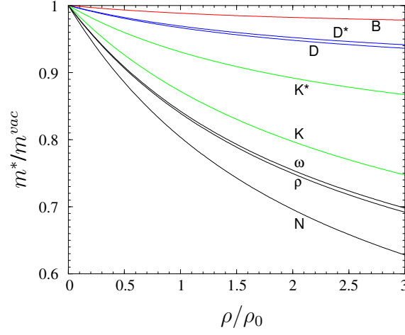
Figure 1.7: Prediction of the QMC model for meson masses as function of density. [10]
