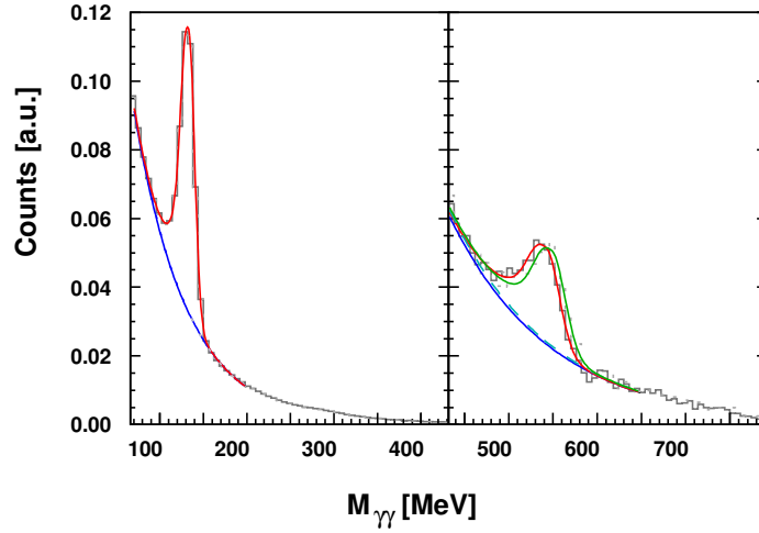
Figure 4.6: The position of the \pi^0 - (left) and \eta -meson invariant mass (right) before and after polynomial calibration. The blue curve shows the background contribution. The position of the pion is unchanged, while the position of the \eta -meson is shifted down roughly by 10 MeV/ c^2 to the nominal mass of the \eta -meson. [4]
