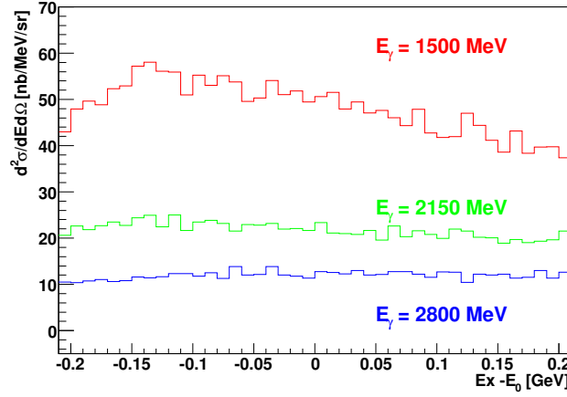
Figure 6.4: Double differential cross section for a forward going proton assuming photoproduction of an \eta' -meson. Three different incoming photon energies are plotted.
