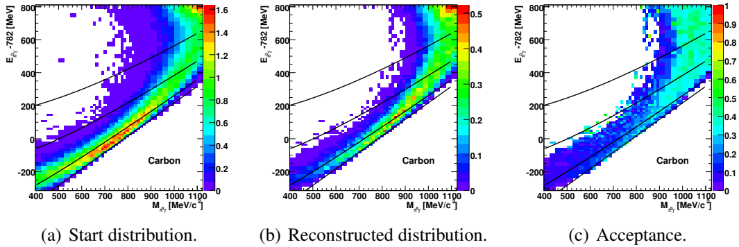
Figure F.3: \pi^0\gamma -simulation for E_\gamma = 1850 - 2050 MeV on carbon.
