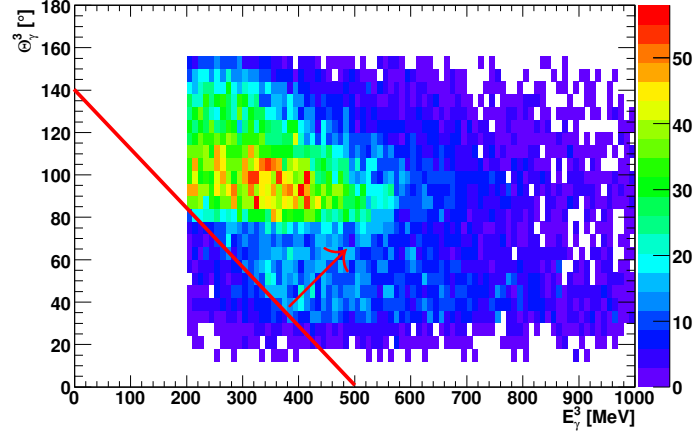
Figure 4.18: Two-dimensional spectrum of the polar angle of the bachelor photon as a function of its energy (carbon data). Events in the area indicated by the arrow are analyzed further.
