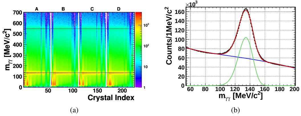
Figure 4.4: (a) Two-photon invariant mass as function of the crystal index in Mini-TAPS. 56 channels belong to one sector, but only 54 are read out. This is the reason why the last two channels of the sectors do not hold any information.
