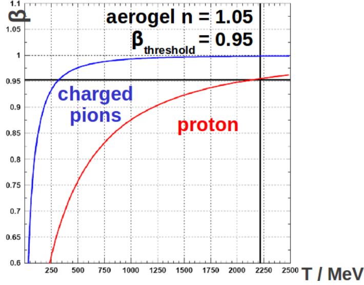
Figure 2.13: Plot of the \beta -factor ( \beta = v/c ) of charged pions and protons as function of the kinetic energy [38]. The threshold \beta_{\text{thrsh}} for the used aerogel and the threshold energy for protons are shown.
