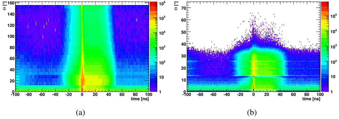
Figure 4.12: Two-dimensional plot of polar angle vs. calibrated time for particles marked as “charged” or “neutral” depositing energy in the scintillation crystals (LH 2 beamtime, October 2008). For this distinction the read-out information of Inner Detector, Forward Plug veto detector and Mini-TAPS veto detector are used. Please note that the Crystal Barrel detector itself does not provide time information. The cut limits for the various detectors are shown in table 4.1.
