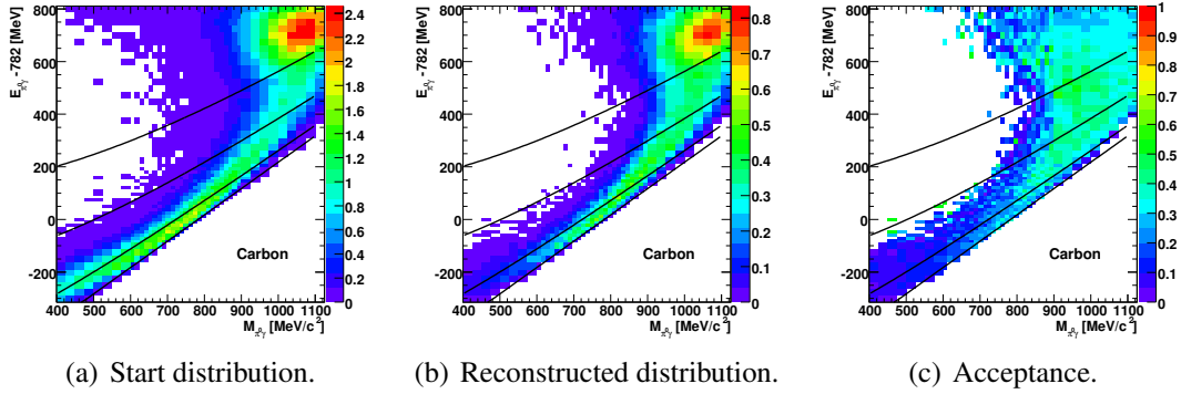
Figure F.2: \pi^0\gamma -simulation for E_\gamma = 1650 - 1850 MeV on carbon.
