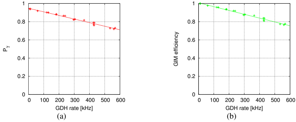
Figure 4.30: Tagger rate dependency for (a) the P_\gamma -value and (b) deduced GIM efficiency derived by (a) (Niobium beamtime, January 2014).
