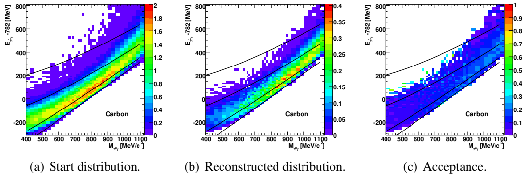
Figure F.6: \pi^0\gamma -simulation for E_\gamma = 2650 - 2850 MeV on carbon.
