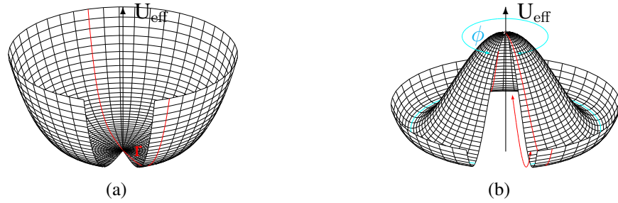
Figure 1.3: In figure (a) (restored symmetry), the minimum of the potential is in the center, therefore the ground state is invariant under rotation (no spontaneous breaking of the symmetry), while in figure (b) (spontaneously broken symmetry) the ground state is located at a finite distance from the center where the potential actually has a local minimum. The red lines represent the radial excitation, the cyan line the rotational mode. [4]
