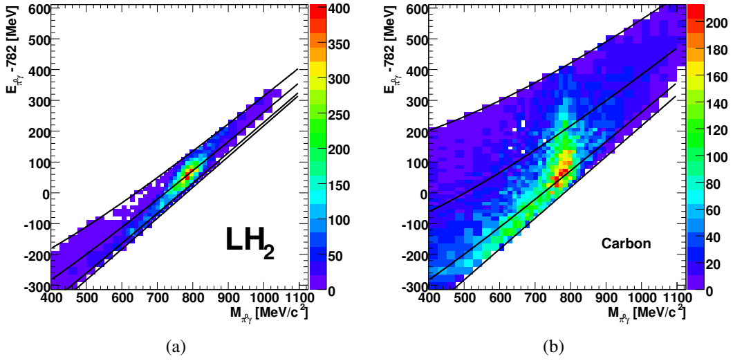
Figure 4.20: Signal spectrum with background contribution.
