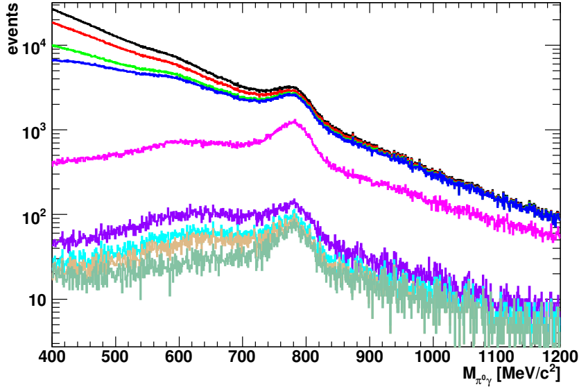
Figure 4.19: \pi^0\gamma -invariant mass spectrum after subsequent application of different cuts (carbon data). The first four histograms show the impact of the following cuts: no cut (black), E_{beam} (red), E_{\gamma^3} (green), T_{\pi^0} (blue). As a result, the shape of the spectra is hardly changed. In contrast, the missing mass cut drastically reduces the background (pink) and enhances the signal to background ratio. The cut on the proton polar angle reduces the statistics a lot (violet). The proton band cut reduces background since the proton is identified explicitly and not only a “charged” particle (light blue). The beige histogram shows the distribution after additionally applying the cuts on the relative angles, the energies of the single photons and the restriction for photons not to be registered in the MiniTAPS detector. In the last step (grey) the cut on the polar angle vs. energy of the bachelor photon is applied.
