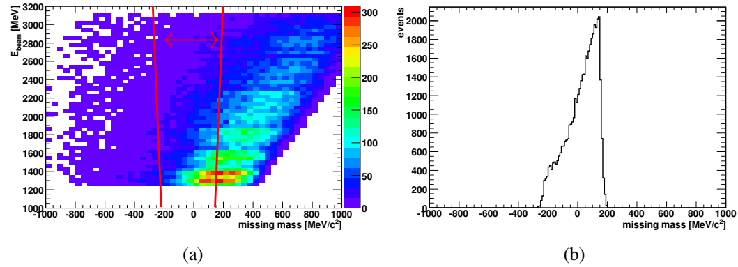
Figure 4.17: Missing mass distribution MM(\gamma N \pi^0 \gamma) for the carbon data. (a) Incident photon energy as a function of the missing mass. The cut limits are indicated by red lines. b) The projection onto the x -axis after the applied cut.
