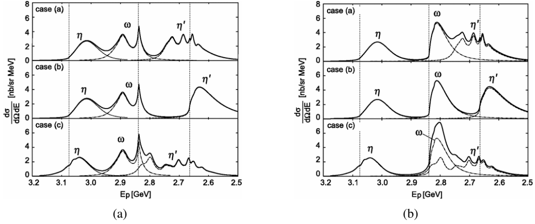
Figure 1.15: Calculated spectra of ^{12}\text{C}(\gamma, p) reactions for \eta -, \omega - and \eta' -mesic nucleus formation at E_\gamma = 2.7 GeV are shown as functions of the emitted proton energies in the final states. The vertical dashed lines indicate the production thresholds of the \eta -, \omega - and \eta' -mesons. The \omega -nucleus potential is assumed to be (a) attractive and (b) repulsive. [23]
