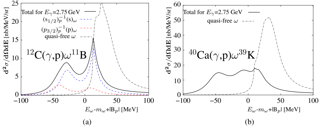
Figure 1.14: Missing energy spectra at E_\gamma = 2.75 GeV for the (a) ^{12}\text{C}(\gamma, p)\omega^{11}\text{B} reaction and (b) for the ^{40}\text{Ca}(\gamma, p)\omega^{39}\text{K} reaction ( |B_p| is the binding energy of the bound initial proton) [19].
