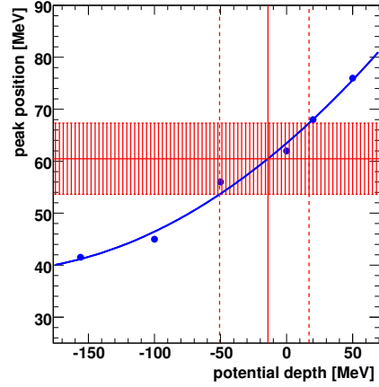
(d) Correlation between the potential depth and the peak position of the total energy distribution (blue points). The blue curve represents a fit. The dashed red area corresponds to the measured peak position, including the error band.
