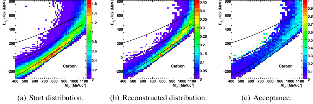
Figure 5.6: \pi^0\gamma -simulation for E_{\gamma} = 2050 - 2250 MeV on carbon.
