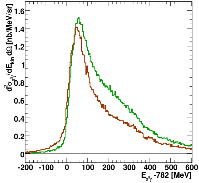
Figure 6.9: Spectra of \omega -mesons in coincidence with a forward going proton with kinetic energy larger than 100 MeV after FSI of all particles for two different in-medium scenarios: Collisional broadening only (green) and in addition an attractive potential of -125 MeV (brown).
