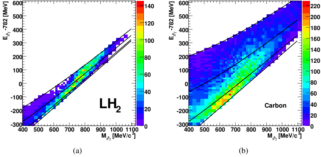
Figure 4.21: Background spectrum (not scaled): Two-dimensional plot of total \pi^0\gamma -energy minus 782.65 MeV vs. the \pi^0\gamma -invariant mass for events with four neutral and one charged hit in MiniTAPS for (a) LH 2 data and (b) carbon data. One of the four photons has been omitted in the analysis.
