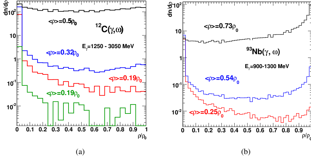
Figure 6.1: GiBUU simulations: Nuclear density distributions for \omega -photoproduction on (a) carbon and (b) niobium nucleus.
