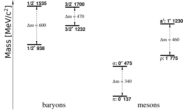
Figure 1.2: Masses of selected hadrons and their chiral partners (not to scale) [1]. The mass-split between the chiral partners is comparable to the masses of the hadrons.
