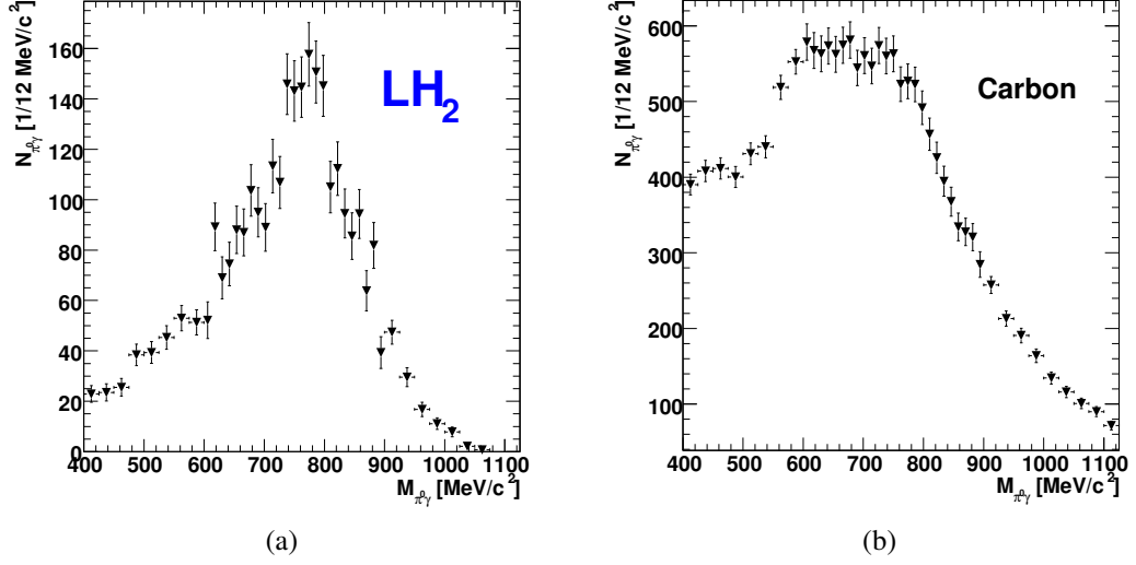
Figure 4.22: \pi^0\gamma -invariant mass background spectrum (not scaled) for (a) LH 2 data and (b) carbon data.
