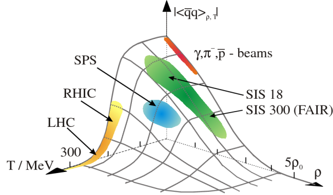
Figure 1.5: Dependence of the chiral condensate on density and temperature. Indicated are the areas where modern accelerators can probe the chiral condensate. [5]
