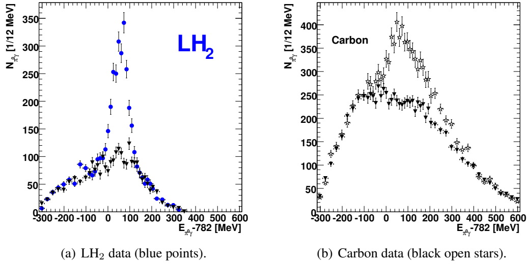
Figure 4.26: E_{\pi^0\gamma} - 782.65 MeV signal spectrum with normalized background contribution (scaled, black triangles).
