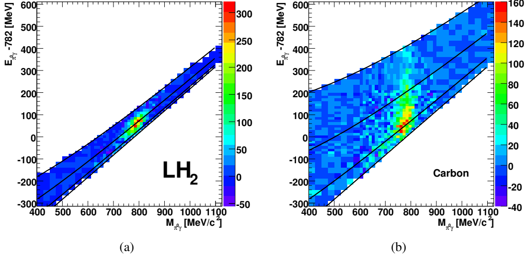
Figure 4.27: Two-dimensional signal spectrum after background subtraction for (a) \text{LH}_2 data and (b) carbon data.
