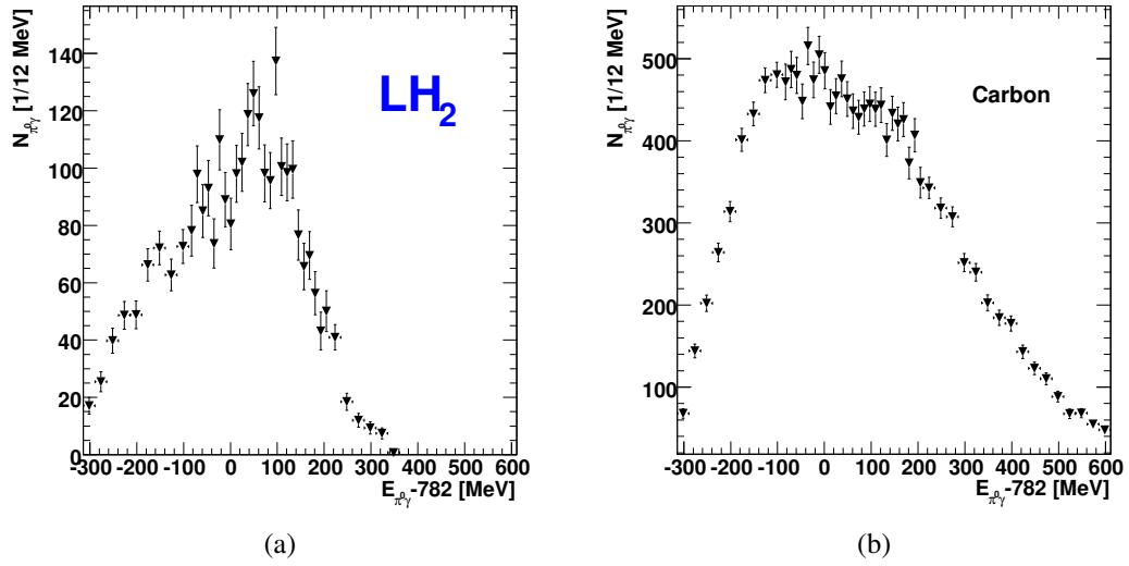
Figure 4.23: E_{\pi^0\gamma} - 782.65 MeV background spectrum (not scaled) for (a) LH 2 data and (b) carbon data.
