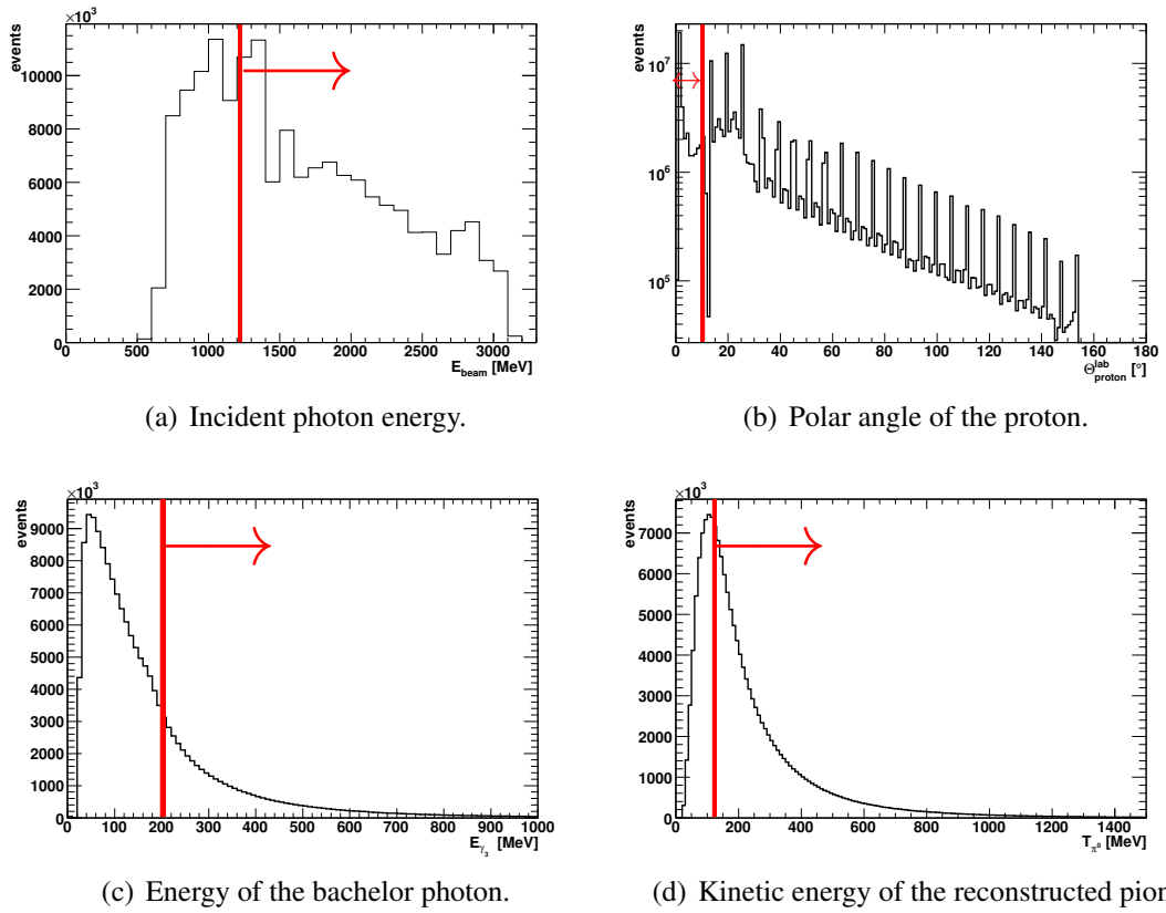
Figure 4.14: Spectra of selected kinematic quantities (carbon data). The cut limits are indicated by red lines and arrows.
