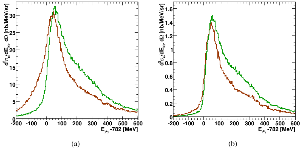
Figure 6.7: Spectra of \omega -mesons in coincidence with a forward going proton (with proton FSI) for two different in-medium scenarios: Collisional broadening only (green) and in addition an attractive potential of -125 MeV (brown). (a): Spectrum of the sum of figures 6.6(a) (absorption) and 6.6(b) (decay) (denominator). (b): Spectrum after FSI of all particles and reconstruction of \pi^0\gamma -pairs (numerator).
