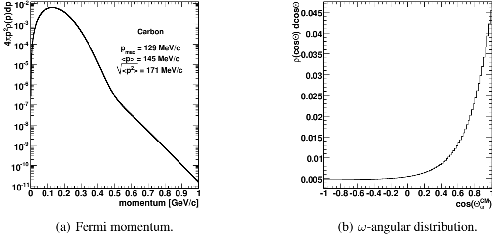
Figure 5.1: Fermi momentum distribution and angular distribution used for the event generator.
