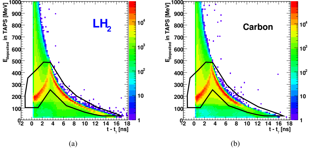
Figure 5.4: Reconstructed distribution: Energy deposited in the MiniTAPS detectors as a function of the time-of-flight. The proton band cut is indicated for a simulation on (a) free proton and (b) carbon target. No time resolution has been folded in.
