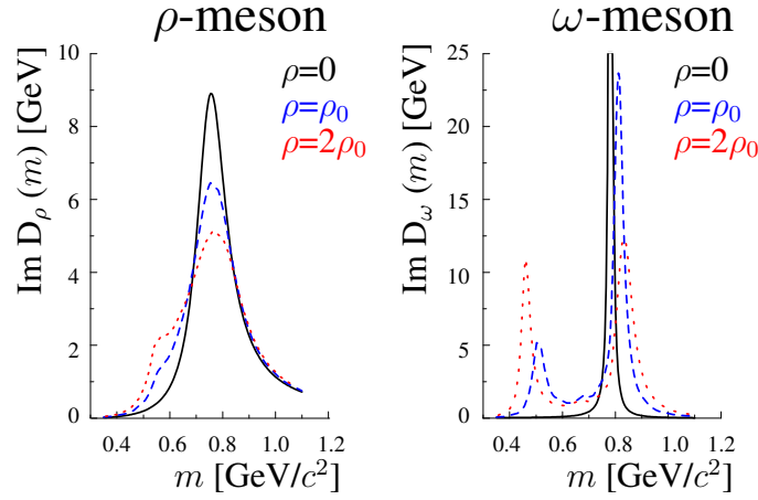
Figure 1.8: Prediction of a hadronic model [11] for the imaginary part of the \rho - and \omega -meson spectral functions inside nuclear matter at \rho = 0 , \rho = \rho_0 and \rho = 2\rho_0 .
