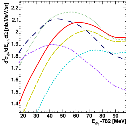
(c) Double differential \pi^0\gamma -cross sections derived from (a) by multiplying with (b).
