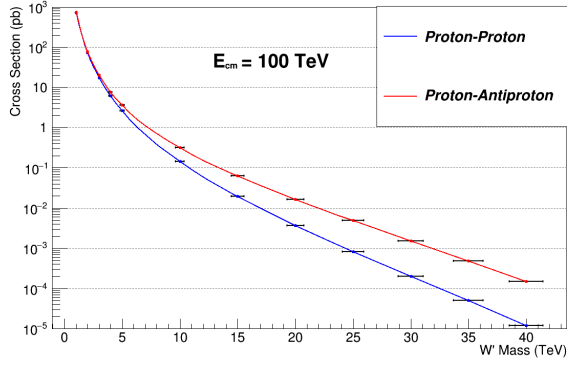
Figure 2: W' cross section as a function of the mass using pp and p\bar{p} collisions with E_{\text{cm}} = 100 TeV using MadGraph [12].
