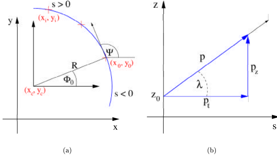
Figure 6.5: Projection of a helix onto the transverse plane (a) and onto the bend plane (b)
