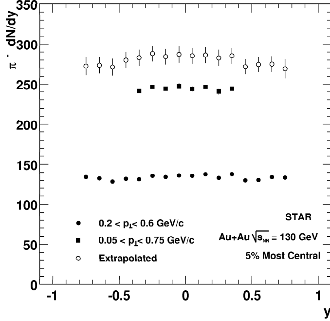
Figure 10.5: \pi^- rapidity distribution. The black circles (squares) are obtained summing the yield between p_\perp 0.2 - 0.6 GeV/ c (0.05 - 0.75) from Fig. 10.3. The hollow data points are the yields obtained using the fit function extrapolated to all p_\perp .
