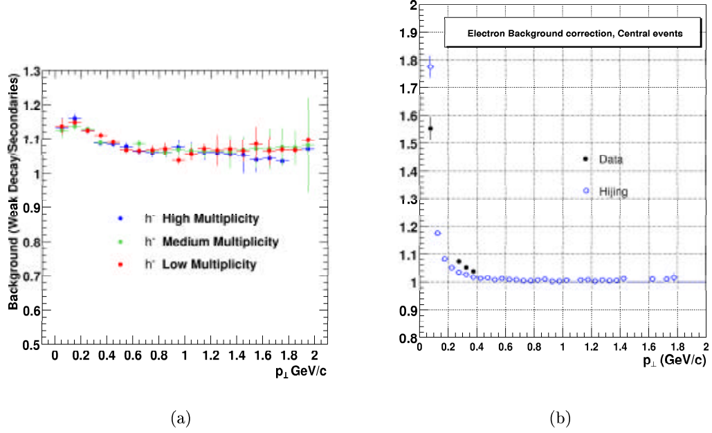
Figure 8.12: Background correction to the h^- spectrum coming from weak decays and secondary interactions in the detector material (a) and electrons (b) as a function of p_{\perp} . The corrections were obtained via HIJING events processed through the STAR offline simulation and reconstruction chain.
