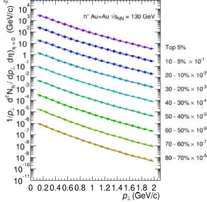
Figure 9.10: The h^- p_\perp distribution for different centralities. The data are scaled down by successive powers of 10 for display purpose.
