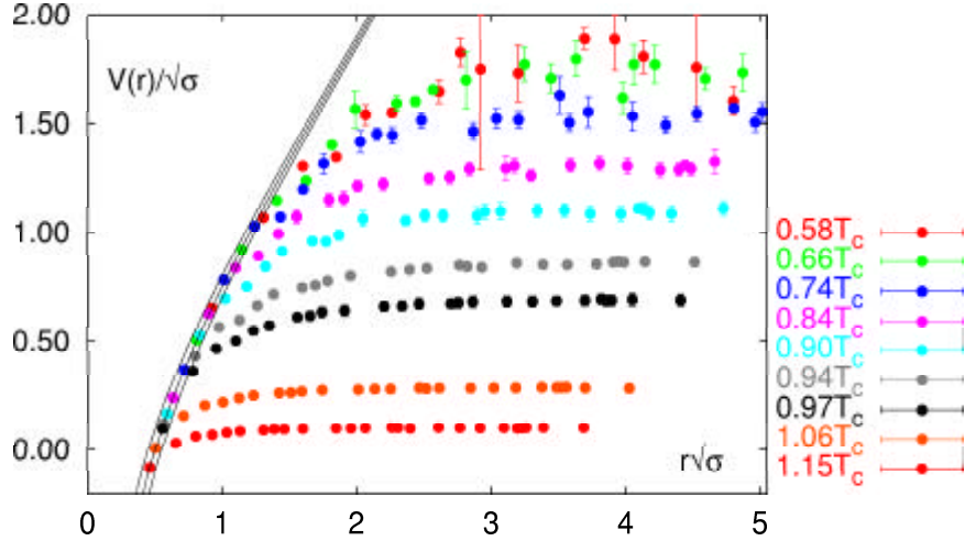
Figure 2.5: The heavy quark effective potential for different temperatures, taken from Ref. [42]. The linear rise of the potential is weakened as one approaches the critical temperature. The solid curves show the Cornell potential V(r) = -\alpha/r + \sigma r with \alpha = 0.25 \pm 0.05 , which is used to normalize the finite temperature free energies at the shortest distance available, r = 1/(4T) .
