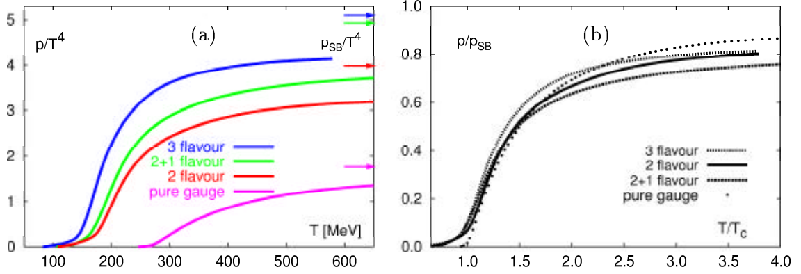
Figure 2.3: The Pressure p in lattice QCD [42]. Left panel: Curves with N_F = 0, 2 and 3 light quarks as well as the “(2+1)” case. Right panel: T axis scaled by the value of T_c for each curve.
