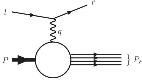
Figure 1: Schematic diagram of deeply inelastic scattering via single boson exchange
