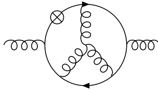
Figure 18: The 3-loop Benz diagram for I_2(N) , Eq. (592).
