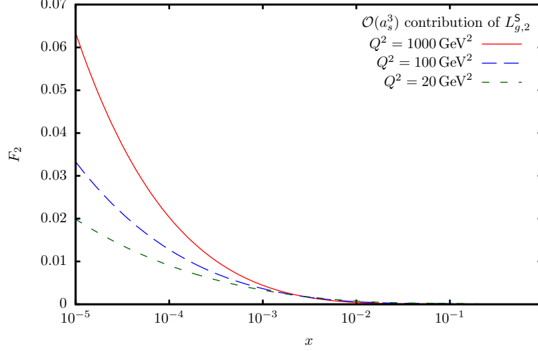
Figure 4: The O(a_s^3) contribution by L_{g,2}^S to the structure function F_2(x, Q^2) .
