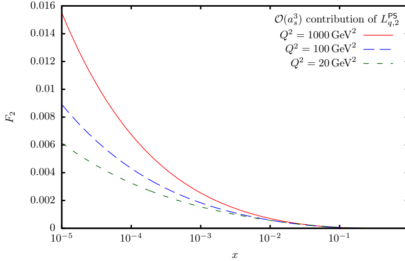
Figure 5: The O(a_s^3) contribution by L_{q,2}^{\text{PS}} to the structure function F_2(x, Q^2) .
