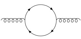
Figure 6: One of the massive fermion loop insertion is effectively rendered massless via a Mellin–Barnes representation.
