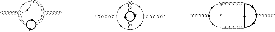
Figure 2: Some typical diagrams contributing to the OME A_{qg,Q} . Thick lines represent heavy quarks, whereas thin ones depict massless fermion flavors.
