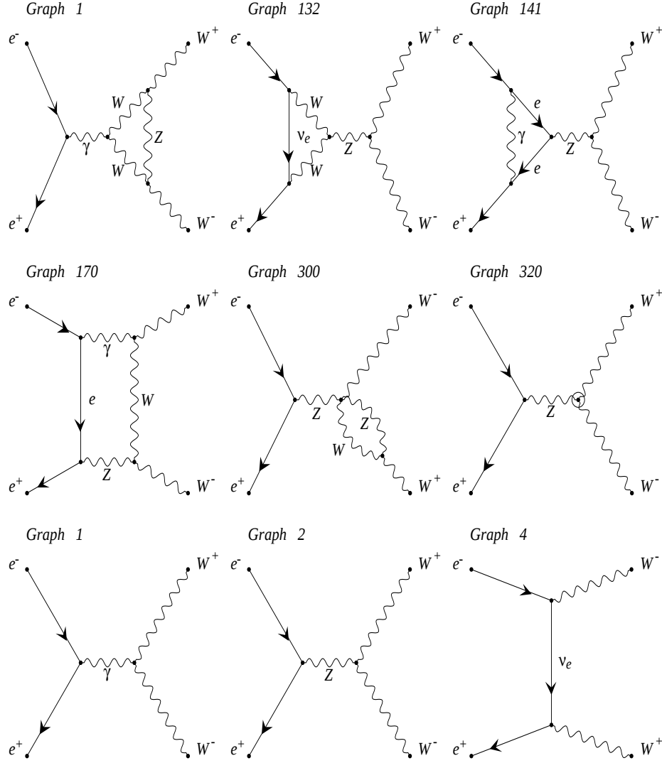
Fig. 1. Typical Feynman diagrams for the process e^-e^+ \rightarrow W^-W^+ .
