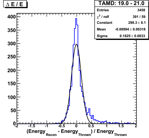
Figure 3: Middle Drum energy resolution for events with energy between 10^{19.0} and 10^{21.0} eV.
