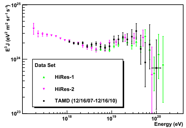
Figure 8: Middle Drum energy spectrum compared to HiRes.
