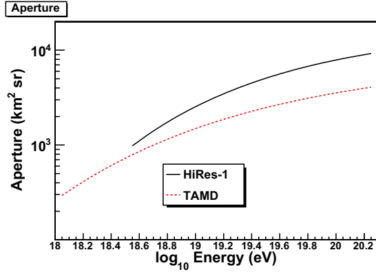
Figure 2: Middle Drum aperture compared to HiRes-1 aperture.
