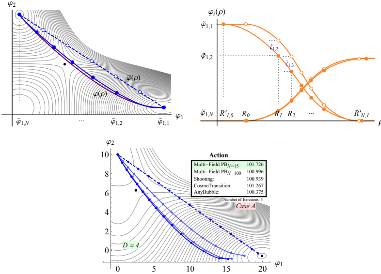
Fig. 4. Top left: Path in field space with the initial straight dashed line Ansatz \bar{\varphi} with empty circles and the first iteration of the PB solution in solid black/blue and full circles; the result from shooting is shown in black/purple. Top right: Iterations of the bounce field configuration for \varphi_1(\rho) . Bottom: Multi-field polygonal solution in D = 4 with N = 15 segmentation points. The starting Ansatz is the straight dashed line connecting the two minima, shown as black dots, together with the saddle point. The solid lines are subsequent iterations that converge to the final path that solves the bounce equations. Insets show the action compared to other approaches.
