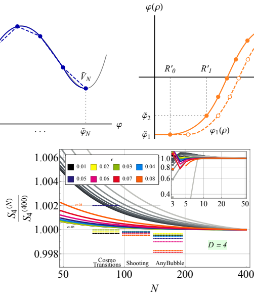
Fig. 3. (Color online) Top left: The polygonal potential with N = 7 field points in dashed black/blue and with the inclusion of non-linear terms in solid black/blue, circumscribed by the potential V in gray. Top right: The bounce field configuration of the polygonal potential on the left, PB dashed and extension PB solid. Bottom: The bounce action S_D^{(N)} for different values of energy gaps between the false and true vacua, similar to figure 2, and computed for different field point values N normalized to N = 400 uniform segmentation in D = 4 . The results are compared with other methods and polygonal bounce in gray.
