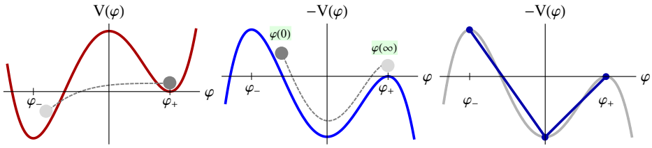
Fig. 1. (Color online) Left: An example of a potential with two minima with unstable false state of vacuum at \varphi_+ and a stable true one at \varphi_- . Center: The potential on the left after an analytic continuation into the Euclidean space. The field starts in a non-trivial value of the field \varphi_0 such that ends up at the true vacuum at infinity. Right: The piece-wise linear potential with two segments in black/blue circumscribed on the potential V in gray.
