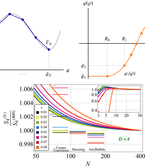
Fig. 2. (Color online) Top left: The polygonal potential with N = 7 field points in black/blue, circumscribed by the actual potential V in gray. Top right: The bounce field configuration of the polygonal potential on the left. Bottom: The bounce action S_D^{(N)} for different values of energy gaps between the false and true vacua. It is computed with the polygonal bounce approach for different field point values N normalized to the maximal N = 400 uniform segmentation in D = 4 . It is compared with other packages in the literature as CosmoTransition [18], AnyBubble [19].
