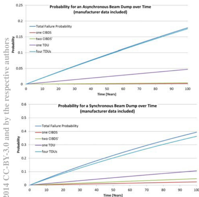
Figure 6: Probability for beam dumps over time.
