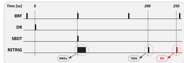
Figure 4: Timing of dump requests.
