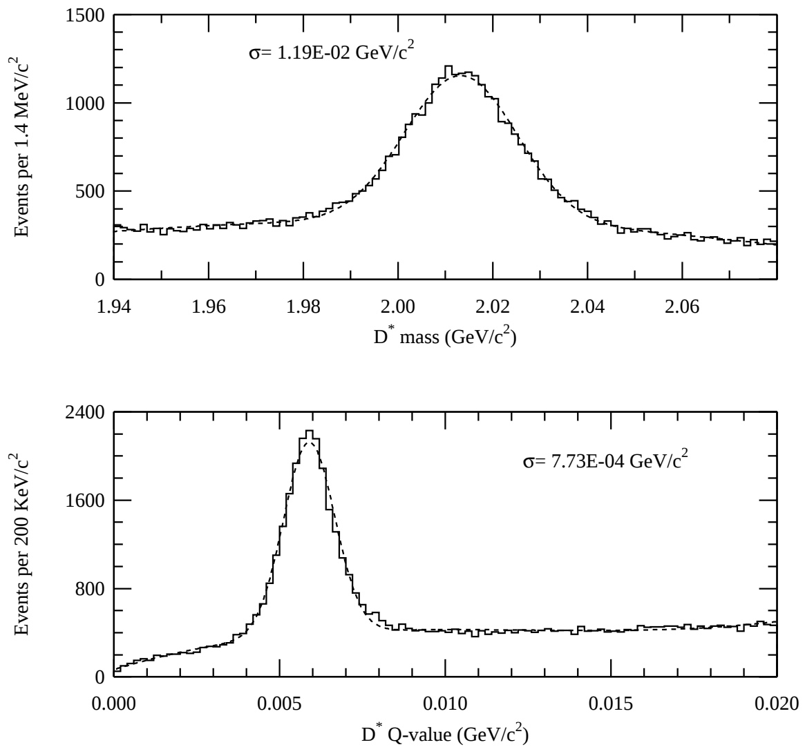
Figure 6.1: Comparison of widths of D^{*\pm} mass and Q -value distributions. Note the difference in horizontal scale in the two histograms.
