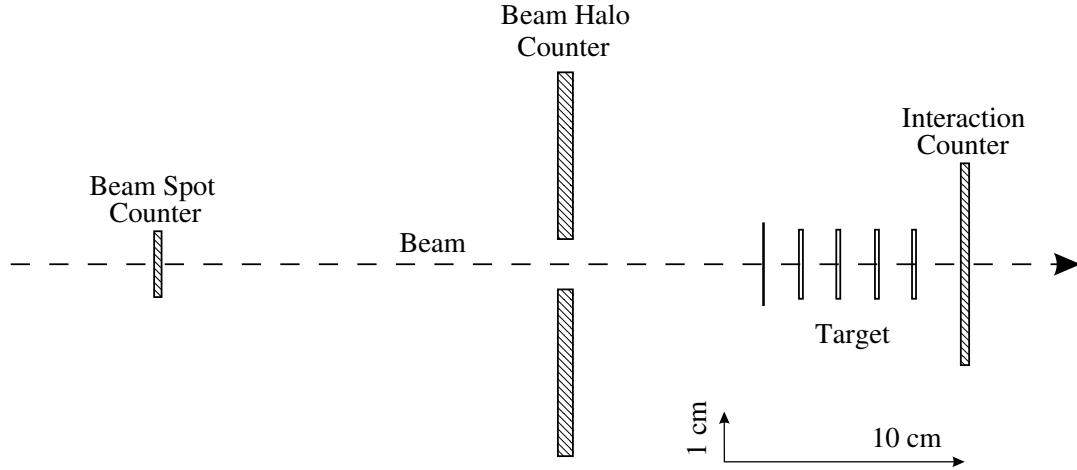
Figure 4.1: Scale drawing of pretrigger scintillator paddles and target foils.
