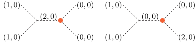
Figure 7.17: L2 scenario - loop level processes. Here we show only schematically the contribution modes, t-channel diagrams also contribute. The loop level vertices are shown in red.
