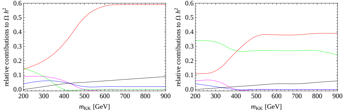
Figure 7.19: Relative contributions of the partial annihilation cross sections to the relic abundance in L2 scenario when all the coannihilation channels are open. On the left panel we see the dominant contribution of l_{D/S}^{(1)} A^{(1)} \rightarrow l A^{(2)} in red. Other channel are l_D^{(1)} \nu^1 \rightarrow q\bar{q} co-annihilation in green, l_D^{(1)} \nu^1 \rightarrow A H^{(2)} in magenta, q^{(1)} A^{(1)} \rightarrow q A^{(2)} in blue and b_D^{(1)} W^{(1)} \rightarrow b, W^{(2)} in black. On the right panel the same colors are applied for the contributions when we include the loop couplings. We see the importance of the W^{(2)} resonance in the l_D^{(1)} \nu^{(1)} \rightarrow q\bar{q} processes when the loop couplings are turned on.
