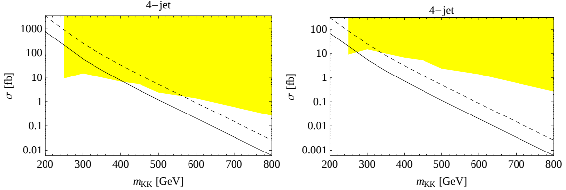
Figure 8.14: Bounds from study of di-jet resonances. We plot the total effective cross section of 4-jet events assuming the efficiency of 3% (solid black) and 13% (dashed black). CMS bounds (7) are indicated in yellow. On the left: non degenerate geometry is assumed R_4 \gg R_5 and On the right: degenerate radii R_4 = R_5 . Thanks to G. Cacciapaglia.
