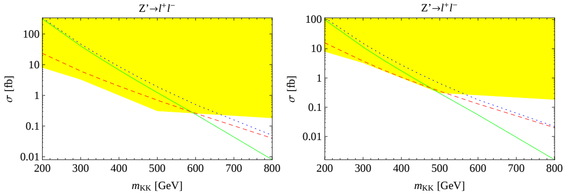
Figure 8.13: Bounds from the study of Z' \rightarrow l^+ l^- . Total effective cross section (black), cross section from pair production (blue), cross section from single production (red). ATLAS bounds (6) are indicated in yellow. On the left: non degenerate geometry is assumed R_4 \gg R_5 and On the right: degenerate radii R_4 = R_5 . Thanks to G. Cacciapaglia.
