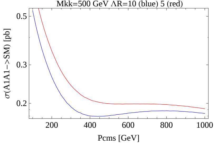
Figure 7.24: Total annihilation cross section A^{(1)}A^{(1)} \rightarrow SM as a function of p_{cms} for M_{KK} = 500 GeV and \Delta R = 5, 10 in red and blue respectively.
