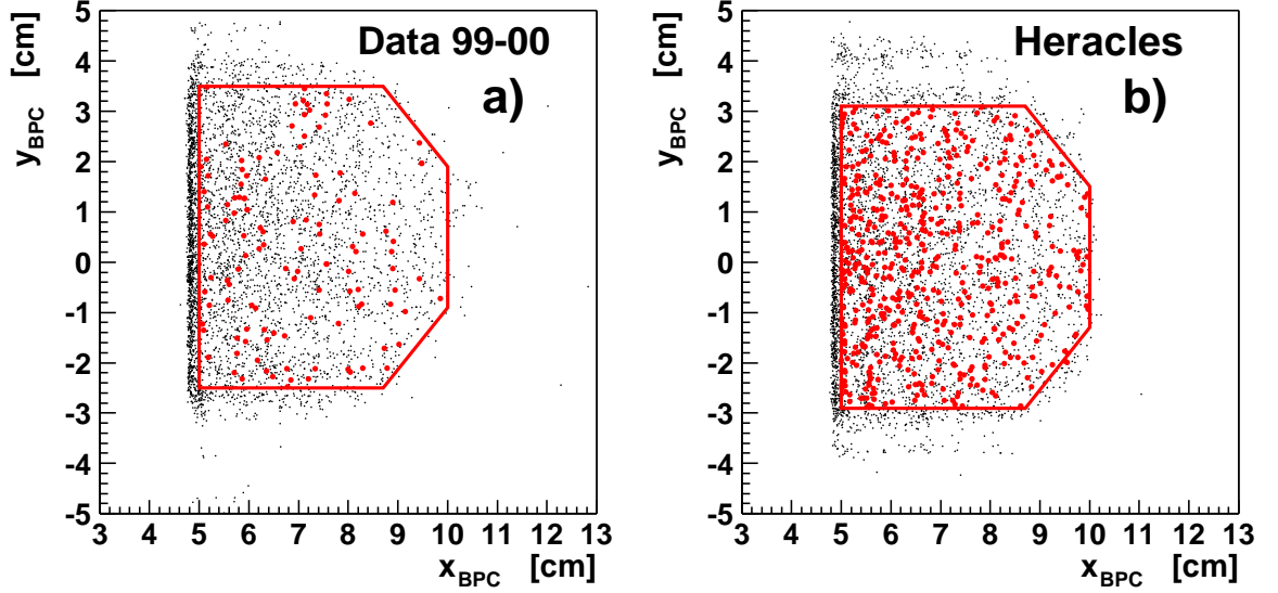
Figure 3.4: Electron impact positions in the BPC a) for the data and b) the signal Monte Carlo. The small dots are from events triggered with HFL 06 and with E_{BPC} > 10 \text{ GeV} . Here, the shift in y_{BPC} of 4 mm between data and Monte Carlo can be clearly seen. The bigger dots are the events passing the selection cuts. Thus, they fall into the fiducial areas, which are indicated as well.
