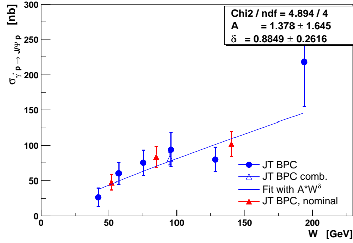
Figure 4.16: Cross section vs. W for the analysis twice the number of bins (statistical errors only) and a fit to these points. For comparison, the nominal cross sections are shown.
