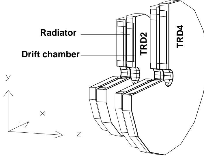
Figure 2.12: Layout of the four TRD modules.
