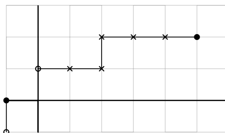
Figure 6. The structure of zeros and poles of the generating function \psi(u) for the fundamental representation in direction h_3 of Y_{5,2,0}[\Psi] . We draw one example of the snake configuration.
