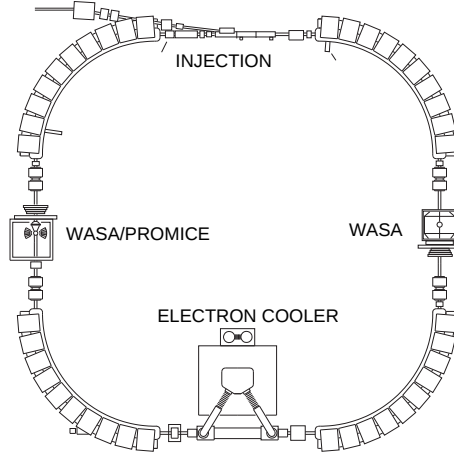
Fig. 4. The CELSIUS ring.
