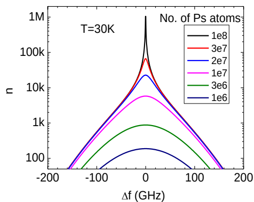
Figure 2. Calculated Doppler distribution of the Ps Lyman- \alpha line at 243 nm for a 2D polarized Ps gas in a 10 \mu\text{m}^2 planar cavity approximating 2D Ps on the surface of quartz. The transition to a 2D BEC (i.e. significant departure from a Maxwell-Boltzmann momentum distribution) is signalled by the appearance of positive curvature in the log of the momentum density.
