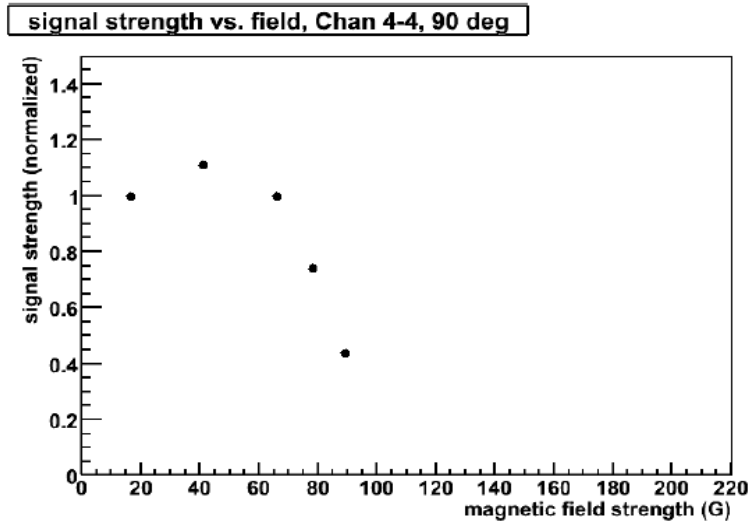
Figure 4.1: Burle 85011-501 MCP–MAPMT output vs. magnetic field strength at 90° between device axis and the field.
