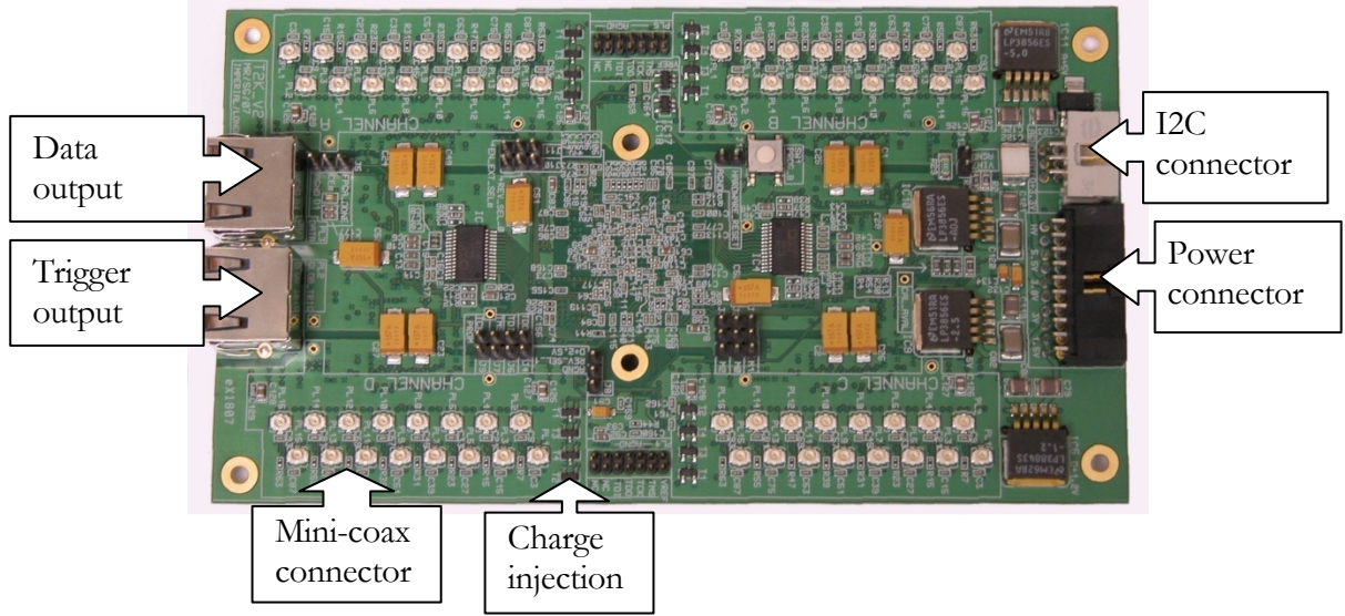
Figure 5.2: TFB Board, top view.
