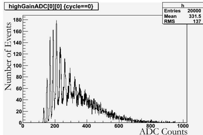
Figure 4.31: ADC spectrum of MPPC PE output.
