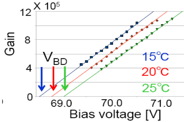
Figure 4.37: MPPC gain vs. biasing voltage and temperature.
