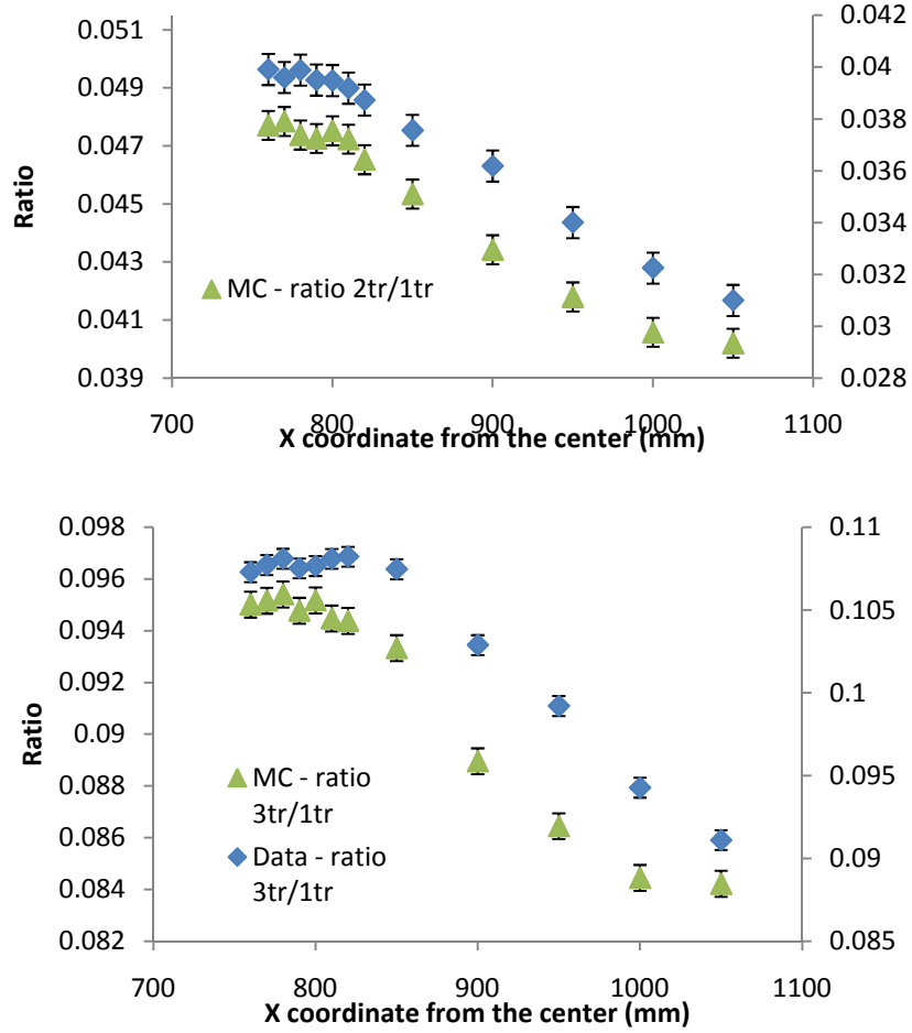
Figure 6.6: Two-track to single-track events (top) and three-track to single track events (bottom) ratio vs. X coordinate.
