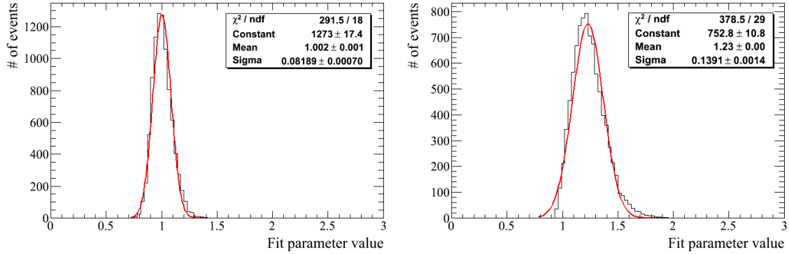
Figure 8.5: Distributions of the CCCQE (left) and CCC1\pi^+ (right) fit coefficients for different random scale triplets.
