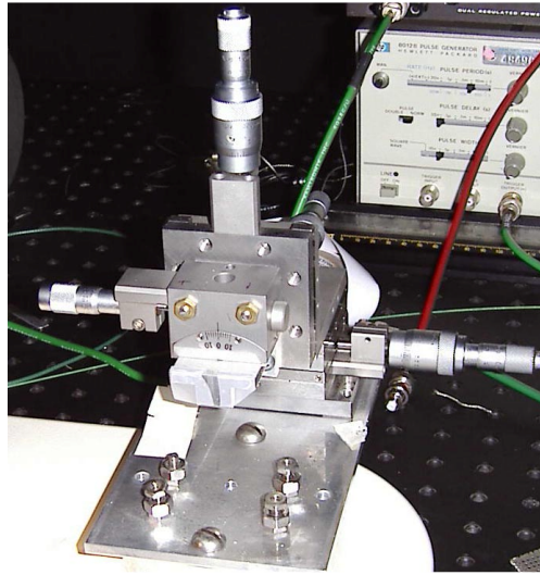
Figure 4.25: 462 series XYZ-M stage.
