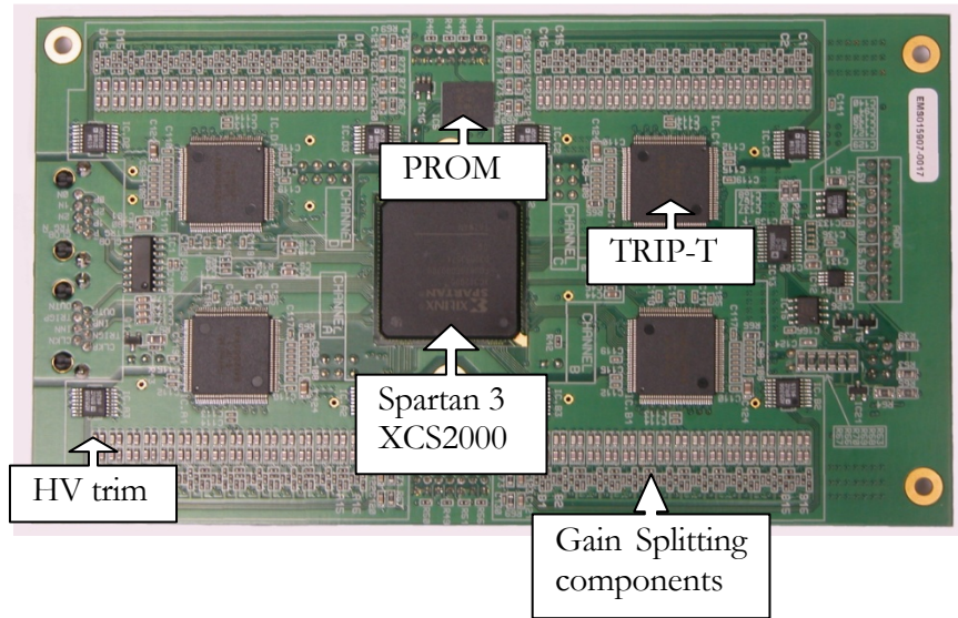
Figure 5.3: TFB Board, bottom view.
