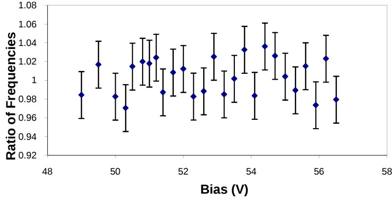
Figure 4.7: Ratio of dark noise rate at different biases of before to after irradiation.
