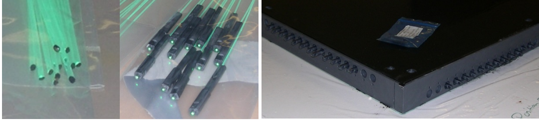
Figure 5.13: WLS fiber ends cleaver at 45o and blackened (left); WLS fiber glued and polished with ferrules (middle); PØDule with inserted WLS fibers and MPPC sensors on top (right).
