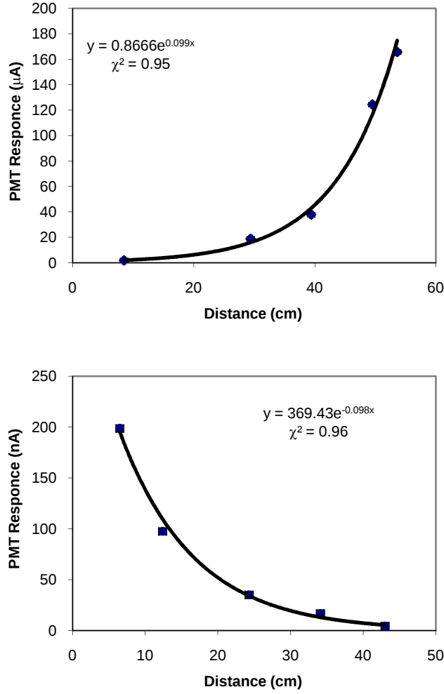
Figure 3.4: PMT response to UV LED position (top) and radioactive source position (bottom) along the bulk triangular shape scintillator without WLS fiber.
