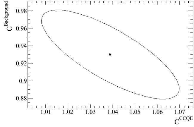
Figure 7.8: The 1\text{-}\sigma contour plot for the single light track sample 2-parameter fit.
