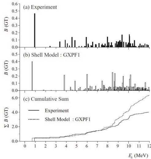
Fig. 3. Comparison of B(\text{GT}) strength distributions from the ^{54}\text{Fe}(^3\text{He}, t)^{54}\text{Co} measurement and a shell model (SM) calculation. (a) The experimental B(\text{GT}) distribution. (b) The B(\text{GT}) distribution obtained in the SM calculation using the GXPF1 interaction. (c) Cumulative sums of B(\text{GT}) values from the experiment and the SM calculation.
