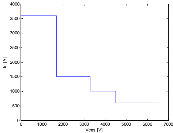
Figure 3: Voltage and current ratings range of commercially available high voltage IGBT modules.
