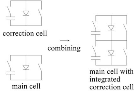
Figure 2: Schematic representation of the proposed droop correction concept. Both cells consist of an energy storage capacitor, a charge switch (right switch), a discharge switch (left switch) and a bypass diode.
