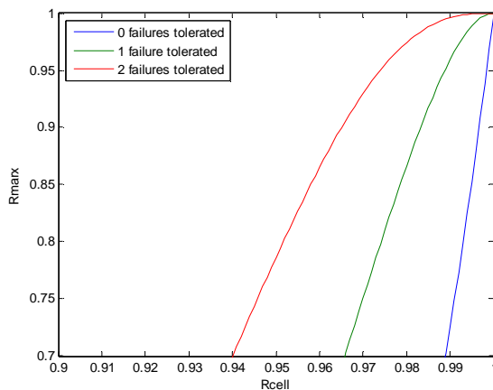
Figure 5: Reliability of a 32-cell Marx modulator versus the reliability of one basic Marx cell PEBB.
