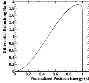
Fig. 1: Positron energy spectrum of Michel decay as a function of normalized positron energy x = 2E_e/m_\mu . Positron background yield around the signal energy ( x \approx 1 ) is abundant
