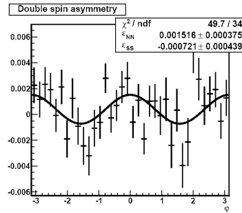
Fig. 7: STAR Preliminary results on raw double spin asymmetry
