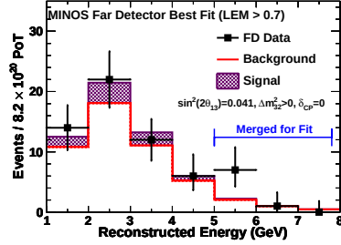
Fig. 4: Reconstructed neutrino energy spectrum for the \nu_e -CC candidate events in the Far Detector. The black points represent the data. The histogram shows the expected background (unfilled area) and the contribution of \nu_\mu \rightarrow \nu_e signal (filled area) for the best-fit value of \sin^2(2\theta_{13}) = 0.041
