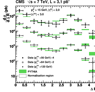
Fig. 6: Differential B\bar{B} production cross sections as a function of \Delta R for the three leading jet p_T regions
