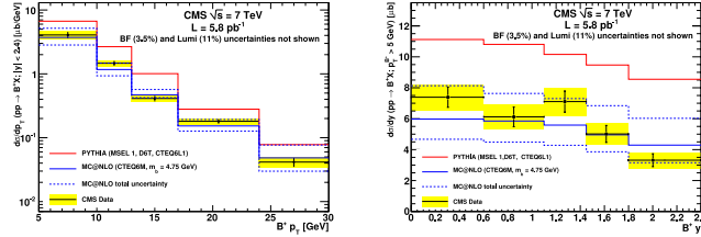
Fig. 2: B^\pm production cross section as a function of B p_T (left) and rapidity (right)
