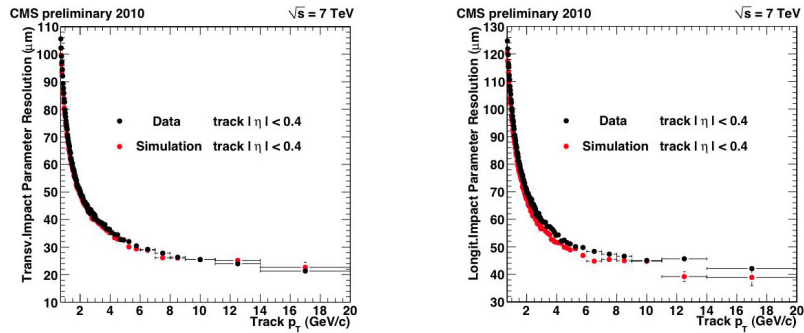
Fig. 8: Measured resolution of the track transverse (left) and longitudinal (right) impact parameter as a function of the track p_T . Only central tracks with |\eta| < 0.4 are considered. Black and red symbols correspond to results from data and simulation, respectively
