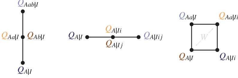
Figure 7.3. The two bosonic and the fermionic type of QQ-relations of equation 7.7 relate the Q-functions at the respective nodes according to \mathcal{Q}\mathcal{Q} = \mathcal{Q}^+ \mathcal{Q}^- - \mathcal{Q}^- \mathcal{Q}^+ .
