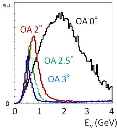
Fig. 1. Neutrino energy spectra at SK at different off-axis angles, 3^\circ , 2.5^\circ , 2^\circ and on-axis.
