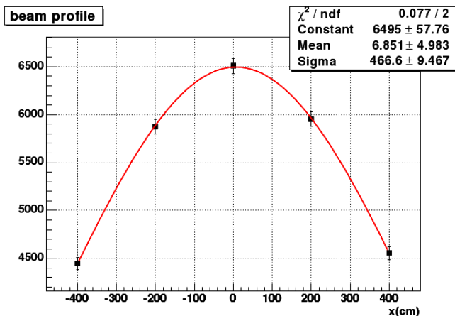
Fig. 4. Neutrino beam profile measured with the INGRID detector (Monte Carlo simulation) [25].
