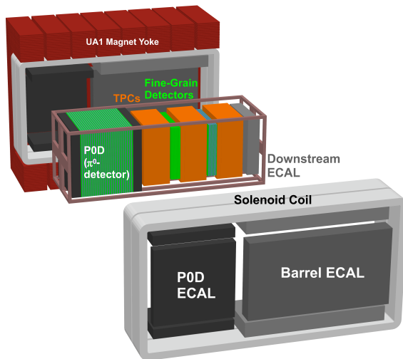
Fig. 3. The off-axis near detector system shown with one side of the UA1 magnet. The inner detectors are supported by a basket and consist of the P0D upstream, followed by the Tracker , and the downstream ECAL. They are surrounded by the side ECALs. The slits of the yokes are equipped with SMRD counters.
