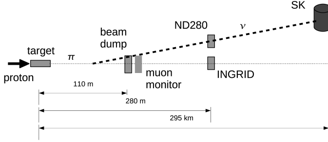
Fig. 2. Layout of T2K neutrino beam and detectors.
