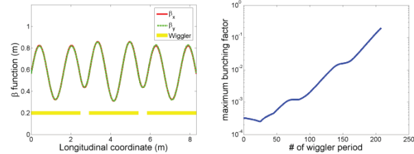
Figure 4: Location of three-section wigglers and \beta function evolution with minimum overall variation (left) and evolution of bunching factor amplitude of shot noise (right) in FEL amplifier.
