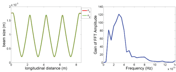
Figure 8: Evolution of transverse beam size (left) and spectrum of gain of density modulation (right) in a four-cell plasma cascade amplifier.
