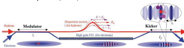
Figure 1: Layout of coherent electron cooler with a high gain free electron laser amplifier.
