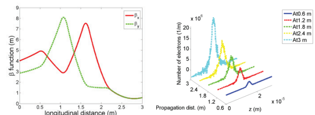
Figure 3: Evolution of electron beam \beta function (left) and longitudinal density modulation (right) in modulator.
