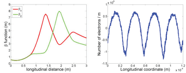
Figure 6: Evolution of electron beam \beta function (left) and amplified longitudinal density modulation (right) in kicker.
