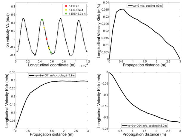
Figure 7: Coherent longitudinal velocity kick to ions with various energy spread (top left), a single ion with reference energy (top right), a single ion with lower energy of energy spread 3e-4 (bottom left) and a single ion with higher energy of energy spread 3e-4 (bottom right) in kicker.
