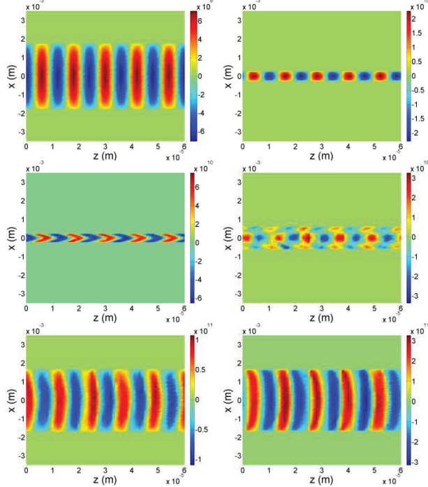
Figure 9: 2-D density modulation in the electron beam at the entrance of PCA (top left), at the waist in first cell (top right), slightly before the waist of second cell (middle left), slightly after the waist of second cell (middle right), end of third cell (bottom left) and exit of fourth cell (bottom right). X-axis is along the horizontal direction and z-axis is along the longitudinal direction.
