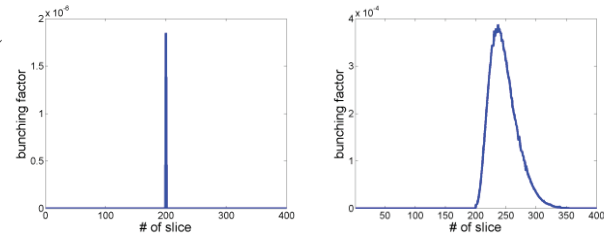
Figure 5: Bunching factor amplitude of modulation signal at the entrance (left) and exit (right) of FEL amplifier.
