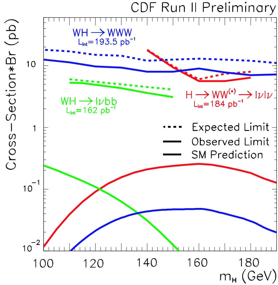
Figure 7.3: CDF Run II preliminary cross section limit for the Standard Model Higgs boson.
