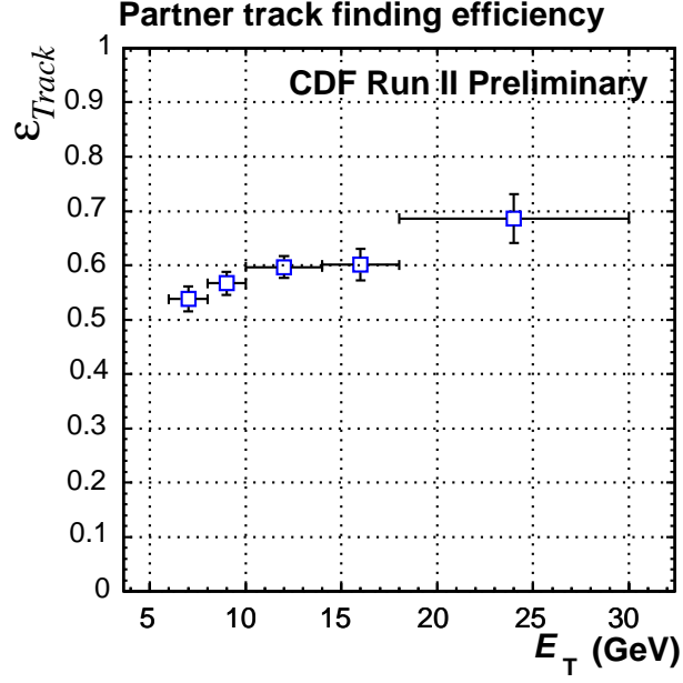
Figure 4.18: The conversion electron E_T dependence of the partner track finding efficiency. We have normalized the Monte Carlo distribution to data in the region of the partner track p_T above 2 GeV/ c .
