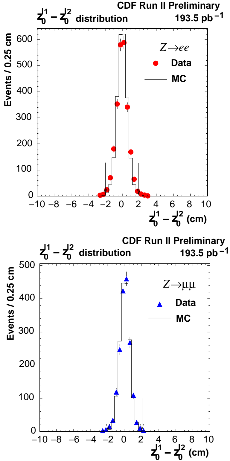
Figure 6.12: |z_0^{l1} - z_0^{l2}| distributions of Z \rightarrow \ell\ell events.
