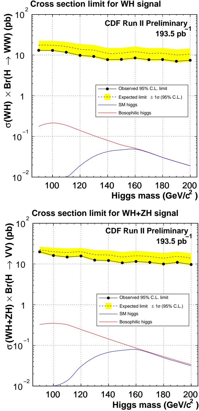
Figure 7.2: Upper (Lower) plot shows 95% C.L. upper limits on the production cross section times branching fraction as a function of Higgs boson mass for the WH ( WH + ZH ) production, together with the cross sections of the Standard Model and of the benchmark scenario for the bosophilic Higgs boson. Results from pseudo-experiments for expected limits are also shown.
