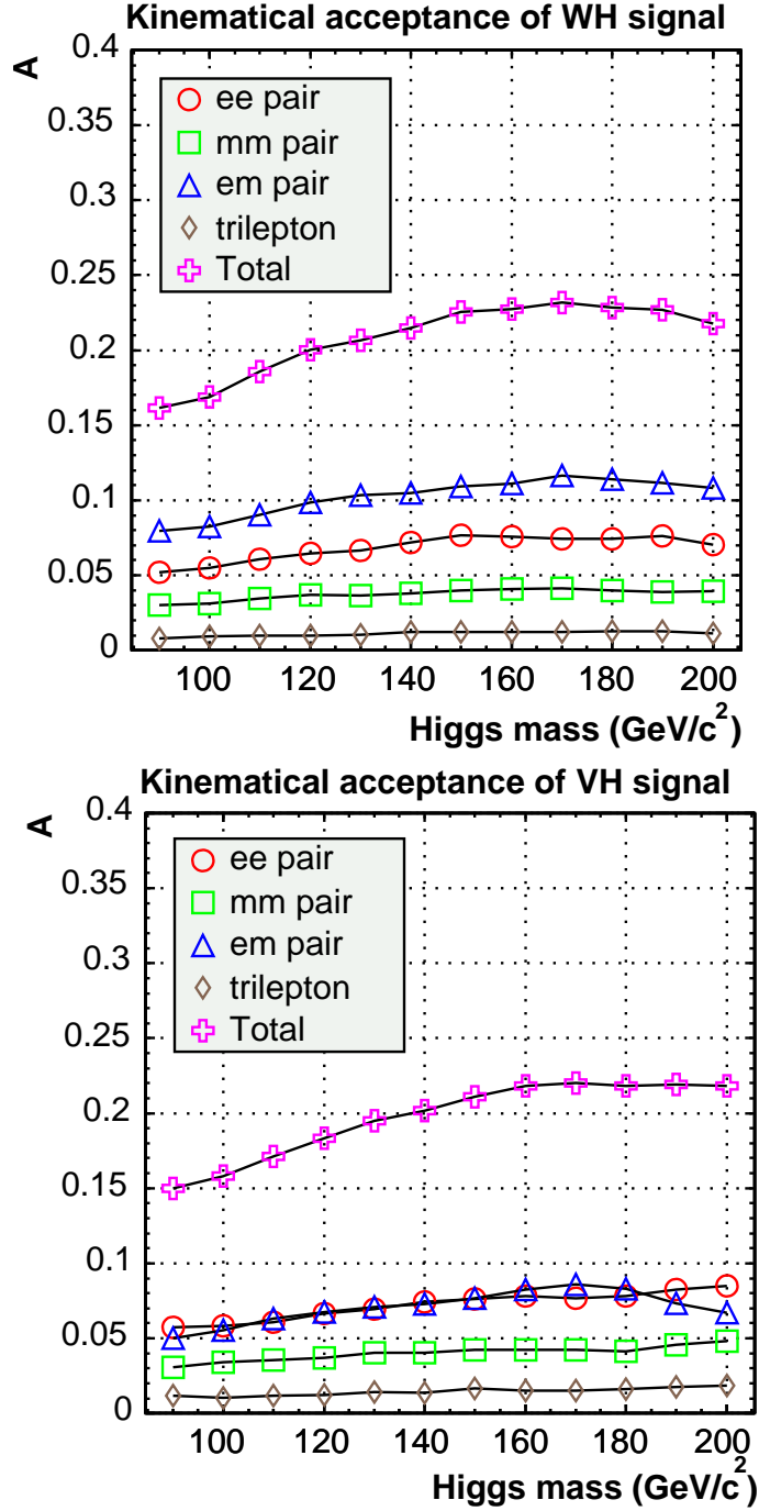
Figure 6.4: Upper (Lower) plot shows geometrical and kinematical cut efficiency for each dilepton type for the WH \rightarrow WW^*W^* \rightarrow \text{dilepton} ( WH + ZH \rightarrow VV^*V^* \rightarrow \text{dilepton} ) signal Monte Carlo samples. Circles, squares, triangles, and diamonds correspond to the dielectron channel, dimuon channel, e\mu channel, and trilepton channel respectively.
