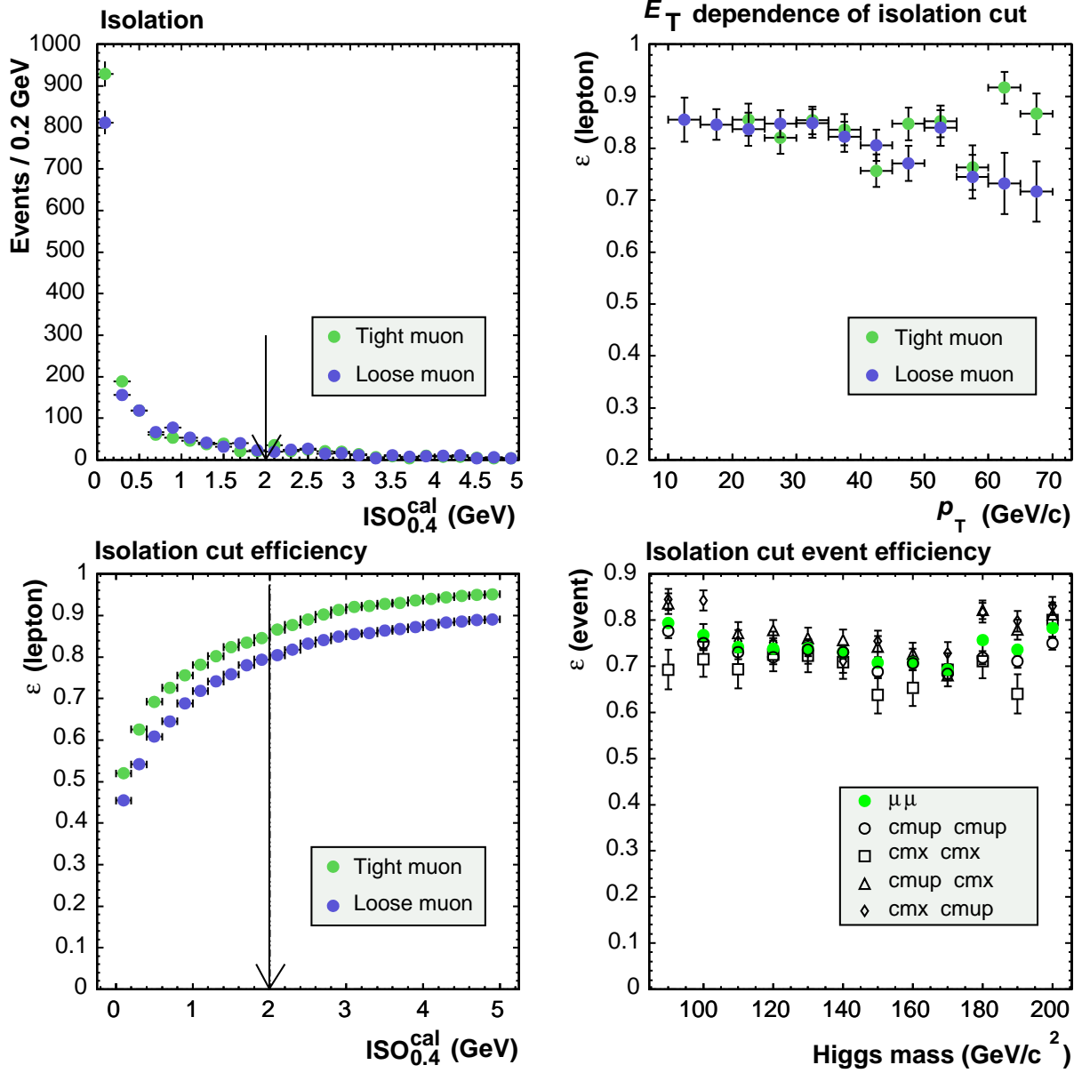
Figure 6.8: The lepton-isolation features of signal Monte Carlo sample. The Higgs boson mass is 160 GeV/c 2 and the event type is dimuon. Upper left plot is raw ISO_{0.4}^{cal} distribution, upper right plot is E_T dependence of isolation cut efficiency, lower left plot is the isolation cut efficiency as a function of the cut value, and lower right is the cut efficiency as a function of the Higgs boson mass.
