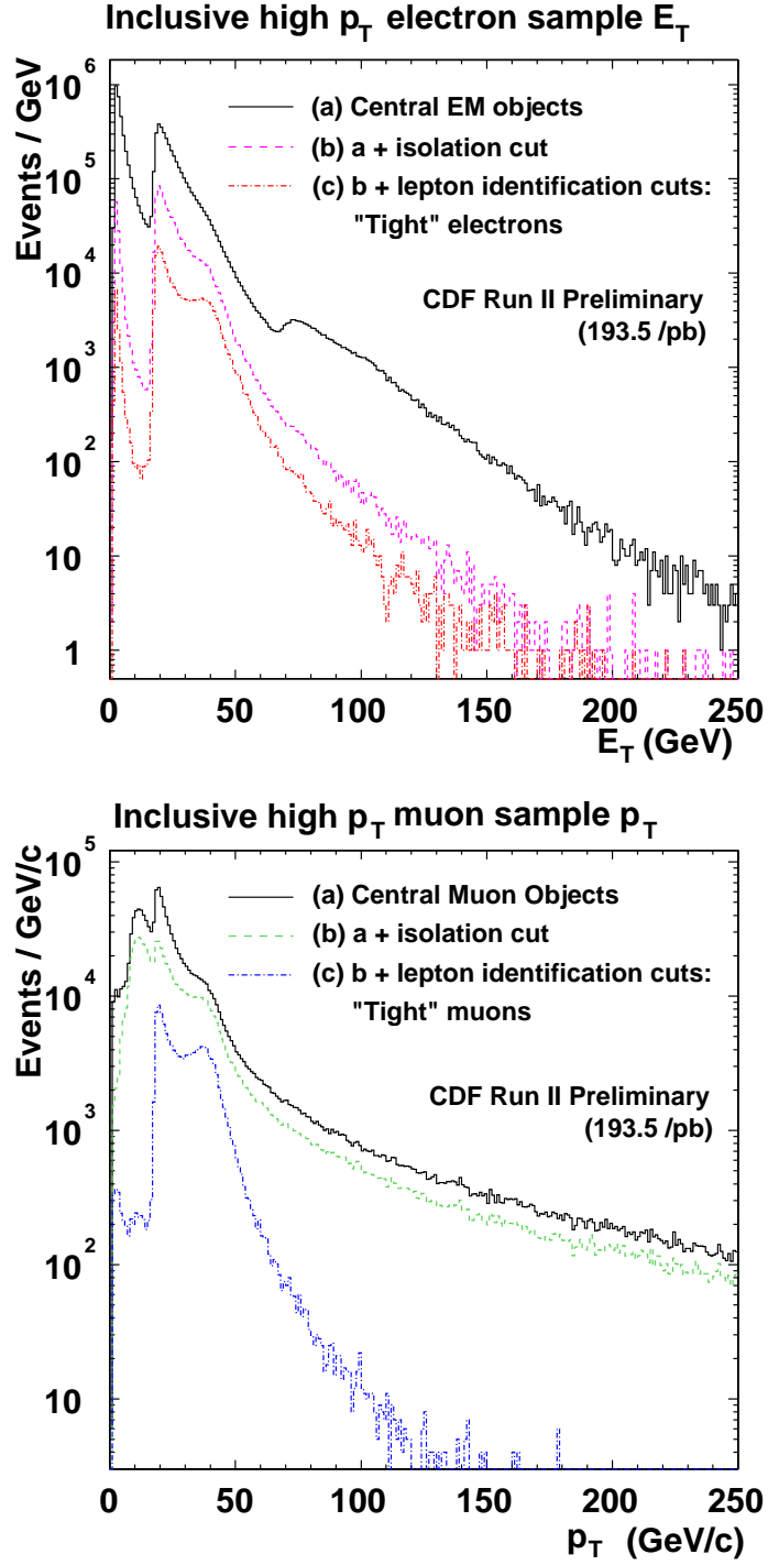
Figure 3.15: Upper distributions are transverse energy for all electrons in the inclusive high p_T electron sample. Lower distributions are transverse momentum for all muons in the inclusive high p_T muon sample.
