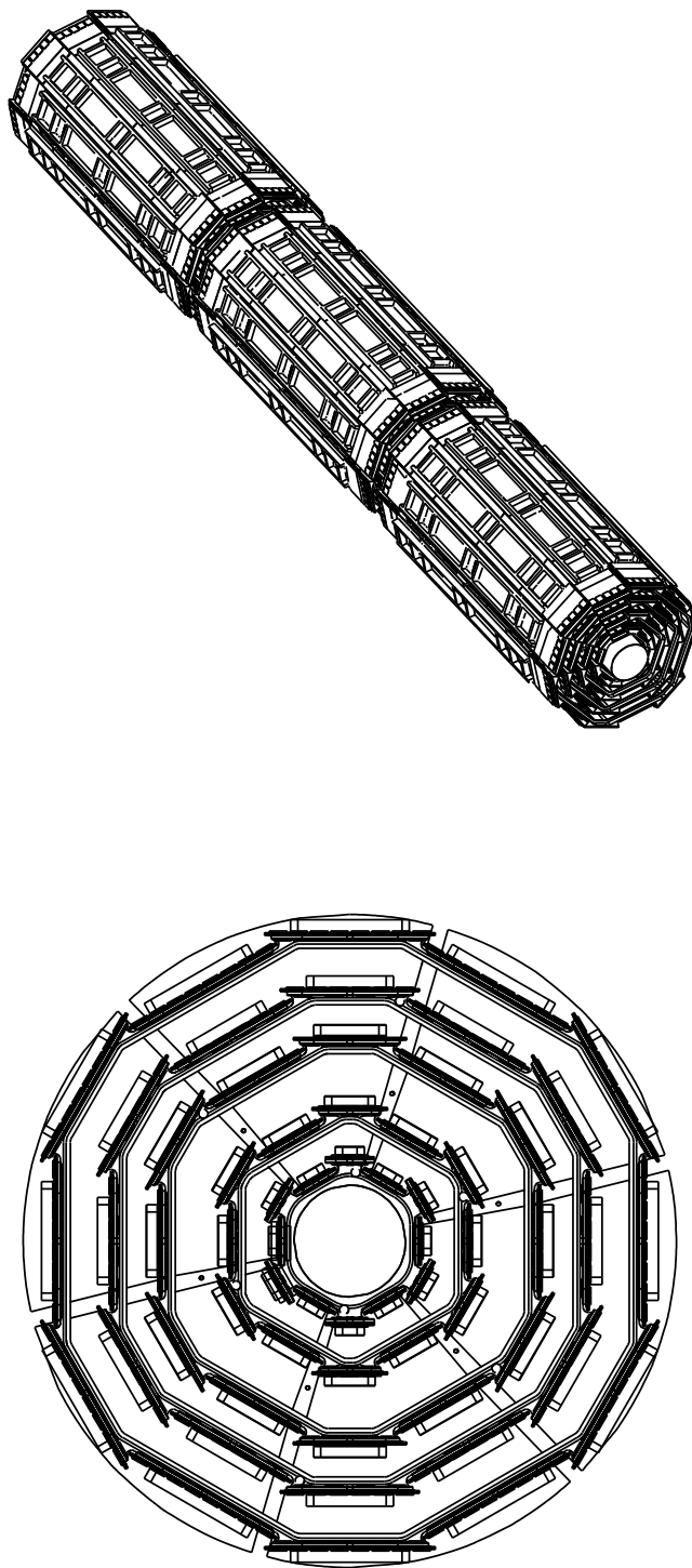
Figure 2.7: Upper figure is a view of the three barrels of SVX II silicon detector. Lower one is a view of one barrel. One barrel has 12 wedges and 5 layers.
