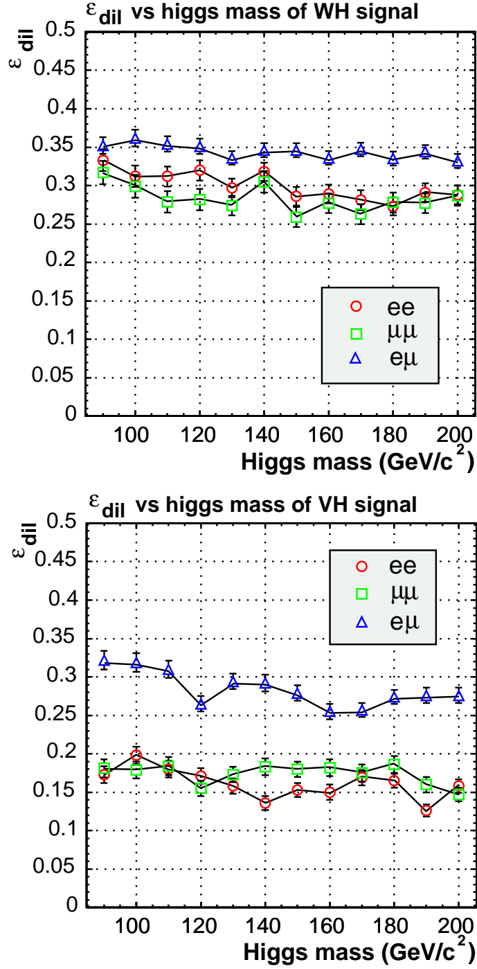
Figure 6.13: Upper (Lower) plot is dilepton selection cuts efficiencies as a function of the Higgs boson mass for WH ( WH + ZH ) production. The circle point is dielectron channel, square one is dimuon channel, and triangle one is e\mu channel
