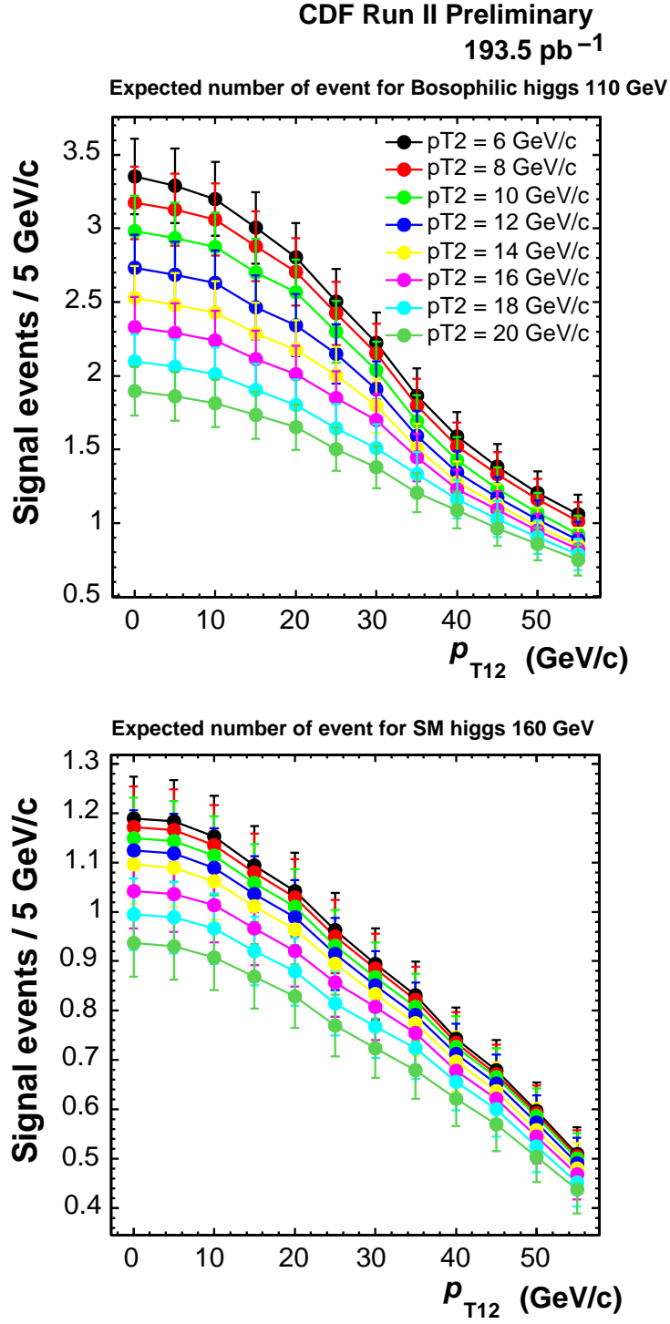
Figure 5.3: Upper (Lower) plot shows the number of expected signal events as a function of p_{T12} cut value for the 110 GeV/ c^2 bosophilic Higgs (160 GeV/ c^2 SM Higgs).
