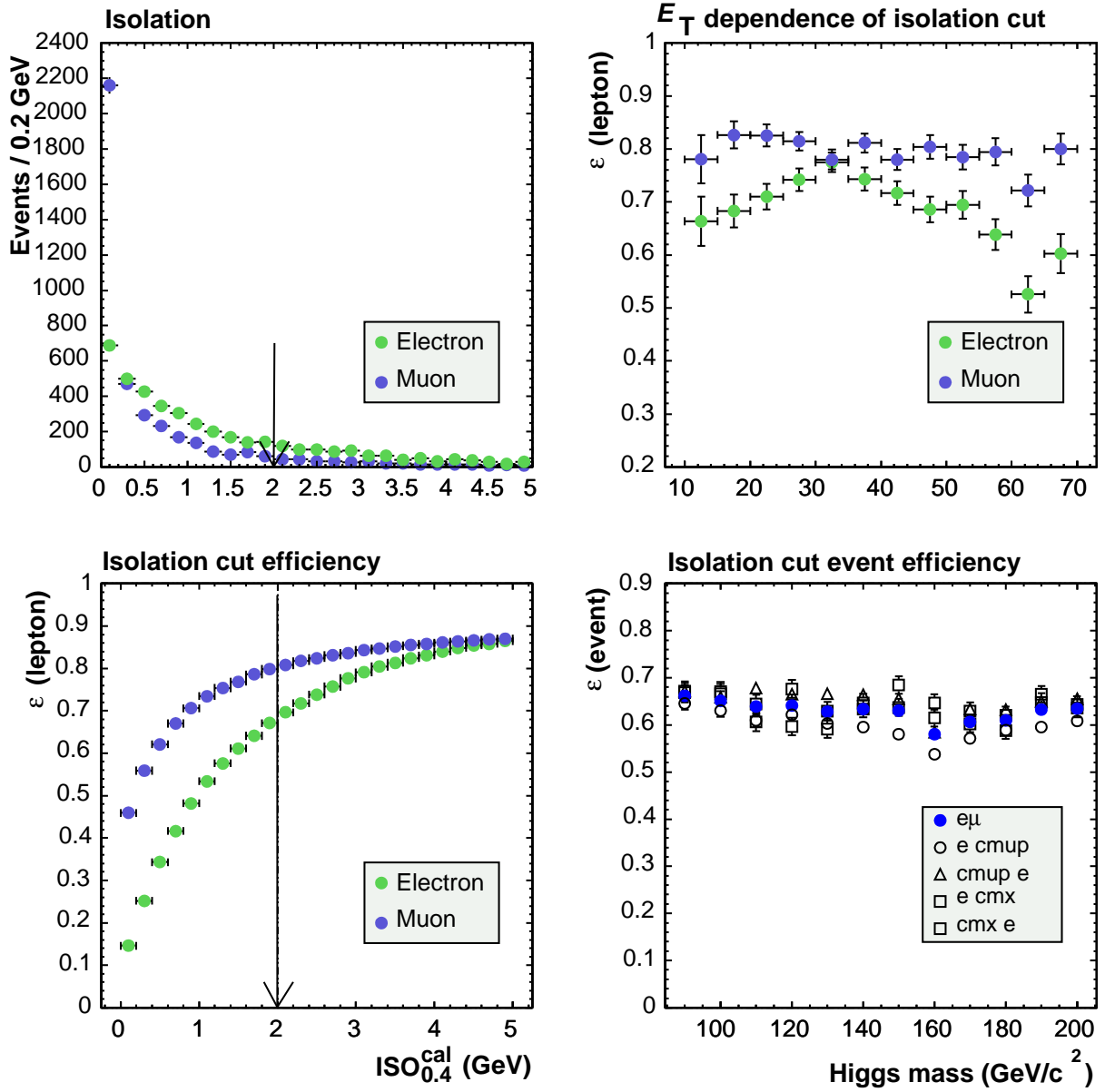
Figure 6.9: The lepton-isolation features of signal Monte Carlo sample. The Higgs boson mass is 160\text{ GeV}/c^2 and the event type is e\mu . Upper left plot is raw ISO_{0.4}^{cal} distribution, upper right plot is E_T dependence of isolation cut efficiency, lower left plot is the isolation cut efficiency as a function of the cut value, and lower right is the cut efficiency as a function of the Higgs boson mass.
