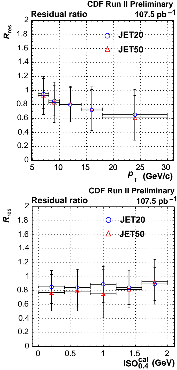
Figure 4.26: The conversion electron p_T and ISO_{0.4}^{\text{cal}} dependence of the residual conversion ratio for the JET20 and JET50 samples.
