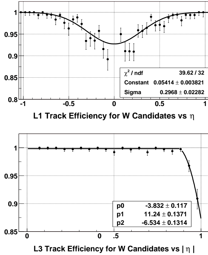
Figure 6.15: Level-1 (top) and Level-3 (bottom) tracking efficiencies as a function of \eta measured by CES.
