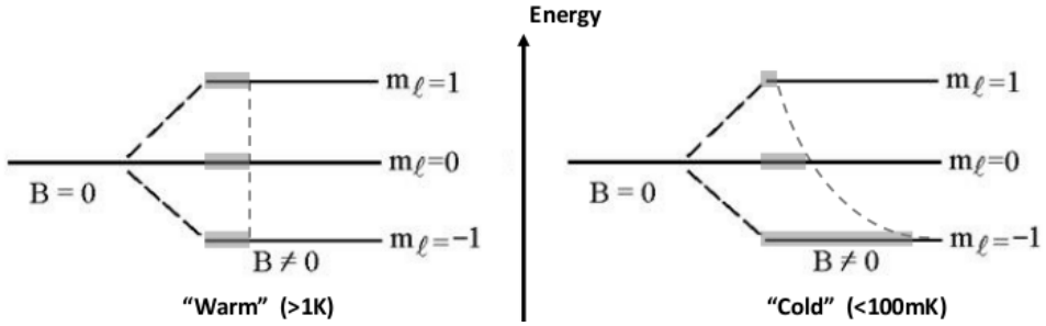
Fig. 1. Population evolution following a Boltzmann distribution for the case I = 1 . On the left-hand side, the nucleus is non-oriented (warm), and on the right-hand side, the nucleus is oriented (cold).
