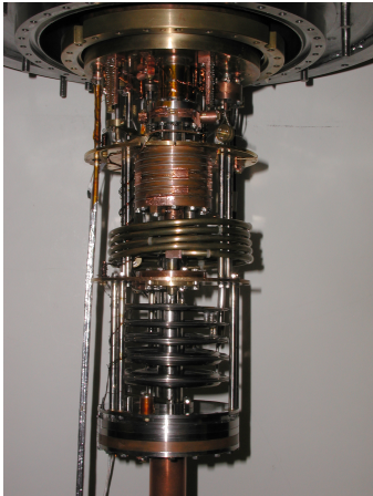
(a) The dilution unit
