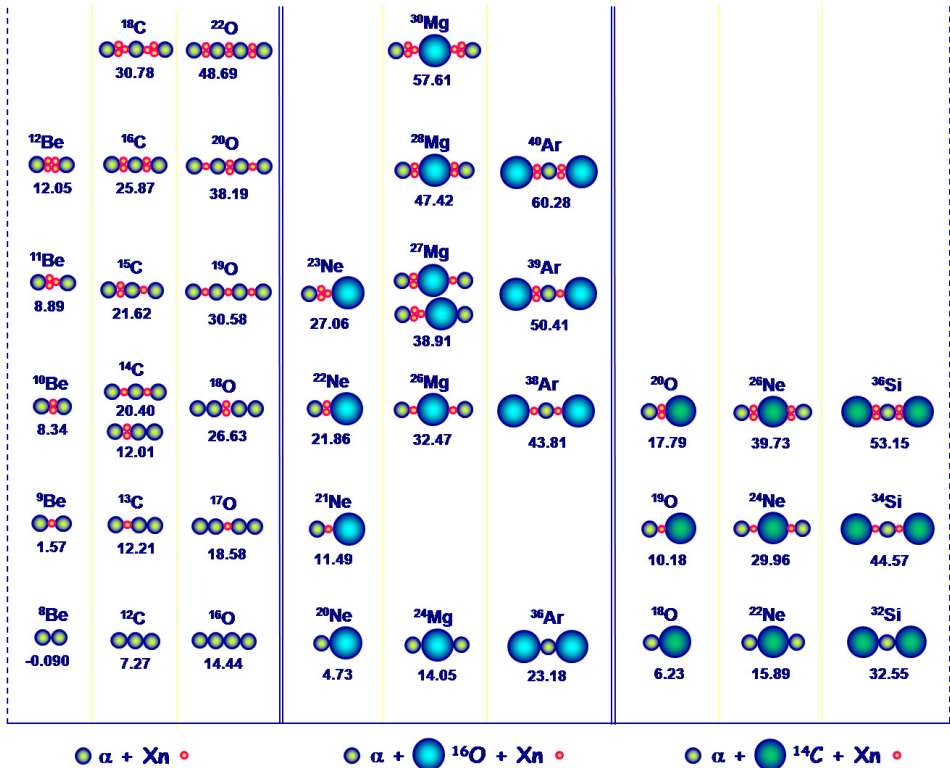
Fig. 1. (Color online) Schematic illustration of the structures of molecular shape isomers in light neutron-rich isotopes of nuclei consisting of \alpha -particles, {}^{16}\text{O} - and {}^{14}\text{C} -clusters plus some covalently bound neutrons ( Xn means X neutrons). The so-called “Extended Ikeda-Diagram” [8] with \alpha -particles (left panel) and {}^{16}\text{O} -cores (middle panel) can be generalized to {}^{14}\text{C} -clusters cores (right panel). Threshold energies (in MeV) are given for the relevant decompositions.
