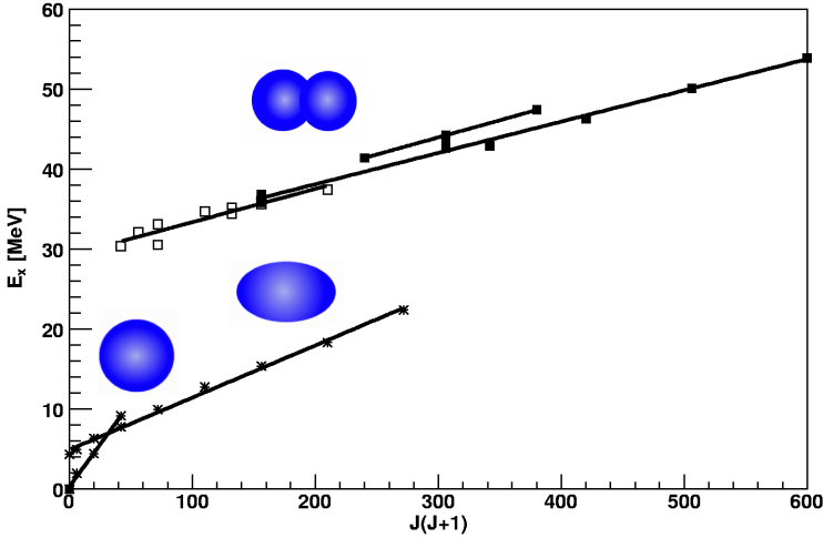
Fig. 2. Rotational bands and deformed shapes in ^{36}\text{Ar} . Excitation energies of the g.s. (spherical shape) and SD bands [20] (ellipsoidal shape), respectively, and the energies of HD band from the quasimolecular resonances observed in the ^{12}\text{C} + ^{24}\text{Mg} (open rectangles) [21, 34, 35, 36] and ^{16}\text{O} + ^{20}\text{Ne} (full rectangles) [37, 38] reactions (dinuclear shape) are plotted as a function of J(J+1) . This figure has been adapted from Refs. [19, 21].
