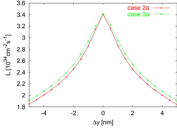
Figure 3: The luminosity as a function of the offset. Case 2a corresponds to the previous plot. In case 3a more slices and macro particles were used in the beam-beam simulation and larger misalignments were applied in the main linac.
