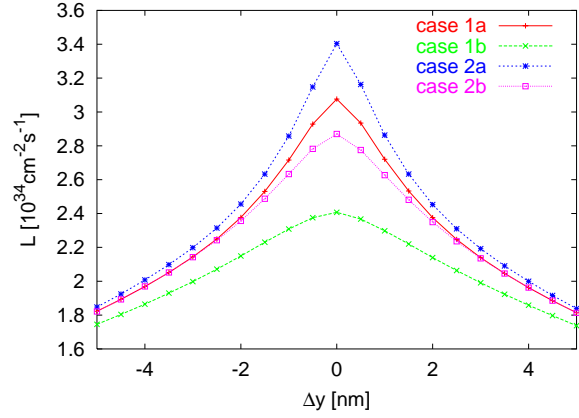
Figure 2: The luminosity as a function of the offset for different cases, see text.
