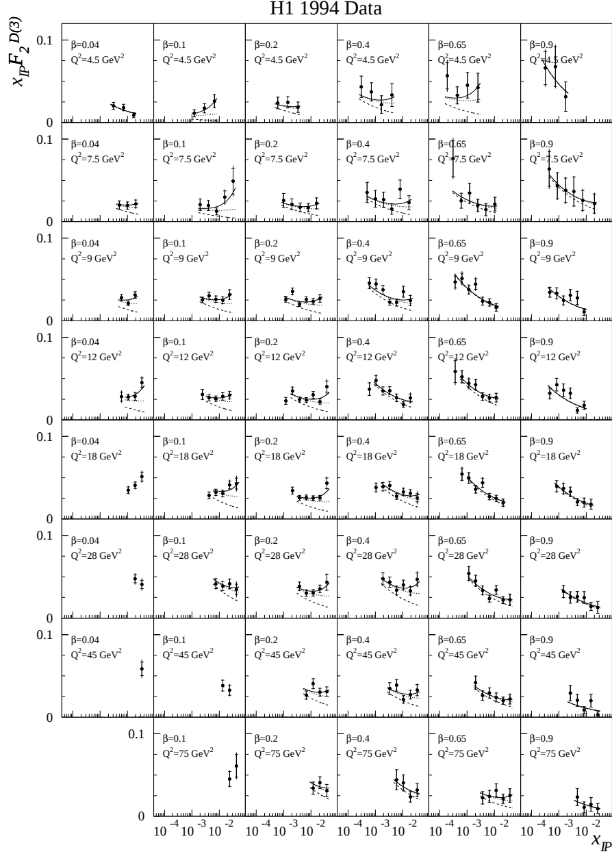
Fig. 16. The differential structure function x_{\mathbb{P}} F_2^{D(3)} as a function of x_{\mathbb{P}} for various \beta and Q^2 values. The solid curves show the results from the two-component Regge fit. The dashed curves show the pomeron contribution alone. From H1.
