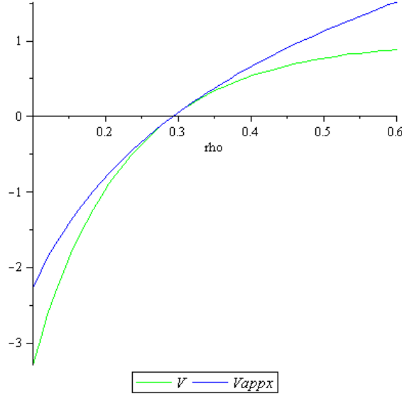
Figure 4.8: Comparison of V (from (4.40)) and V_{appx} (from (4.56)) near the zero for the Sanchez solution for x_3 = 0.5 and \rho := \rho_2
