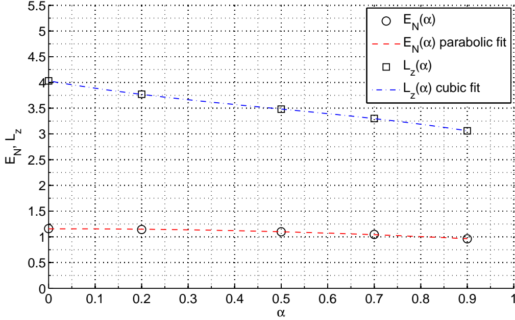
Figure 6.3: Plot of minimal normalized energies E_N and optimal periods L_z vs. \alpha for V+AV configuration.
