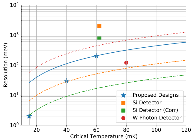
FIG. 3. Energy resolution scaled according to Eq. (12) using the parameters in Table III. These are shown along with the scaling relations for the given volume and efficiency as a function of T_c (solid line for design A, dashed for design B, and dot-dashed for design C). Also shown are the resolution demonstrated in a tungsten TES photon detector [61] and a Si detector with tungsten QET readout [66]. The corrected resolution of the Si detector for upgraded readout electronics is also shown, compared to its ideal scaling relation (dotted red line).
