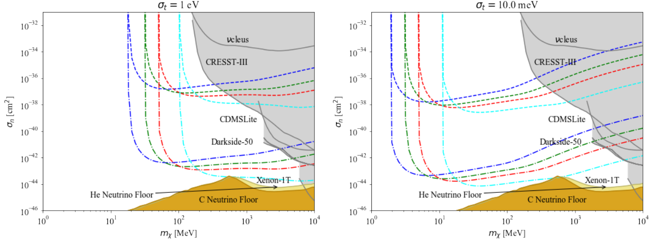
FIG. 8. Nuclear recoil projected reach at 95% C.L. for He (blue), Diamond (green), Si (red), and Xe (cyan) for energy thresholds of 1 eV ( left panel ) and 10 meV ( right panel ). The dashed lines are for a g-day exposure, while the dot-dashed lines are for a kg-year exposure. The yellow region indicates the neutrino floor for He [15], and the brown region the neutrino floor for C (computed according to the formalism in Ref. [77]). Also shown in grey are the current best limits on NR dark matter interactions from \nu CLEUS [91], CRESST-III [35, 92], CDMSlite [93], Darkside-50 [94], and Xenon-1T [95] for comparison.
