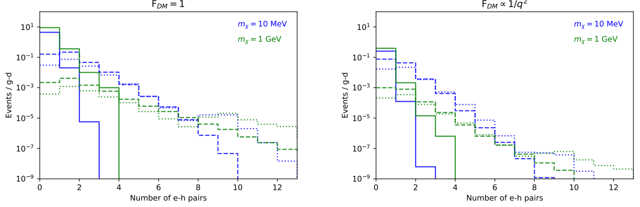
FIG. 6. Recoil spectra for \bar{\sigma}_e = 10^{-37} \text{ cm}^2 of silicon (dashed), germanium (dotted) and diamond (solid) for m_\chi = 10 \text{ MeV} (blue) and 1 \text{ GeV} (green) respectively.
