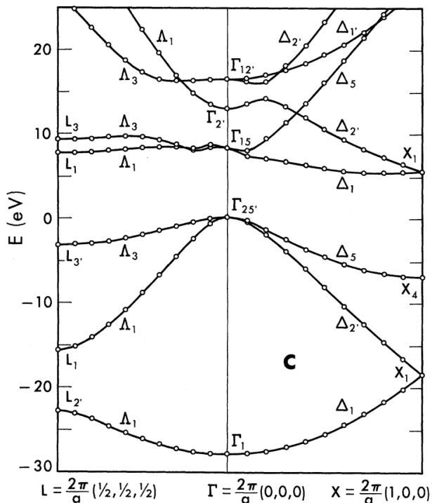
FIG. 1. Band structure of diamond in the reduced-zone scheme, reproduced from Ref. [16].
