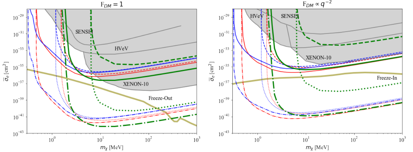
FIG. 7. Projected reach at 95% C.L. for electron recoils in silicon (red), germanium (blue) and diamond (green) detectors with 1 g-day of exposure and 1 e-h pair threshold (solid), 1 g-day of exposure and 2 e-h pair threshold (dashed), 1 kg-year of exposure and 1 e-h pair threshold (dot-dashed), and 1 kg-year of exposure and 2 e-h pair threshold (dotted). The current exclusion limits from SENSEI [71], CDMS HVeV [70], and XENON10 [2] are also depicted for comparison. The parameter space corresponding to producing the observed dark matter relic density via standard freeze-out in a minimal dark sector model is indicated by the solid thick mustard curve labeled ‘Freeze-Out’ (see Ref. [90] for more details).
