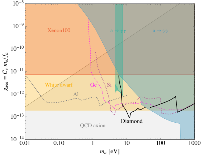
FIG. 5. Projected reach at 95% C.L. for absorption of axion-like particles. The reach of a kg-year exposure of diamond is shown by the solid black curve. The reach for semiconductors such as germanium and silicon [45] and superconducting aluminium [9] targets is depicted by the dotted magenta, purple and gray curves, respectively. Stellar constraints from Xenon100 data [84] and white dwarfs [85] are indicated by the shaded red and orange regions, respectively. Constraints from loop-induced couplings to photons are presented in the shaded blue regions [86, 87]. The QCD axion region of interest is indicated in shaded gray.
