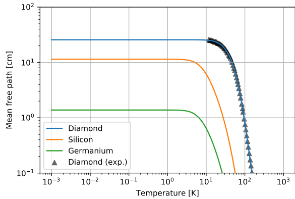
FIG. 2. Estimated mean free path using the Callaway model fitted to experimental data [52, 53] and normalized to the same geometry ( l_b = 2.6 mm) and surface quality ( P = 4 \times 10^{-4} ). The model is described in Ref. [52], with the modification that the specular reflection probability P is a constant rather than a function of phonon frequency.
