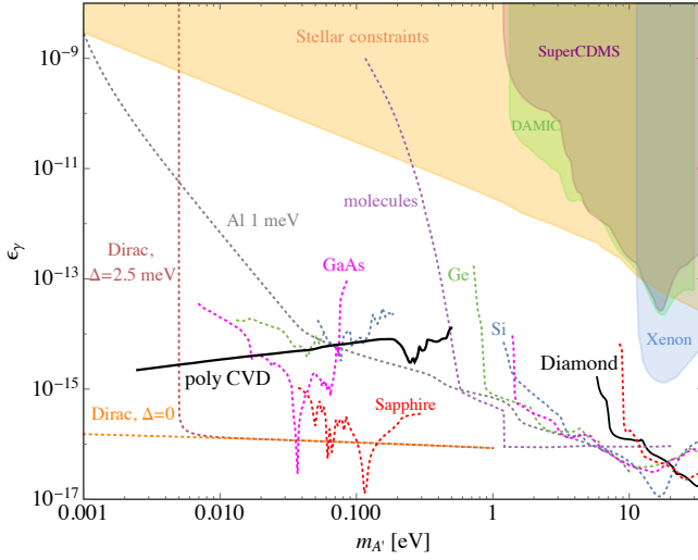
FIG. 4. Projected reach at 95% C.L. for absorption of kinetically mixed dark photons with mass > 1 meV. The solid black curves indicate the expected reach for a kg-year exposure of diamond. Projected reach for germanium and silicon [45], Dirac materials [10], polar crystals [12], molecules [78] and superconducting aluminum [9] targets are indicated by the dotted curves. Constraints from stellar emission [79, 80], DAMIC [81], SuperCDMS [70] and Xenon [80] data are shown by the shaded orange, green, purple and blue regions, respectively.
