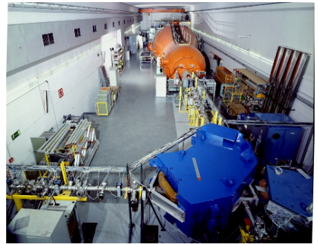
Figure 10.6: Photograph of the Tandem Accelerator tank (orange) and the first deflecting magnet (blue).
