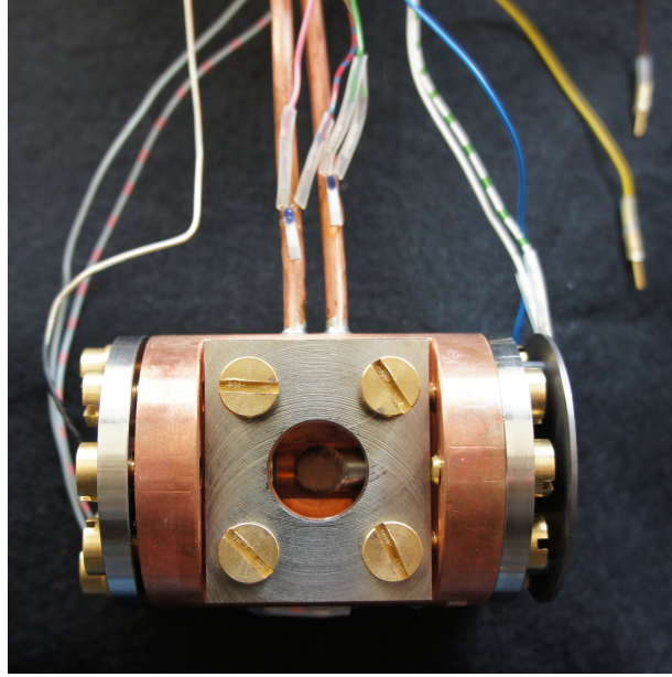
Figure 10.2: Photograph of the fully assembled target cell. In the middle the \text{MgF}_2 -exit window can be seen, which is held by a steel plate. Through the window the titanium entrance foil can be seen, which is glued to the beam entrance flange (from the right). On the very right, the tantalum aperture is visible. In the experiments the ion beam will come from the right, pass this aperture and enter the cell through the titanium foil. The tubes for gas inlet and outlet, respectively, are connected to the cell from the top. The various cables serve for read-out of the four PT-100 resistance thermometers and the electric charge of the endcap and the aperture. The two open cable heads in the top right corner are connected later-on to the heating resistor.
