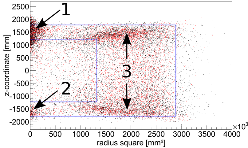
Figure 8.29: rz -distribution of the event vertices (black: delayed events, red: prompt events) of the accidental BiPo-214 coincidences found in the offtime-window analysis. The blue lines indicate the acrylic vessels of Target and GammaCatcher, respectively. Again, most of the events are located close to the chimney (1) because of the above-average high singles rate there. The event excess due to radioactivity from the pressure sensor (2) can be seen, too, in the middle of the GammaCatcher bottom. The two vertex clusters on top and bottom of the GammaCatcher volume (3) cannot be easily attributed to a source of radioactivity, but are likely caused by residual instrumental light.
