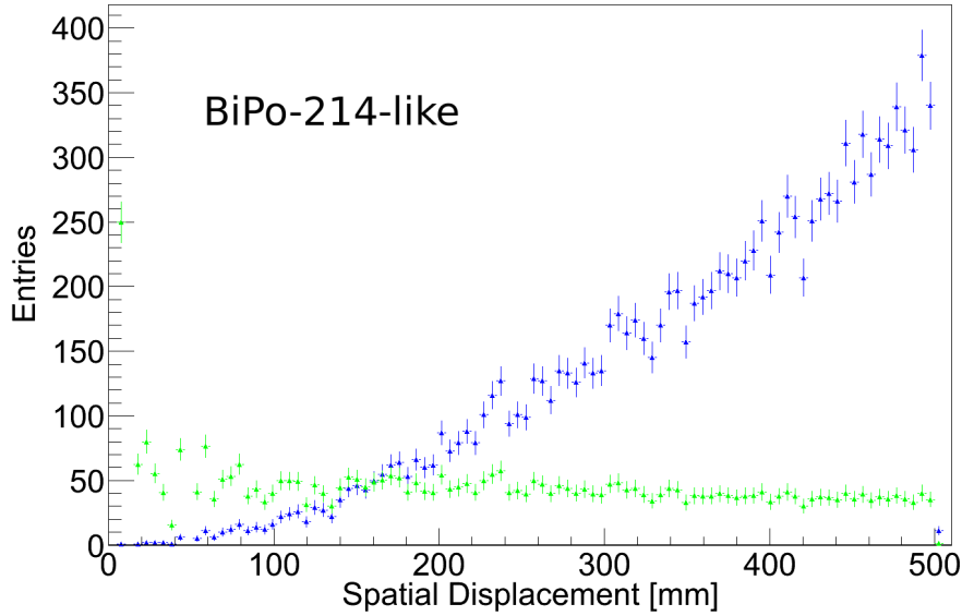
Figure 8.26: Spatial displacement between prompt and delayed event for the BiPo-214 candidates in the offtime-window search. The data (blue) rises like q^2 as is expected for a perfectly uncorrelated sample. The green data depicts the blue data corrected for volume effects, and is found to be flat. Error bars are statistical only.
