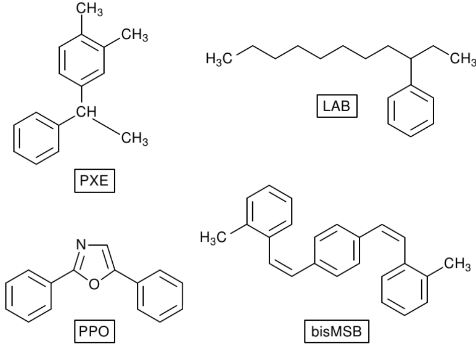
Figure 5.6: Chemical structures of the solvents Phenyl-o-Xylylethan (PXE) and linear Alkyl-Benzene (LAB), as well as of the fluors 2,5-Diphenyl-Oxazole (PPO) and 1,4-bis-(o-Methylstyryl)-Benzene (bisMSB) [Mar08]. The liquid scintillators of Target and GammaCatcher are based on PXE, while the InnerVeto liquid contains LAB as scintillating solvent. In all cases, the wavelength shifters PPO and bisMSB are added in small concentrations.
