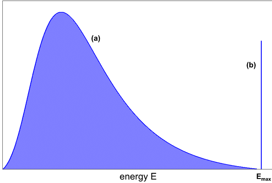
Figure 3.3: Schematic drawing of the summed electron energy spectra of the two neutrino (a) and the neutrinoless (b) double \beta -decay, respectively [Sch97]. E_{\max} denotes the Q -value of the decay. In the 2\nu\beta\beta decay part of the energy is carried away by the two neutrinos emitted, therefore, the energy spectrum of the electrons is continuous. In contrast, the electrons emitted in the 0\nu\beta\beta decay have in sum a well-defined energy, the Q -value of the decay, as the recoil energy of the daughter nucleus is negligible.
