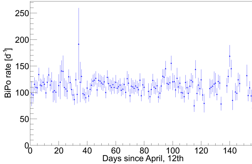
Figure 8.23: Daily rate of the BiPo-212 coincidences. The rate is stable over the time analysed, indicating no sources for thorium insertion into the detector. Error bars are statistical only.
