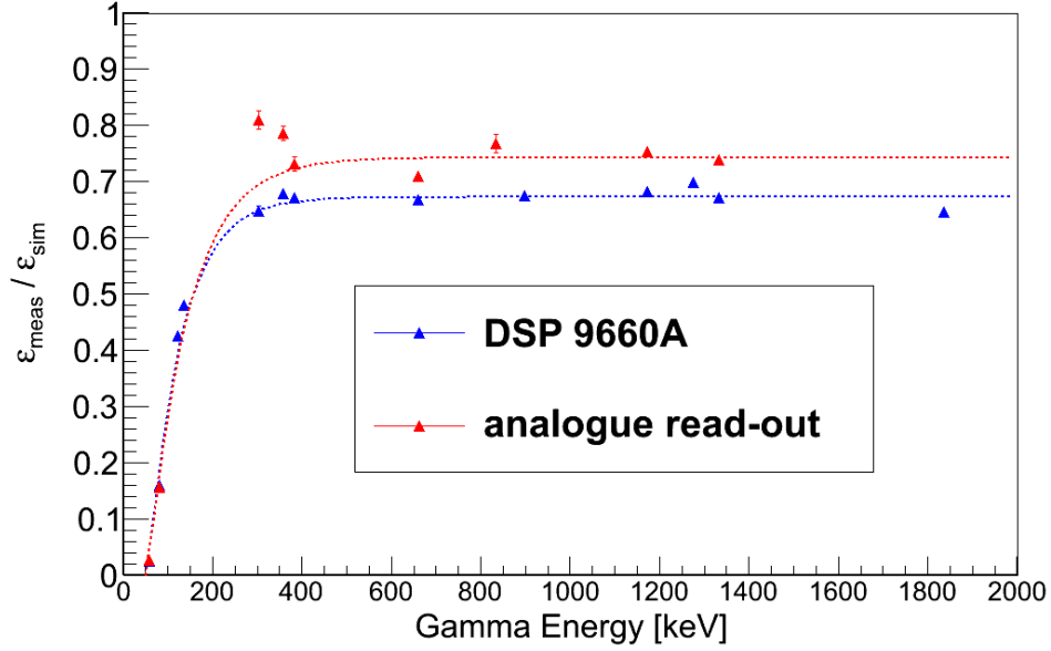
Figure 7.6: Ratio of measured \varepsilon_{meas} to simulated detector efficiencies \varepsilon_{sim} for the source position directly at the entrance window for the analogue read-out system (first calibration campaign; red data points) and the DSP 9660A (second calibration campaign; blue). The ratios obtained for the digital system in the first calibration are not shown here, as they match perfectly with the values of the second calibration. Both data are fitted with an exponential function plus a constant (see eq. (7.5); dashed lines). The error bars are calculated by linear error propagation from the errors quoted in tabs. D.3 through D.5. In most cases the error bars ( 1\sigma ) are smaller than the symbol used. For the gamma spectroscopy results presented in sec. 7.1.3 only the DSP 9660A was used.
