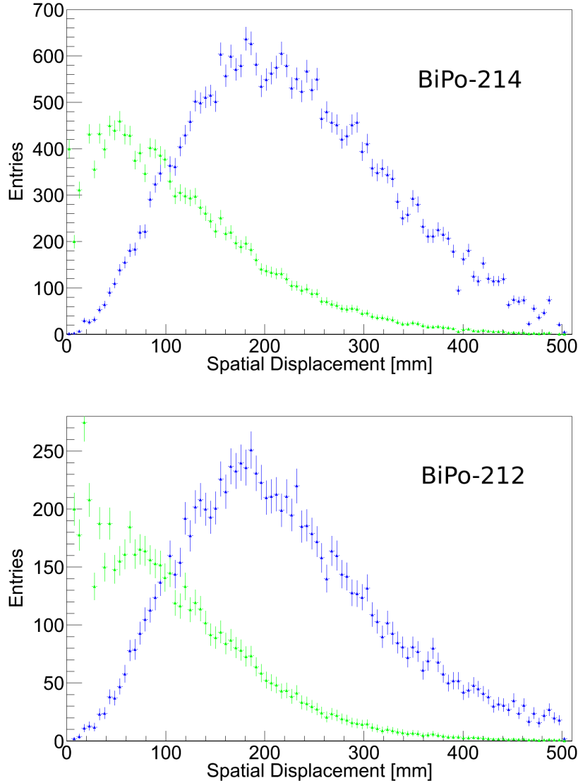
Figure 8.12: Spatial displacement \varrho between prompt and delayed event for the BiPo-214 coincidences (blue data points, top) and the BiPo-212 coincidences (blue data points, bottom). In both cases, the green data points show the displacements corrected for the volume effect (see text), and indicate clearly the spatial correlation of the two events. For the BiPo-214 coincidences the accidental background is once again subtracted statistically. Error bars are statistical only.
