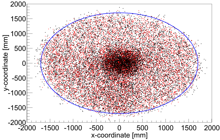
Figure 8.15: xy-projection of the reconstructed event vertices of the BiPo-214 coincidences for events above the Target vessel top lid. The vertices of the prompt events are depicted in red, the vertices of the delayed events in black. The blue ellipse indicates the position of the GammaCatcher acrylic vessel. The excess of BiPo-214 events in the middle is still seen, depicting events close to the chimney which might be due to the higher rate of external gamma rays there.
