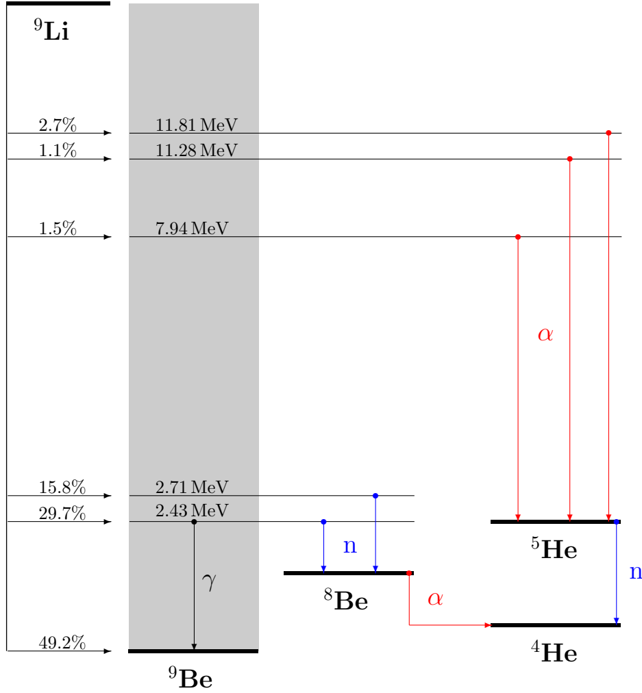
Figure 6.3: Simplified decay scheme of the \beta - n emitting isotope ^9\text{Li} . In nearly 50% of all cases ^9\text{Li} decays directly into the stable ground state of ^9\text{Be} by means of a \beta^- -decay, all other branchings lead to a highly excited state of ^9\text{Be} (greyish shaded box) with energies above the neutron separation threshold; the excitation energies are indicated, too. The states at 2.71 MeV and 2.43 MeV decay by neutron emission into ^8\text{Be} , which subsequently splits up into two alpha particles. Of all the excited states of ^9\text{Be} only that at 2.43 MeV has a non-vanishing probability to de-excite by gamma emission before neutron separation. The higher excited states of ^9\text{Be} are unstable to \alpha -decay, which leads to ^5\text{He} . This isotope also emits a neutron; therefore, all decay modes, except for the direct decay into the ground state (and the gamma transition from the 2.43 MeV level), have the net reaction ^9\text{Li} \rightarrow e^- + \bar{\nu}_e + n + 2\alpha . Data taken from [Fir96, TUN04].
