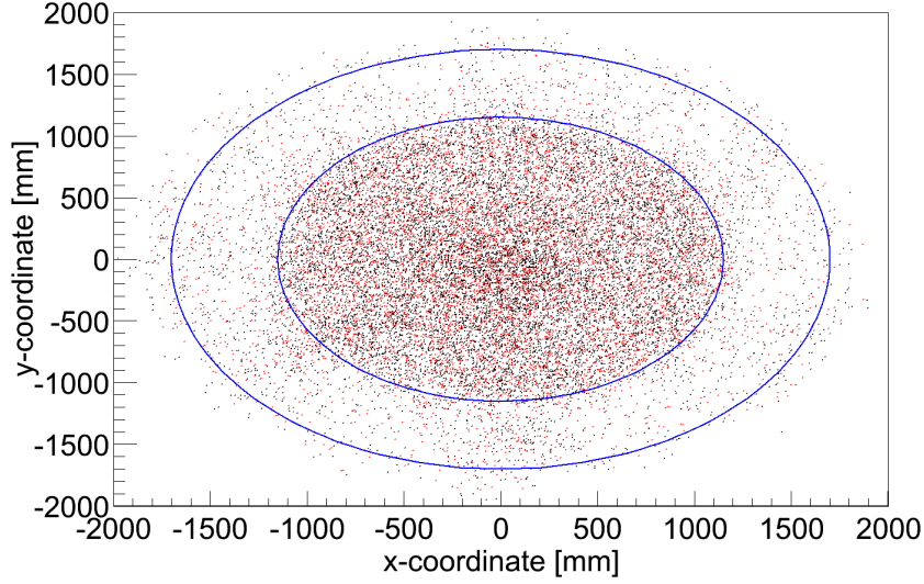
Figure 8.18: xy -projection of the reconstructed event vertices of the BiPo-212 coincidences. The vertices of the prompt events are depicted in red, the vertices of the delayed events in black. The blue ellipses indicate the positions of the Target and GammaCatcher acrylic vessels, respectively. Unlike the BiPo-214 coincidences most of the events are located in the Target region; only little events are found in the GammaCatcher. The homogeneous vertex distribution indicates that the impurities are contained within the liquid itself.
