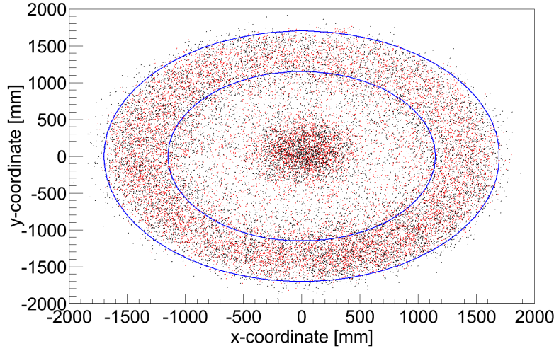
Figure 8.28: xy -projection of the event vertices (black: delayed events, red: prompt events) of the accidental BiPo-214 coincidences found in the offtime-window analysis. The blue ellipses indicate the positions of Target and GammaCatcher acrylic vessel. Most of the vertices are located in the middle close to the chimney. There, no shielding against external radiation is present, which causes the singles rate and with it the BiPo-like coincidences to increase. Like for the true BiPo-214 coincidences more events are found in the GammaCatcher than in the Target, indicating a slightly higher rate of radioactivity-induced events there.
