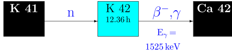
Figure 7.11: Neutron activation and decay scheme of ^{41}\text{K} . Stable ^{41}\text{K} is activated by thermal neutron capture. The subsequent \beta^- -decay of ^{42}\text{K} with a half-life of 12.36 h into stable ^{42}\text{Ca} also releases (with an emission probability of 18.1%) 1525 keV-gamma quanta, which are measurable with the germanium detector. Data taken from [Fir96].
