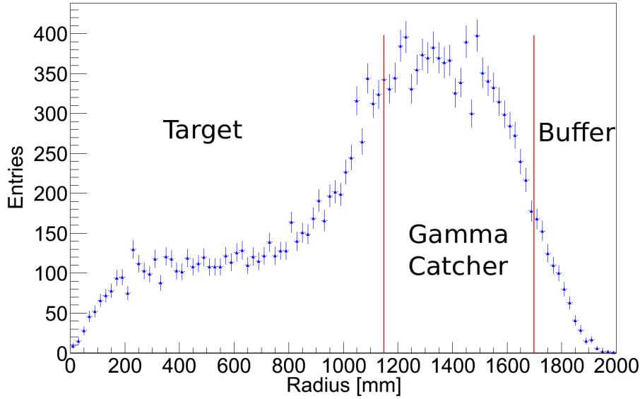
Figure 8.17: Radial distribution of the BiPo-214 coincidences with a z -component of the event vertex greater than -1229\text{ mm} and smaller than 1229\text{ mm} (height of the Target vessel), not corrected for any volume effects. The positions of Target vessel wall and GammaCatcher vessel wall, respectively, are indicated by the two red lines. The Target liquid contains much less BiPo-214 events than the GammaCatcher. The rise in the event number close to the Target vessel and within the Buffer volume is due to the spatial resolution of the vertex reconstruction. No aggregation of events at the vessel walls is seen, i.e. a radon emanation by the acrylic itself is unlikely. Error bars are statistical only.
