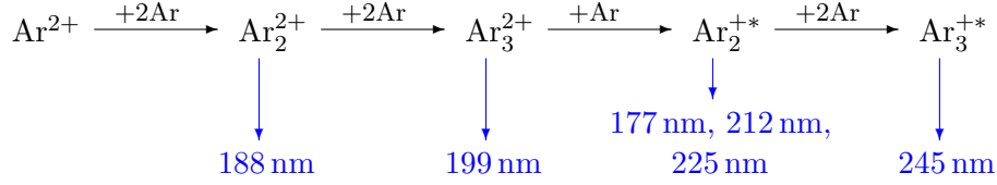
Figure 9.3: Possible interpretation of the initial steps of the gas kinetic processes following the formation of an \text{Ar}^{2+} -ion [Wie00]; the newly formed excimer molecules can either decay radiatively (the photon wavelengths are given in blue) or lose energy in collision processes with other argon atoms, forming molecules with lower energy. For details see text.
