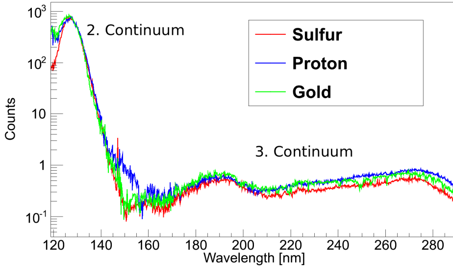
Figure 11.16: Scintillation spectrum (covering 118 nm through 290 nm in wavelength) of gaseous argon at \sim 99 K and 1200 mbar pressure excited by three different particle beams: protons, S^{10+} , and Au^{14+} . The width of the monochromator's entrance slit was set to 100\ \mu\text{m} ( 500\ \mu\text{m} for protons), which translates into an optical resolution of 0.3\ \text{nm} ( 1.5\ \text{nm} ). The spectra are corrected for the detector response function and the "fogging" effect. The deviation in the spectrum recorded with protons between 145\ \text{nm} and 160\ \text{nm} is most likely caused by an instability of the beam current. Besides this the three spectra are similar. For the excitation by the sulfur beam a tiny emission from a xenon impurity can be seen at 146.96\ \text{nm} [NIS12].
