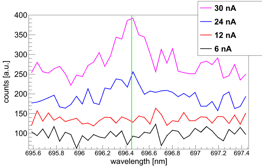
Figure 11.2: The 4p-4s emission line of argon at 696.45 nm (position indicated by the green line) for different values of the beam current: black 6 nA, red 12 nA, blue 24 nA, and pink 30 nA. The different spectra are shifted along the y-axis to make the differences better visible. The 4p-4s line is invisible for beam currents of 6 nA and 12 nA, respectively, while it is indicated for a current of 24 nA and clearly visible for 30 nA. Hence, for this set of beam parameters the evaporation of the liquid argon starts at a beam current around 20 nA, and the beam current has to be kept at lower values for spectroscopy of liquid argon.
