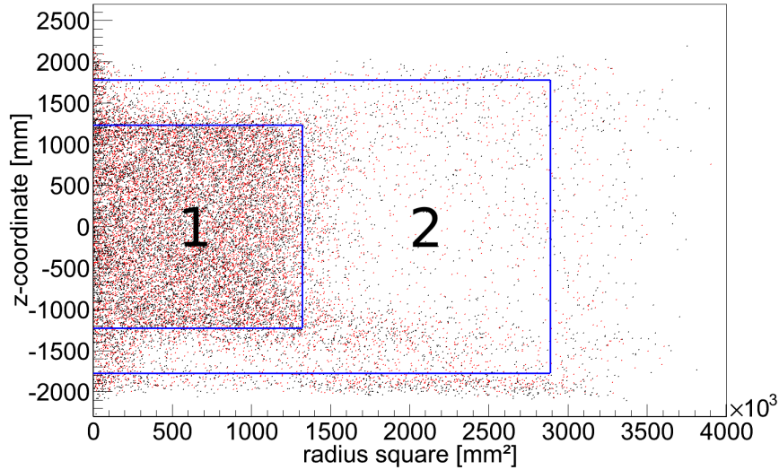
Figure 8.19: rz -projection of the reconstructed event vertices of the BiPo-212 coincidences. The vertices of the prompt events are depicted in red, the vertices of the delayed events in black. The abscissa is scaled quadratically to correct the vertex density for volume effects. The blue lines indicate the positions of the Target and GammaCatcher acrylic vessels, respectively. Again, the higher concentration of thorium in the Target (1) than in the GammaCatcher (2) can be seen.
