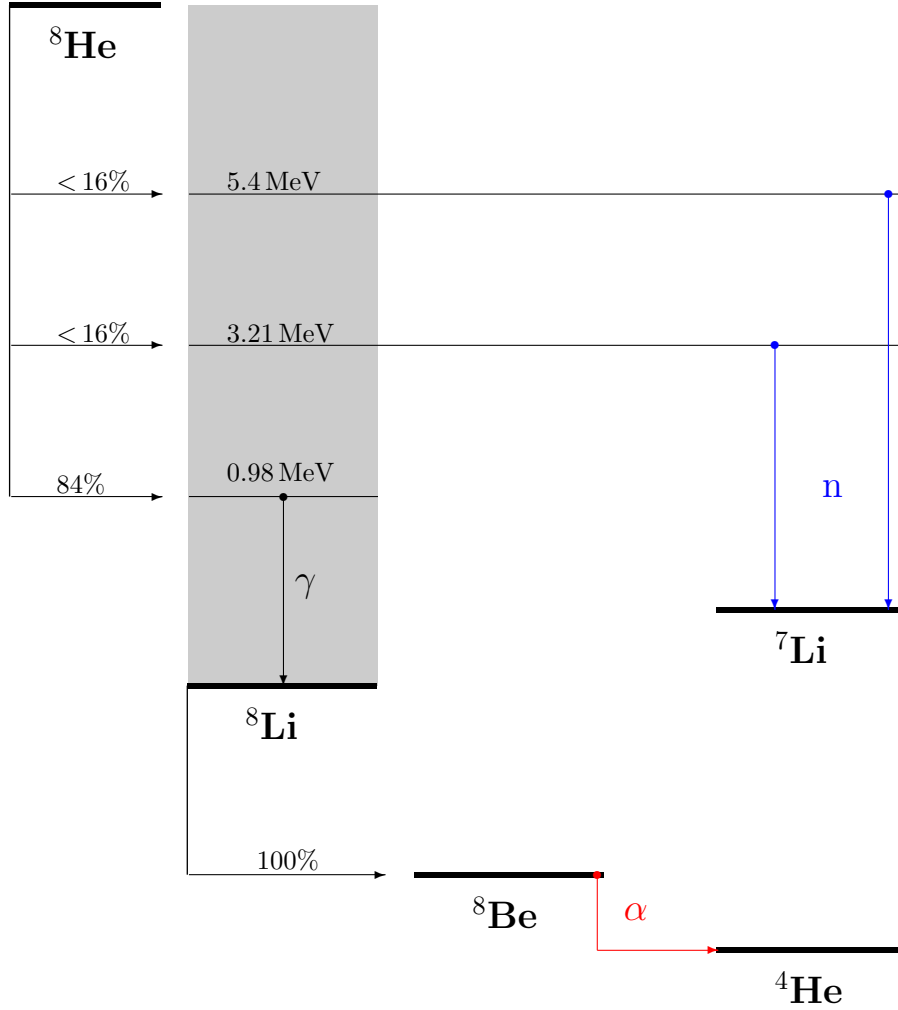
Figure 6.4: Simplified decay scheme of the \beta -n emitting isotope ^8\text{He} . In 84% of all cases ^8\text{He} decays into a low excited state (0.98 MeV) of ^8\text{Li} , which de-excites by gamma emission. ^8\text{Li} is itself unstable to \beta^- -decay, with ^8\text{Be} being the daughter nucleus, which eventually splits up into two \alpha -particles. Thus, in total this branch of the decay has the reaction equation ^8\text{He} \rightarrow 2\alpha + 2e^- + 2\bar{\nu}_e + \gamma . In less than 16% of all cases the \beta^- -decay of ^8\text{He} leads to a highly excited state of ^8\text{Li} , which decays by neutron emission into the stable isotope ^7\text{Li} . The greyish shaded box indicates the excitation levels of ^8\text{Li} ; the excitation energies are given, too. Note that not all levels are shown, therefore, the decay probabilities do not add up to 100%. Data taken from [Fir96, TUN04].
