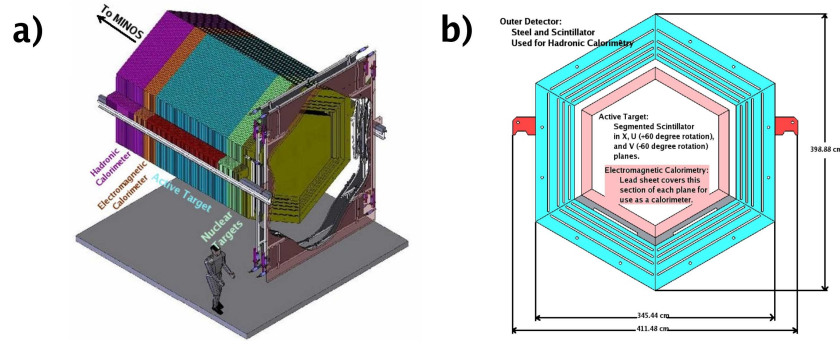
Fig. 6. (a) A schematic drawing of the MINERνA detector. The detector is segmented into various parts as labeled in the figure. The detector is approximately 4 m wide by 4 m long. (b) A schematic of a single plane within the MINERνA detector.
