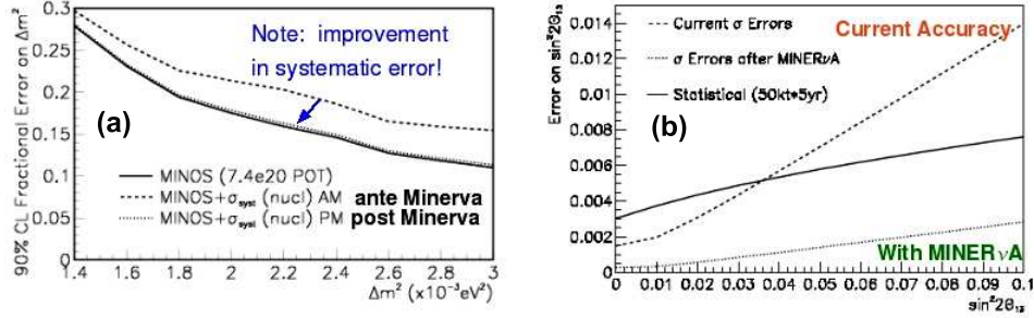
Fig. 4. Effect of increased precision in total cross-section data on the systematic error for neutrino-oscillation measurements for \Delta m^2 (a) and \sin^2(\theta_{13}) (b).
