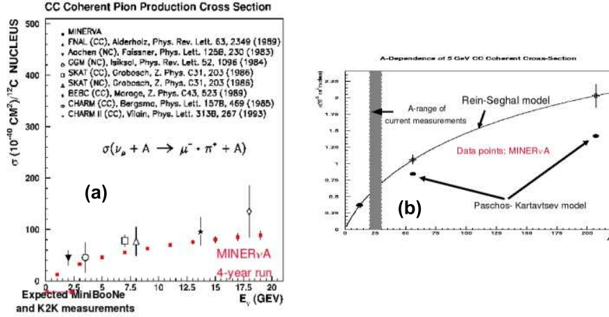
Fig. 3. Estimated improvement in precision for coherent single pion production in neutrino scattering. Notice that the MINER \nu A data will significantly increase the energy range of available data (a) and the A-region and production models [5, 6] explored (b).
