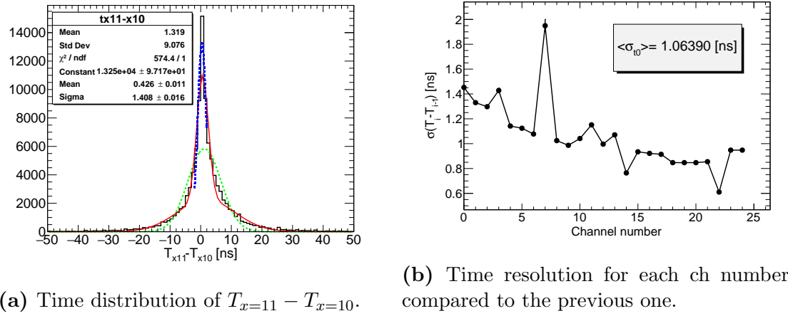
Figure 4.37: Intrinsic time resolution measurements. The left plot shows the time distribution of the difference between two contiguous channels. Two Gaussian fit are adjusted, a narrow and a wider one. The parameters in the plot represent the sigma for the convolution of the two Gaussian functions (in red). The plot on the right, is the collection of each \sigma_i for each comparison of two adjacent channels.
