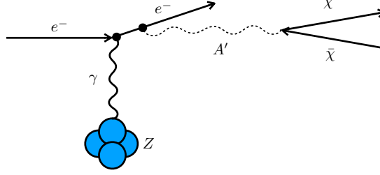
Figure 4.5: Diagram illustrating the massive A' production in the reaction e + Z \rightarrow eZA' of electrons scattering off a nuclei with the subsequent A' into dark matter particles.
