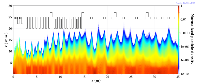
Figure 3: Accumulated beam density for 10^4 linacs with errors in the r plane.
