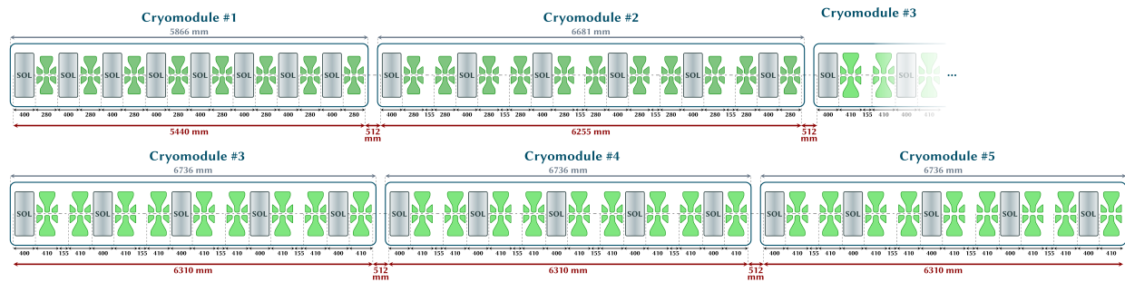
Figure 1: IFMIF-DONES SRF-linac general layout.
