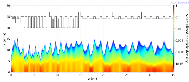
Figure 2: Beam density in r plane along the DONES SRF-linac.
