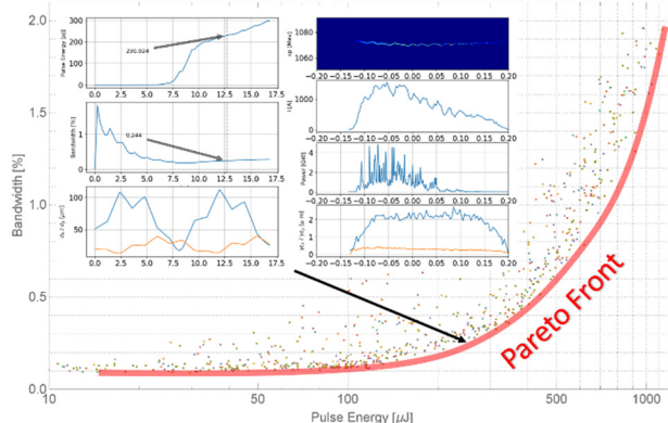
Figure 7: Pareto front in Pulse energy – Bandwidth space for a S2E model of XARA, using Genesis in SASE mode. A 230μJ representative point on the Pareto front is shown.
