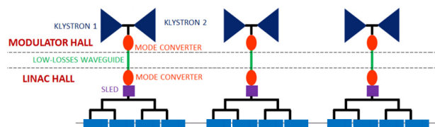
Figure 3: Schematic of the proposed X-band linac section, adapted from [24].
